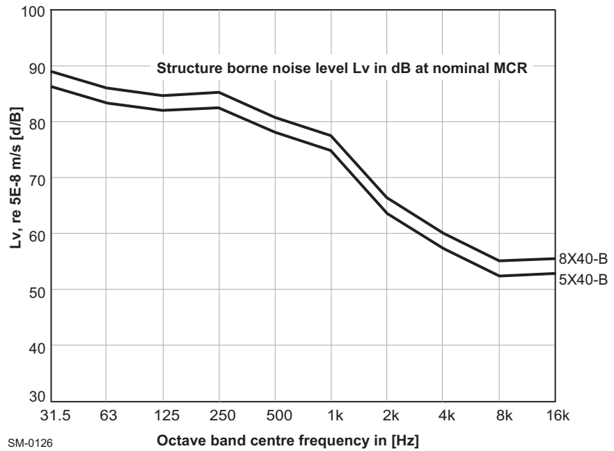
Figure 7-13 Structure-borne noise level at engine feet vertical
