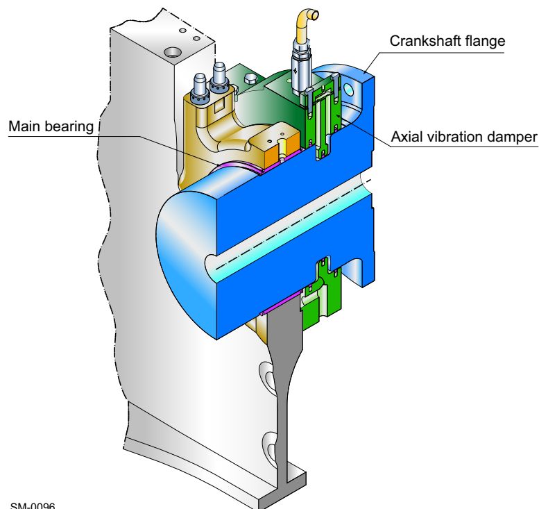
Figure 6-15 Example of axial vibration damper
