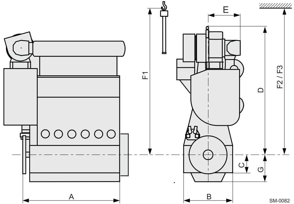
Figure 3-1 Engine dimensions
