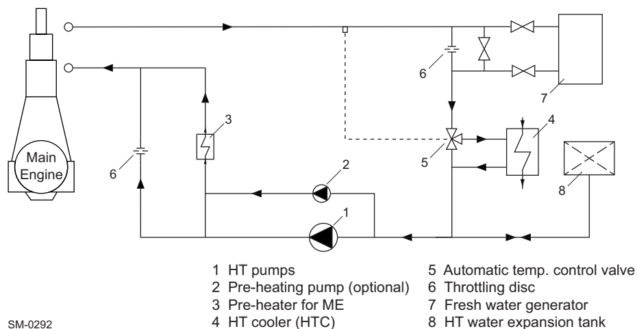
Figure 4-7 HT cooling water circuit
