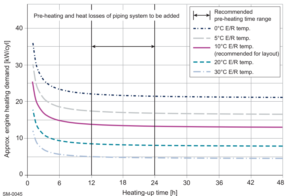
Figure 4-8 Pre-heating power requirement per cylinder
