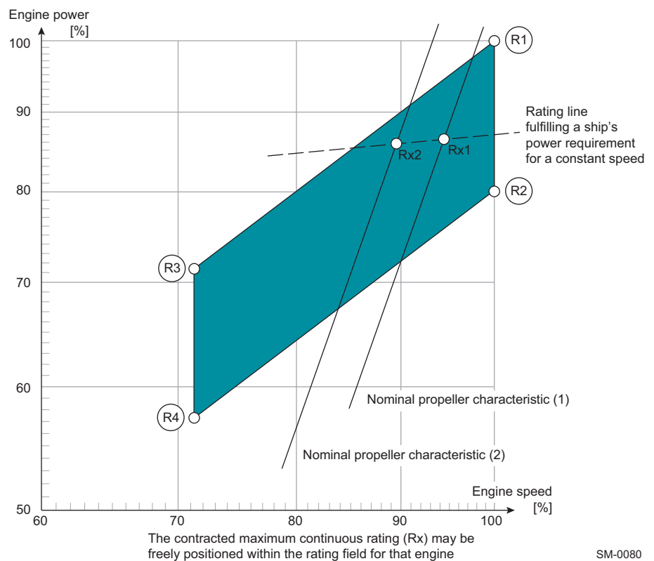
Figure 2-1 Rating field for the X40-B
