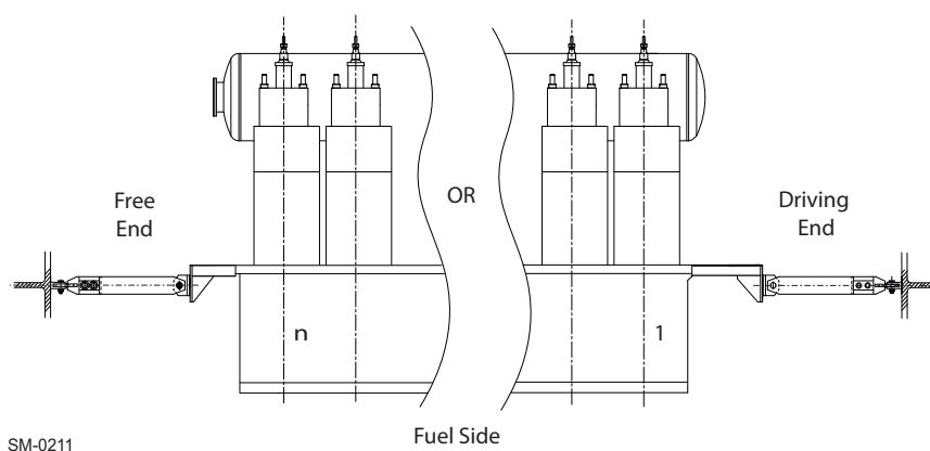
Figure 6-13 Arrangement of longitudinal stays
