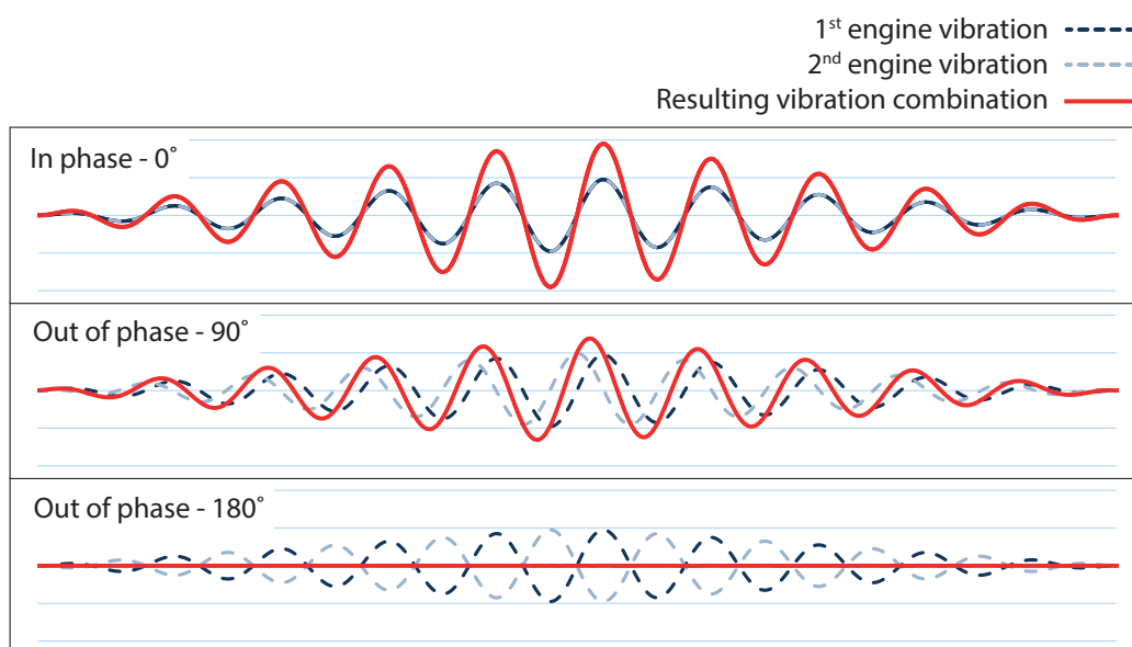
Figure 6-16 Resulting vibration from SPS combinations
