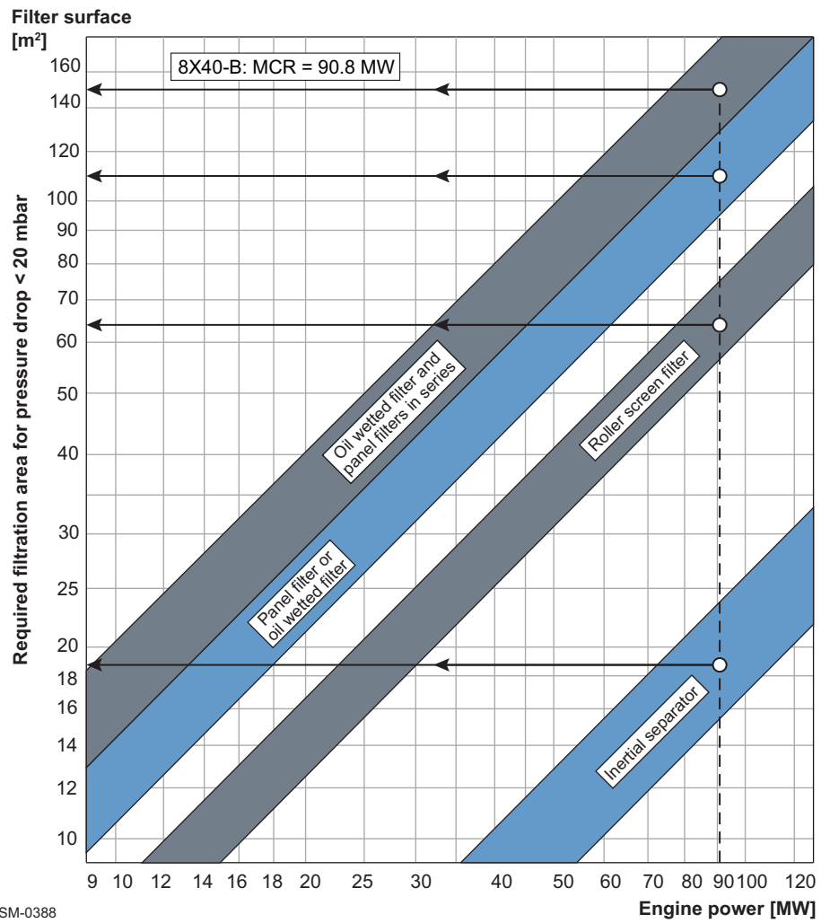
Figure 4-27 Air filter size (example for 8-cyl. engine)
