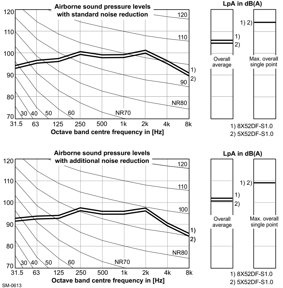
Figure 7-3 Sound pressure level at 1 m distance from engine
