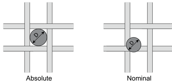
Figure 4-41 Mesh size difference between absolute and nominal
