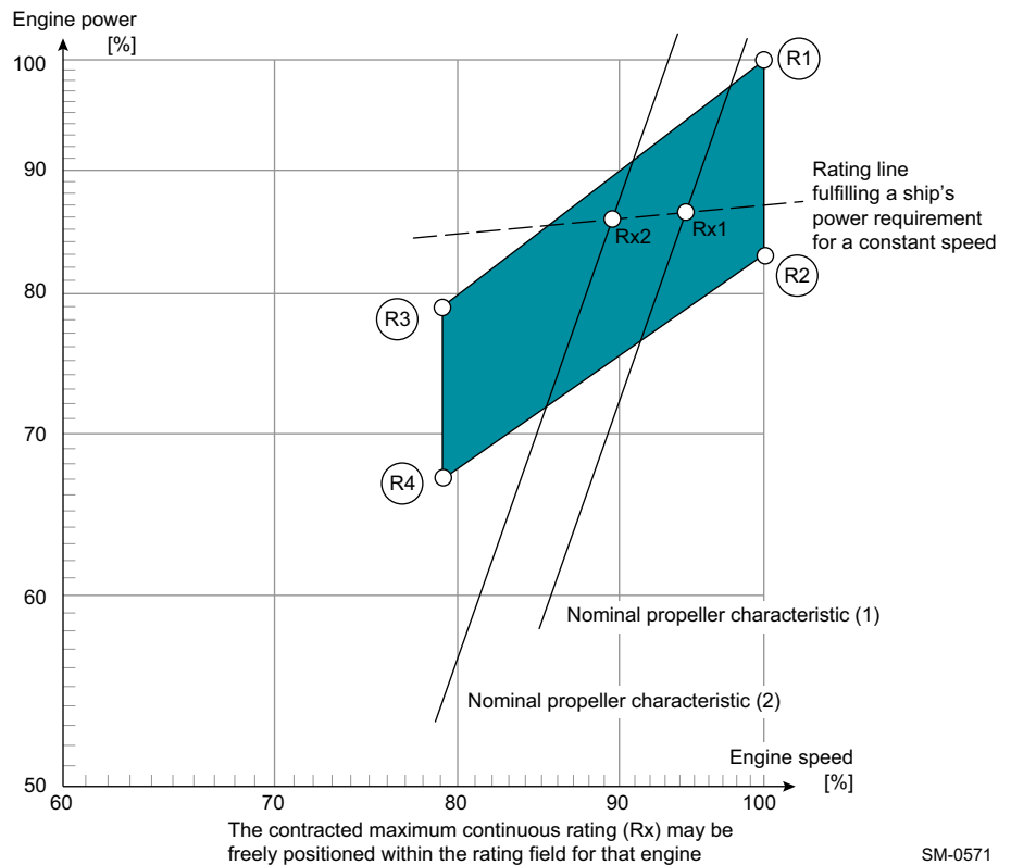
Figure 2-1 Rating field for the X52DF-S1.0
