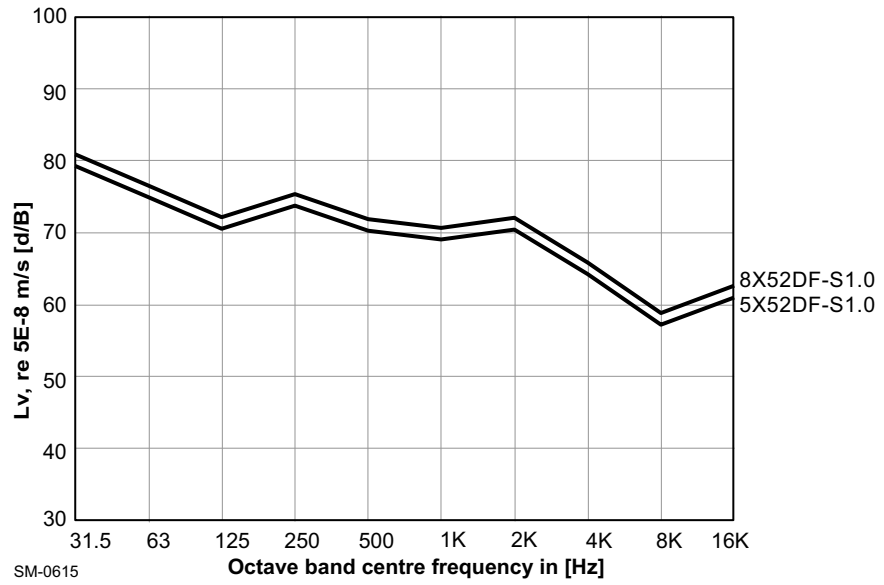
Figure 7-6 Structure-borne noise level at engine feet vertical
