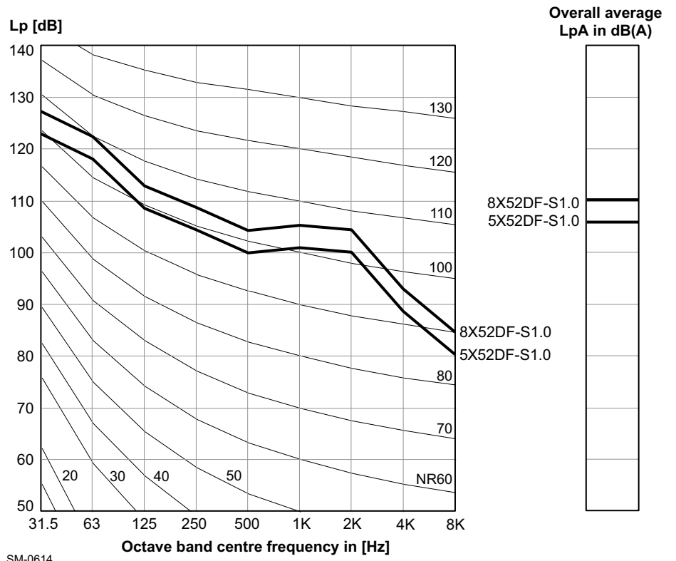
Figure 7-5 Sound pressure level at funnel top of exhaust gas system
