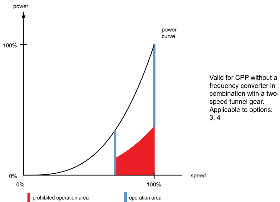
Figure 4-82 CPP with two fixed operation speeds without frequency converter
