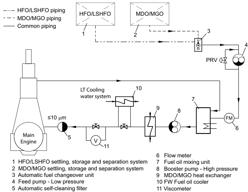
Figure 4-65 Fuel oil filter arrangement ‘B’
