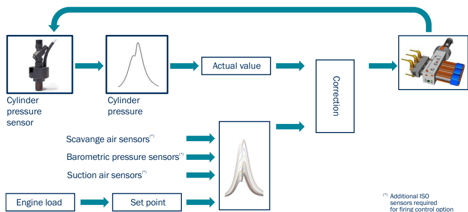
Figure 5-10 The ICC system
