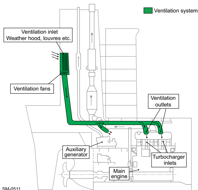
Figure 4-75 Ventilation system arrangement 1: Engine room ventilation system
