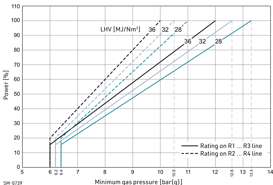
SM-0739 Figure 4-49 Design fuel gas supply pressure requirements
