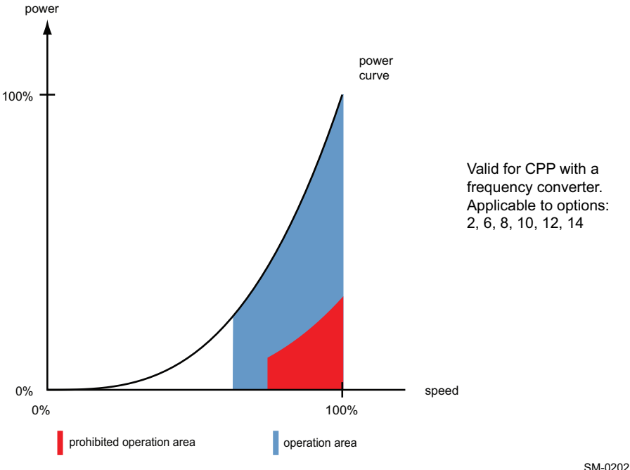
Figure 4-80 CPP in combination with an optional frequency converter
