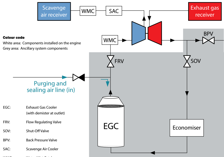
Figure 4-16 The iCER exhaust gas system with one turbocharger and the exhaust gas return pipe routed to the turbocharger connection from above
