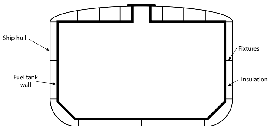
Figure 4-40 Section view of an integrated membrane tank
