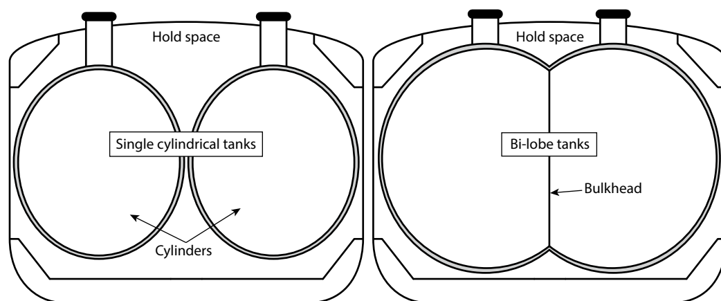
Figure 4-43 Section view of different free-standing Type C tanks installed below the deck
