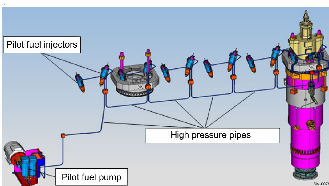
Figure 4-60 Pilot fuel high-pressure system
