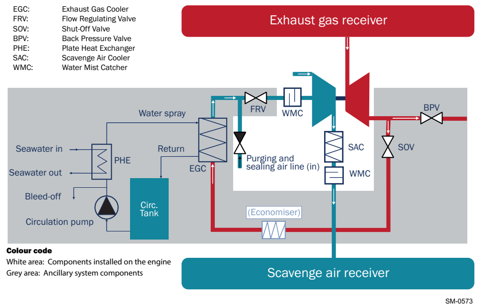
Figure 4-5 The iCER system with one turbocharger and the exhaust gas return pipe routed to the turbocharger connection from above
