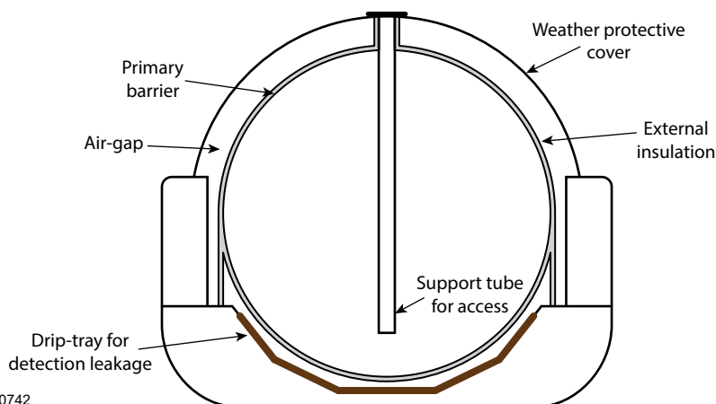
Figure 4-42 Section view of a free-standing Type B tank of moss design
