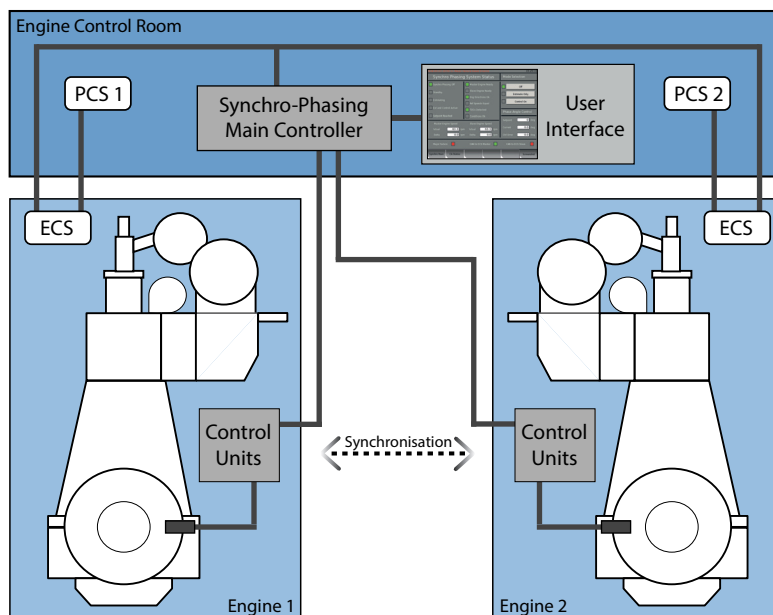
Figure 6-18 Synchro-Phasing system
