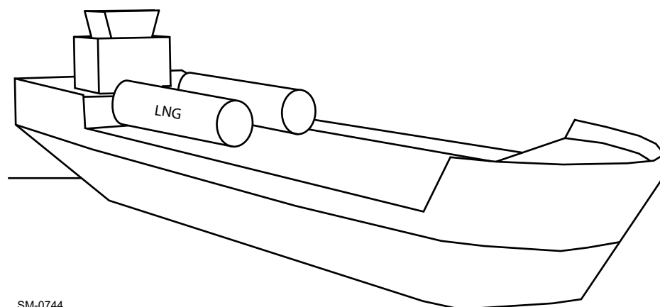
Figure 4-44 Type C tank on the deck of a vessel
