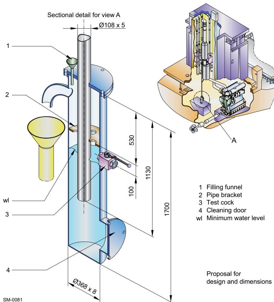
Figure 4-72 Arrangement of automatic water drain
