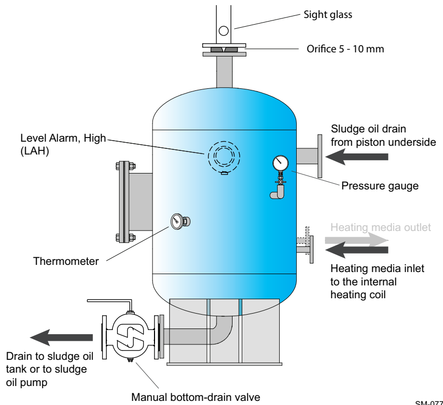
Figure 4-70 Design proposal of a manually bottom-drained sludge oil trap
