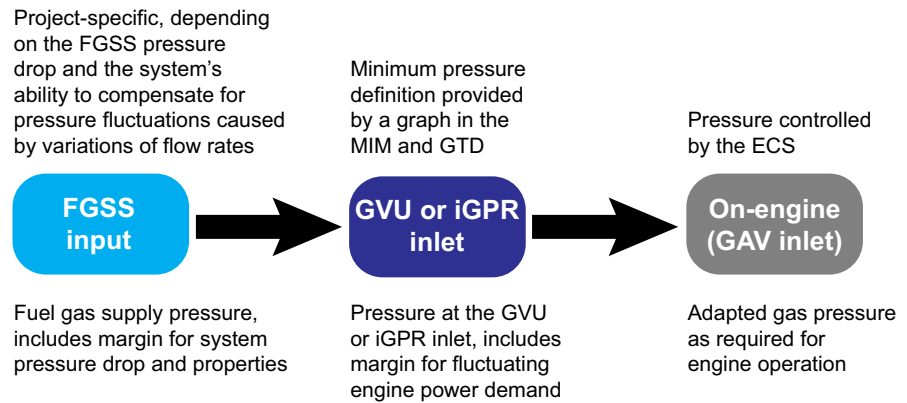
SM-0773 Figure 4-52 Fuel gas pressure level definitions
