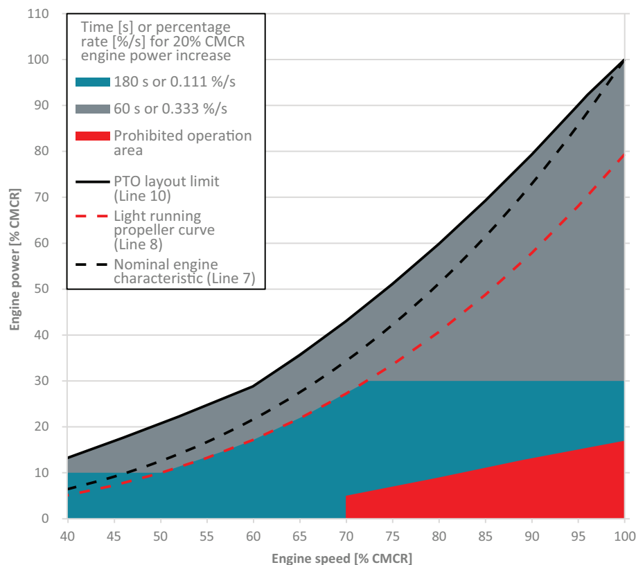
Figure 4-83 Maximum power increase rate for PTO application in gas mode
