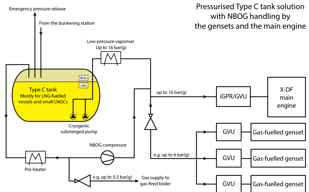
Figure 4-46 Pressurised Type C tank solution with NBOG handling by the gensets and the main engine
