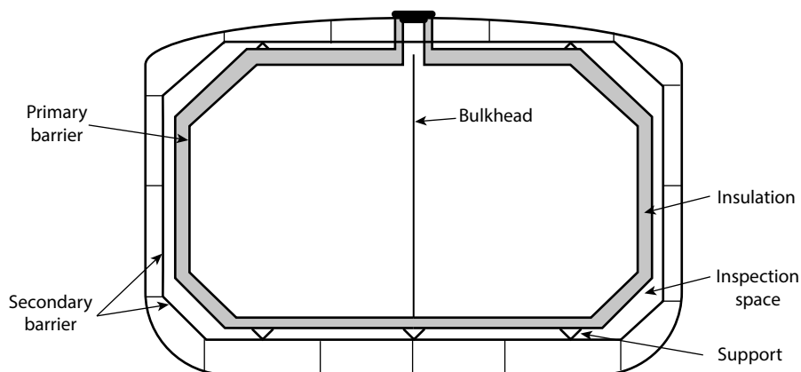
Figure 4-41 Section view of a free-standing Type A tank
