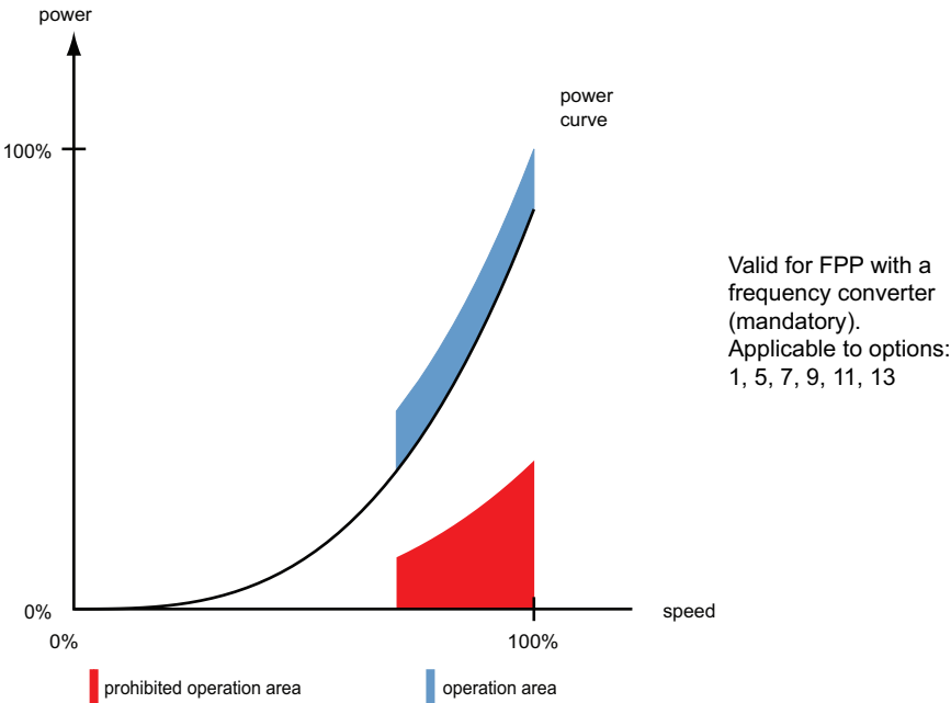
Figure 4-79 FPP with mandatory frequency converter
