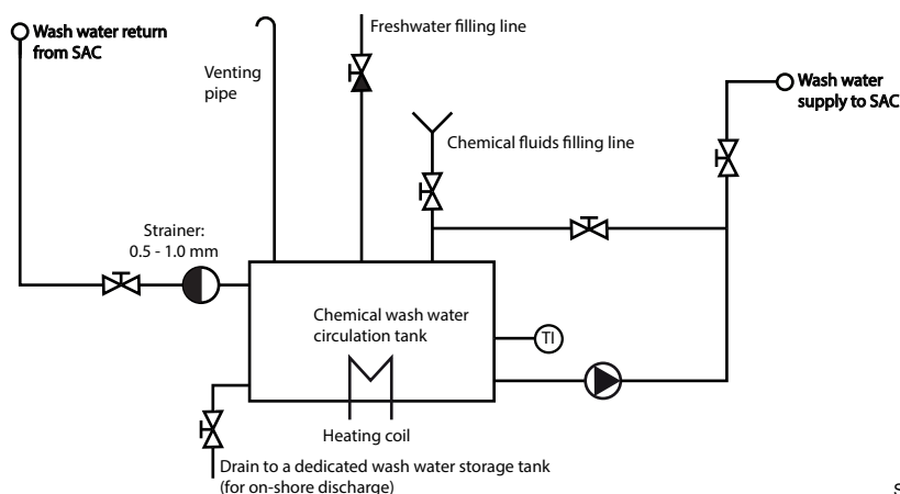
Figure 4-73 Offline SAC washing system (external system)
