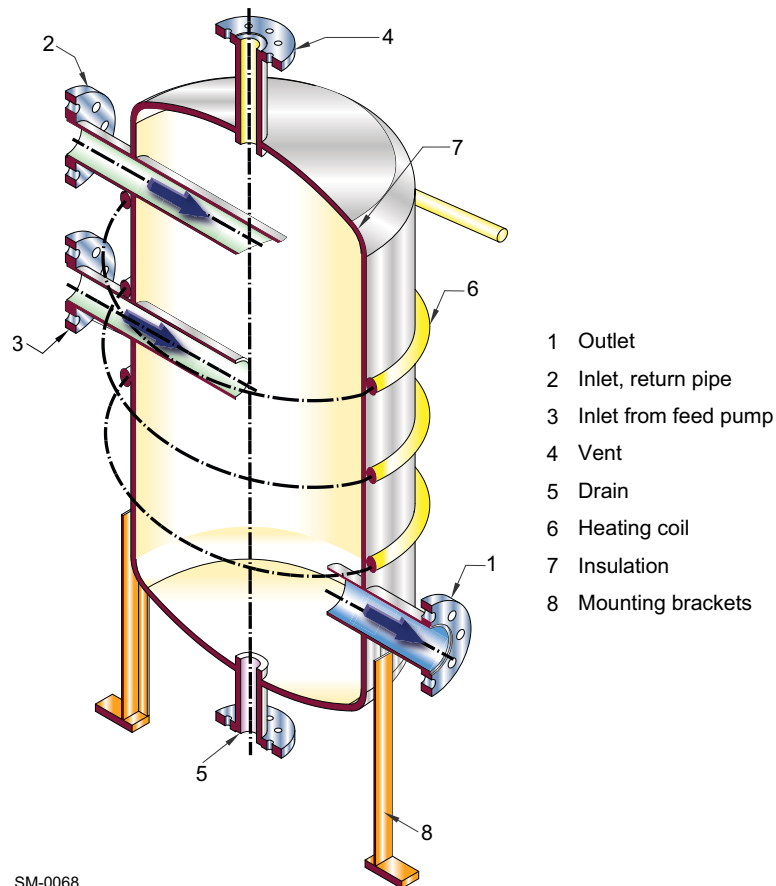
Figure 4-62 Mixing unit
