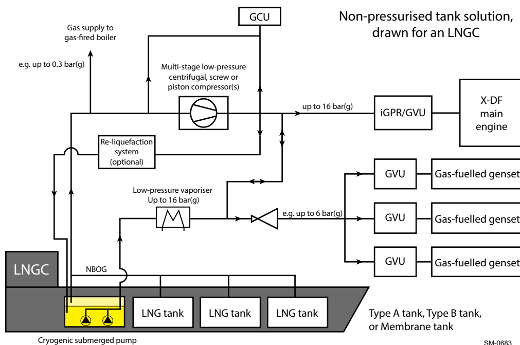
Figure 4-47 Non-pressurised tank solution, drawn for an LNGC
