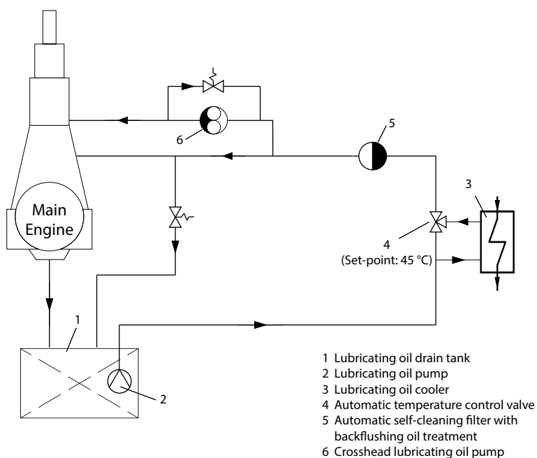
Figure 4-31 LO system
