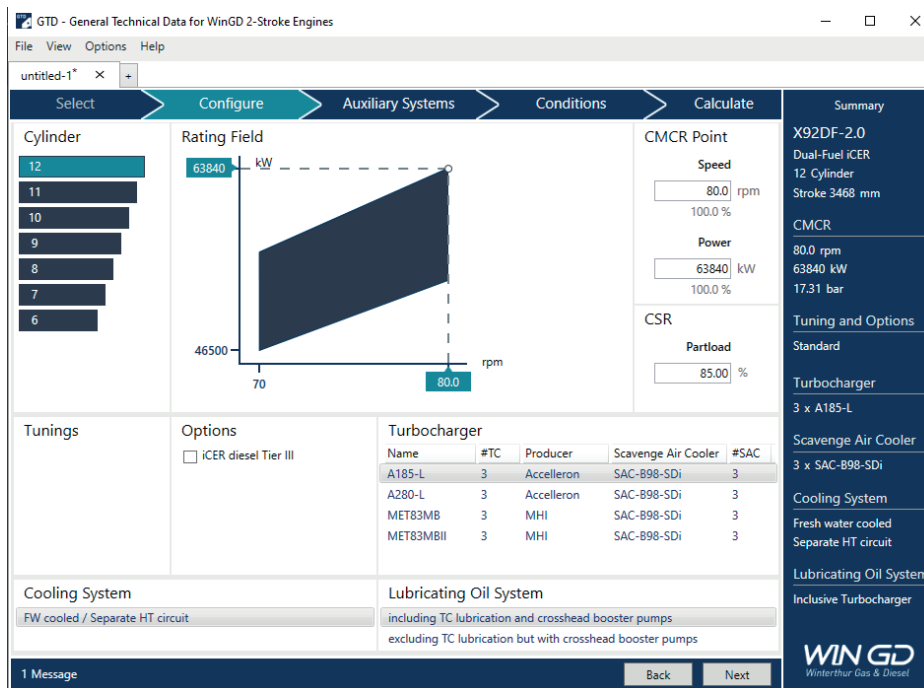
Figure 0-1 GTD screenshot
