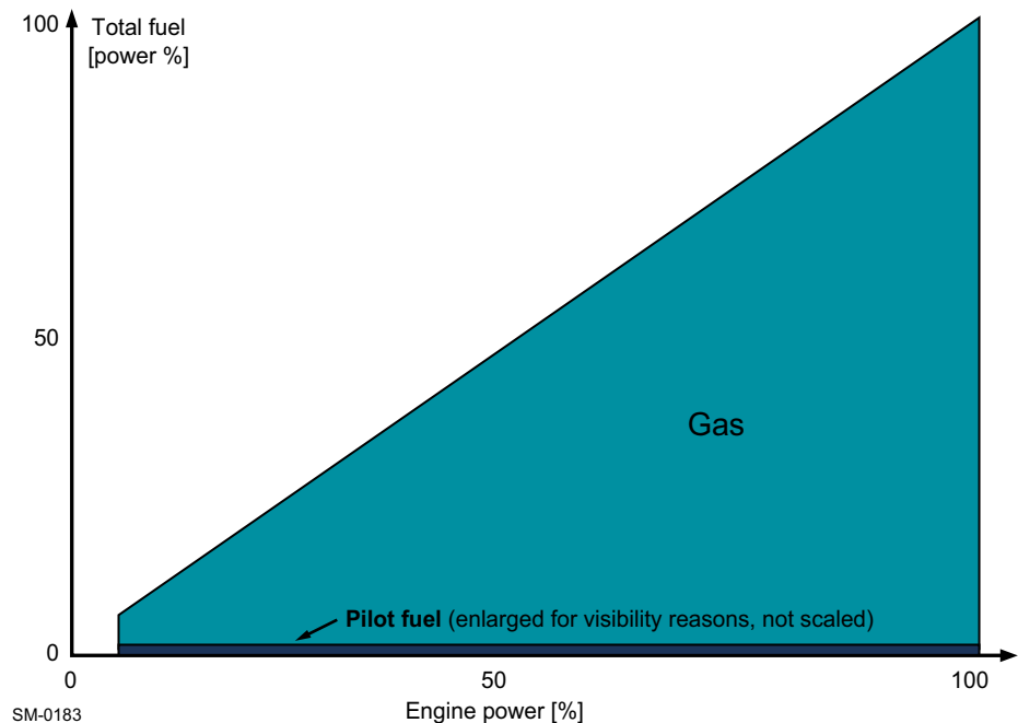
Figure 1-3 Gas mode
