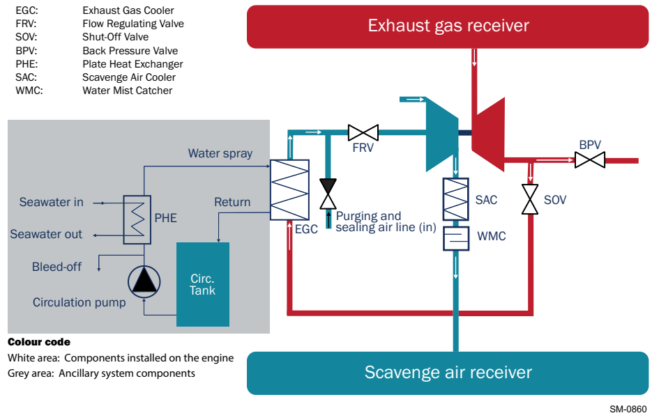
Figure 1-6 The iCER on-engine system
