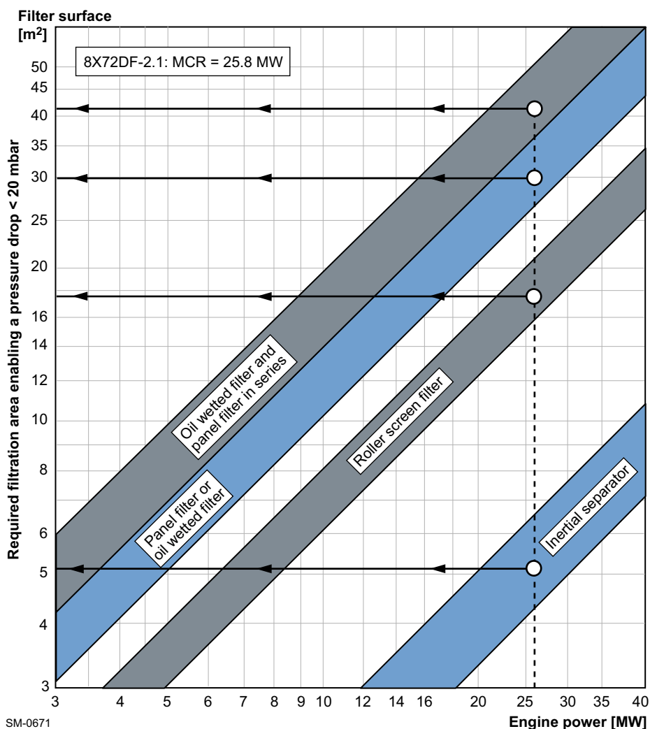
Figure 4-77 Air filter size (example for the 8-cylinder engine)
