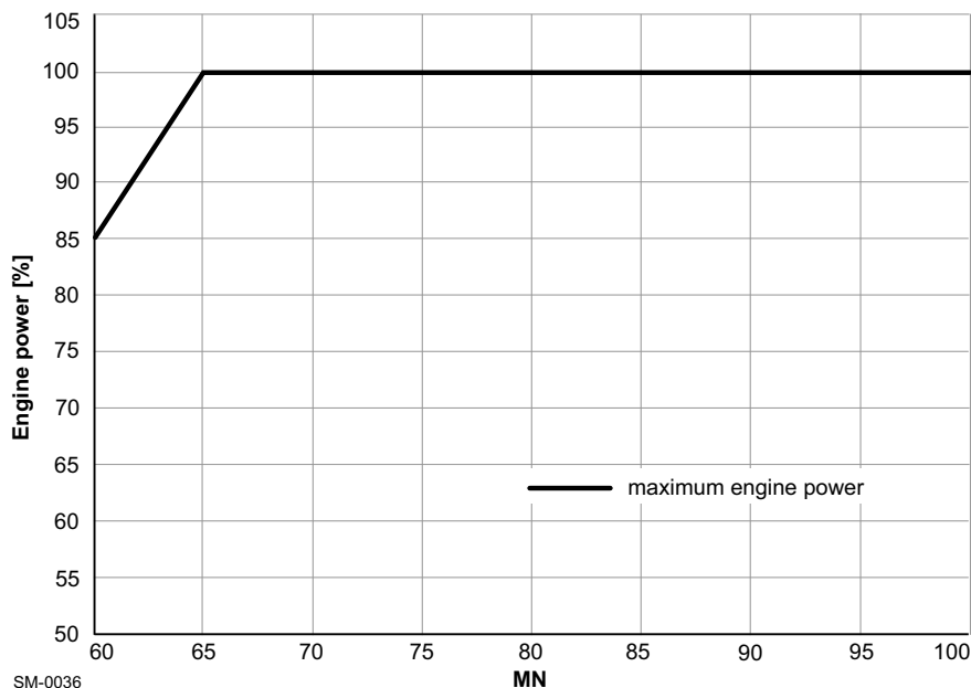
Figure 4-39 Maximum achievable power
