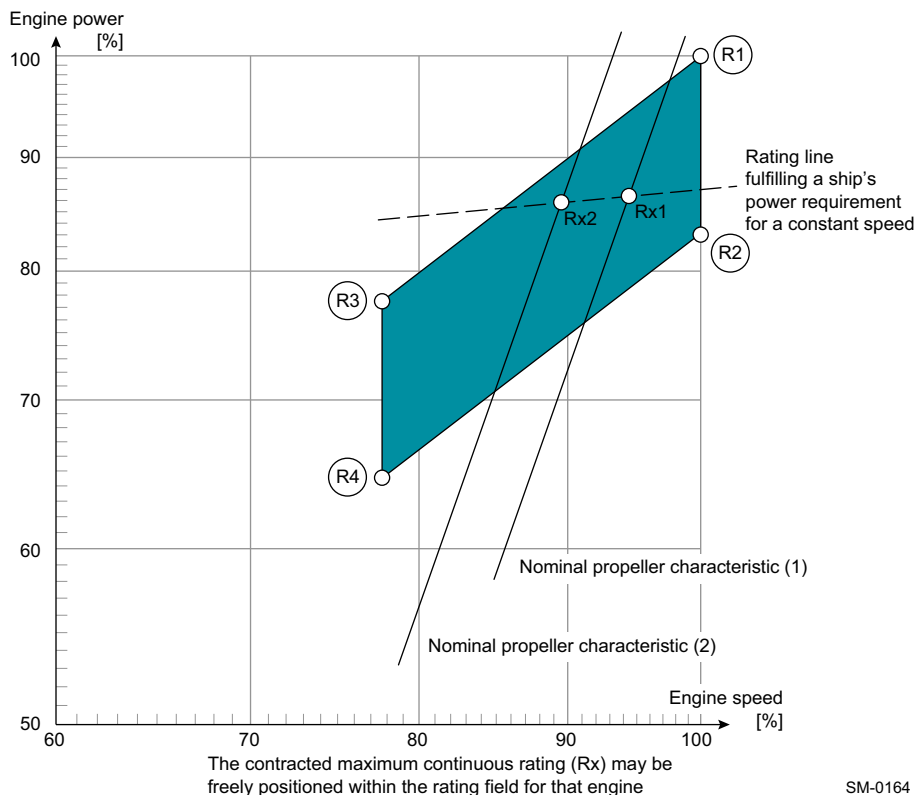
Figure 2-1 Rating field for the X62DF-2.1
