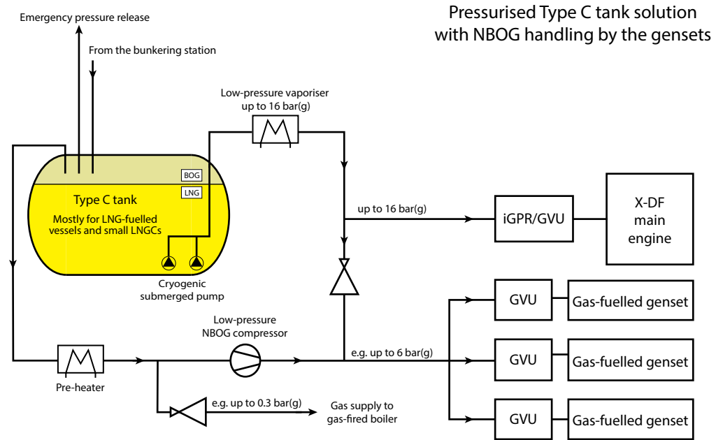
Figure 4-45 Pressurised Type C tank solution with NBOG handling by the gensets
