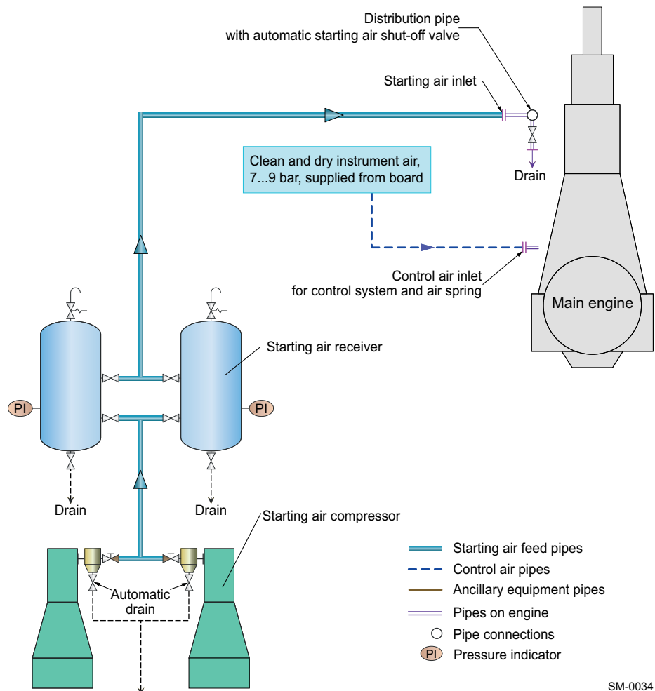
Figure 4-68 Air supply system
