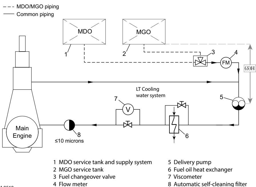
Figure 4-66 Fuel oil system — Arrangement with only MDO/MGO or MGO
