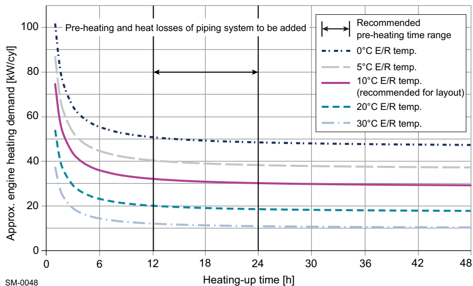
Figure 4-30 Pre-heating power requirement per cylinder
