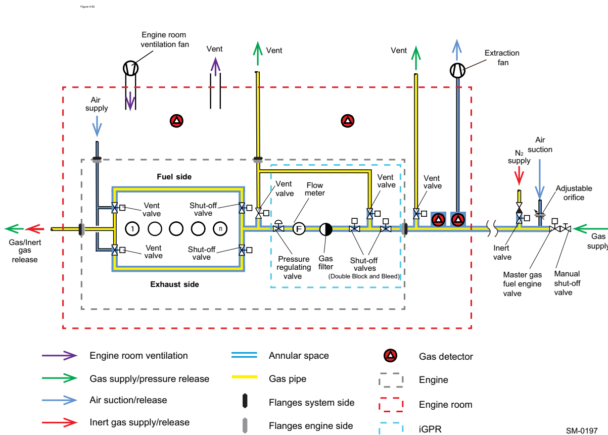
Figure 4-54 FGSS with the iGPR
