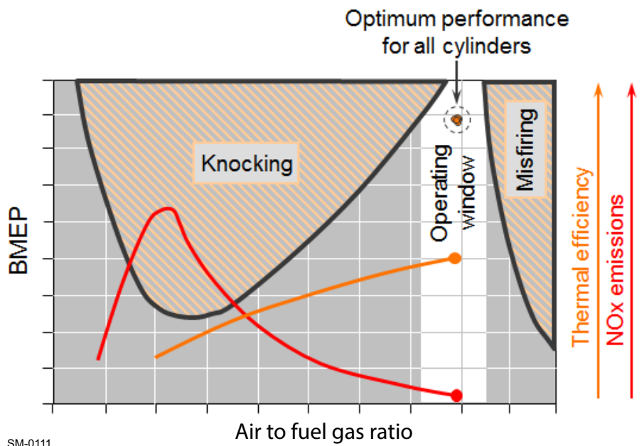
Figure 4-38 Lean-burn operation window
