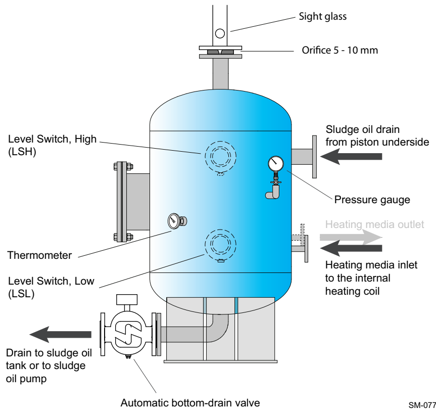
Figure 4-71 Design proposal of an automatically bottom-drained sludge oil trap
