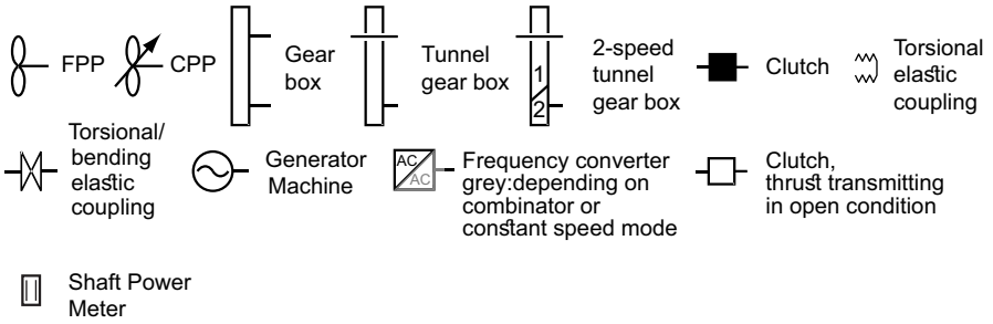
SM-0200 Figure 4-78 Arrangements for PTO, PTI, PTH
