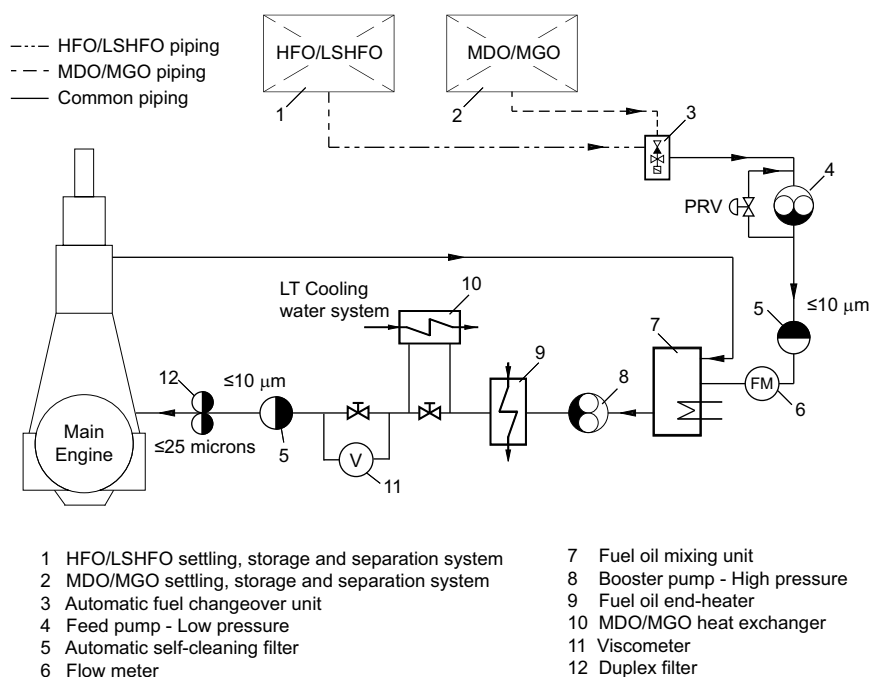
Figure 4-61 Fuel oil system
