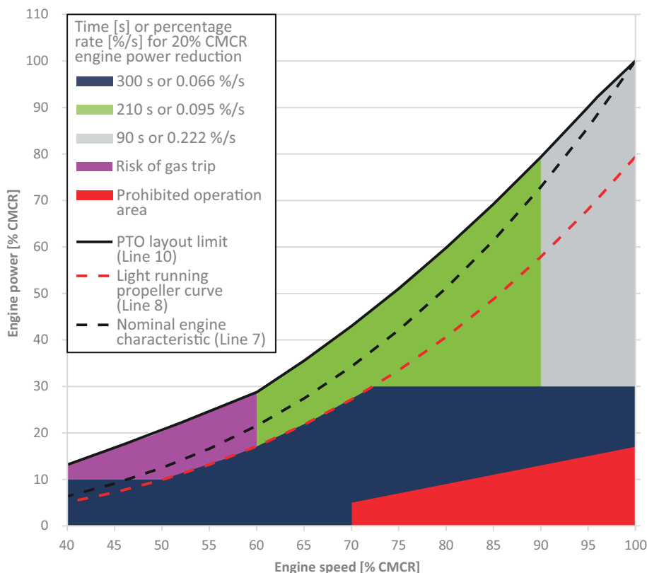
Figure 4-84 Maximum power decrease rate for PTO application in gas mode
