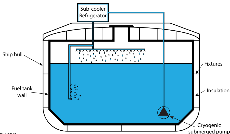
Figure 4-48 An LNG sub-cooler within an integrated tank
