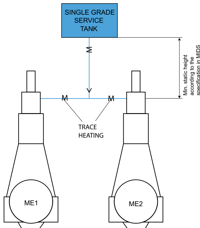
Figure 4-33 Cylinder LO system for fuel with ultra low sulphur content (maximum 0.10% m/m sulphur) or alternatively, a single grade cylinder LO is applied for fuel with very low sulphur content (maximum 0.50% m/m sulphur)
