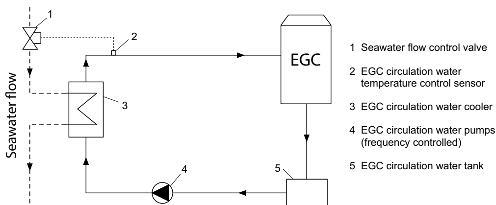
Figure 4-7 The EGC circulation water system
