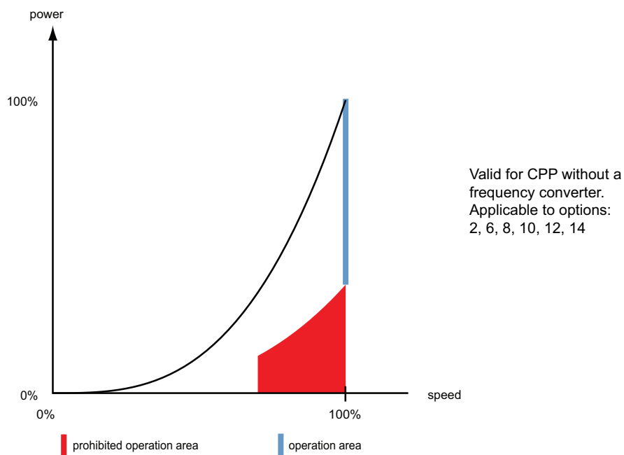
Figure 4-81 CPP in constant speed operation without frequency converter
