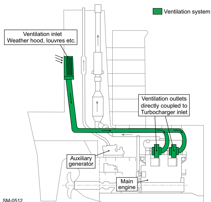
Figure 4-76 Ventilation system arrangement 2: Direct engine ventilation system
