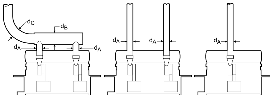
Figure 4-74 Determination of exhaust pipe diameter
