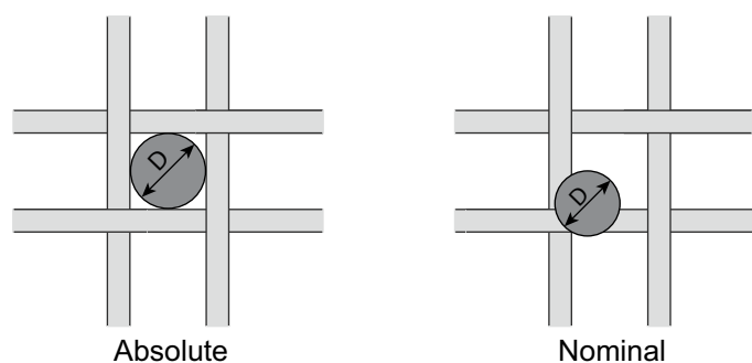
Figure 4-63 Mesh size difference between absolute and nominal
