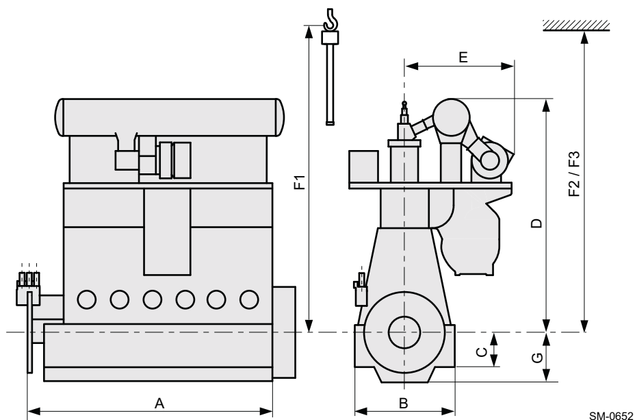
Figure 3-1 Engine dimensions
