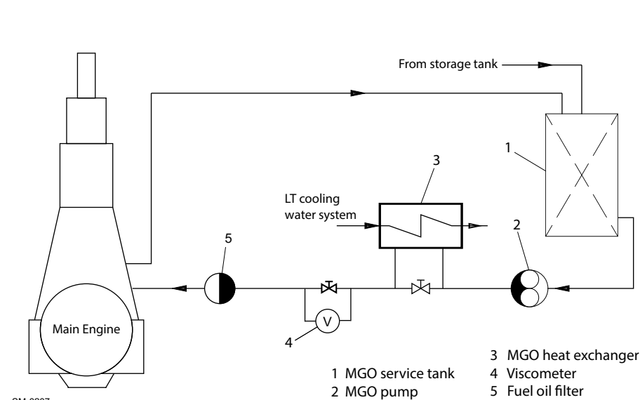
Figure 4-59 Pilot fuel oil system
