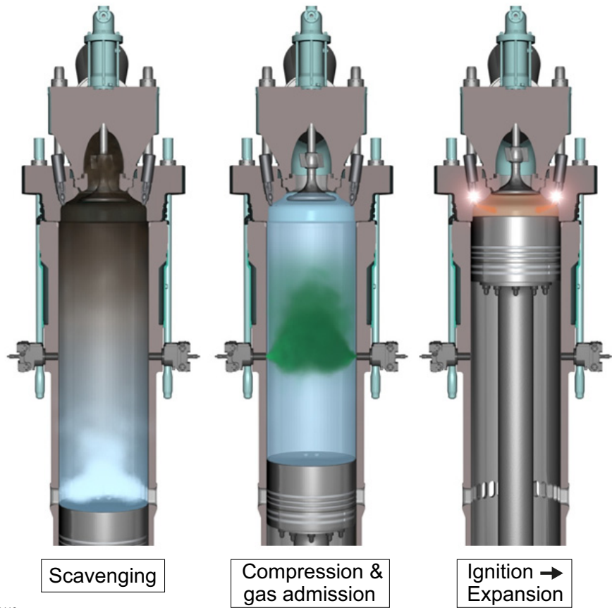
Figure 4-37 Lean burn with pilot ignition
