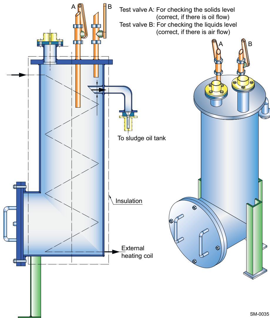
Figure 4-69 Design proposal of the WinGD sludge oil trap
