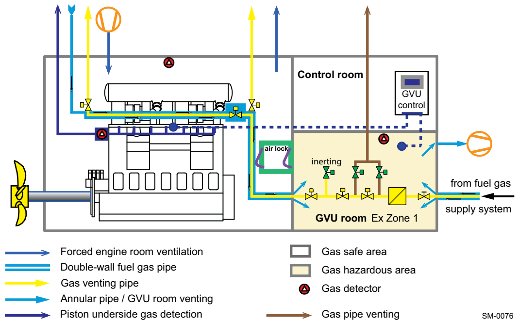
Figure 4-55 The GVO-OD™ from Wärtsilä
