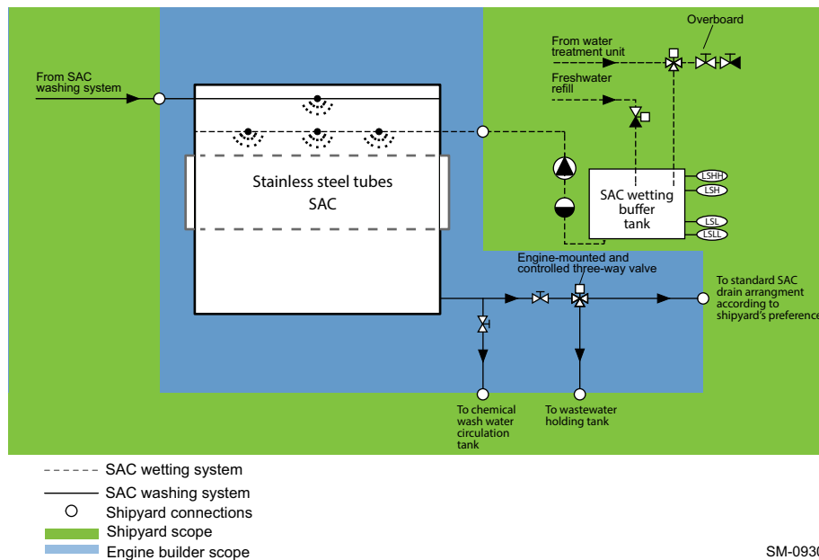
Figure 4-15 The SAC wetting system with the SAC wetting buffer tank arrangement SM-0930
