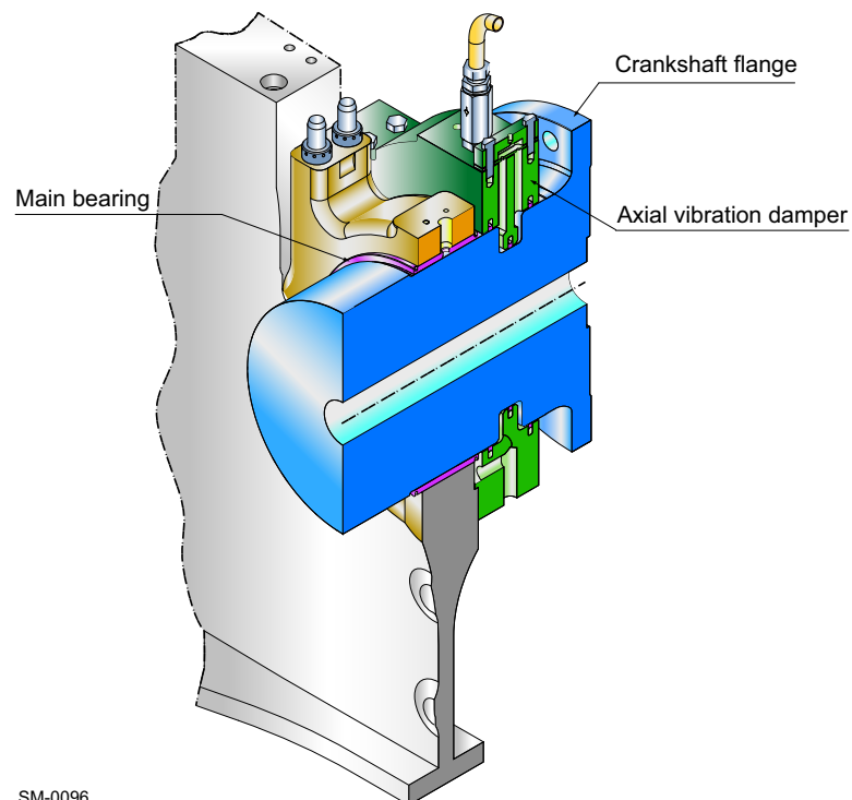
Figure 6-10 Example of axial vibration damper
