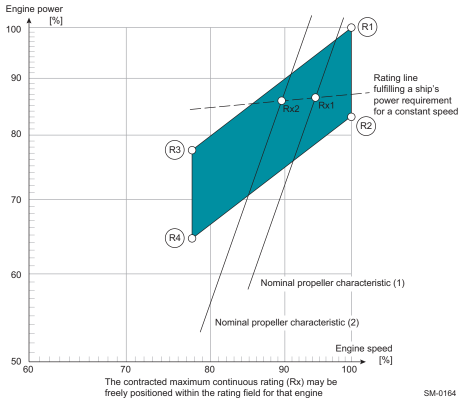
Figure 2-1 Rating field for the X62DF
