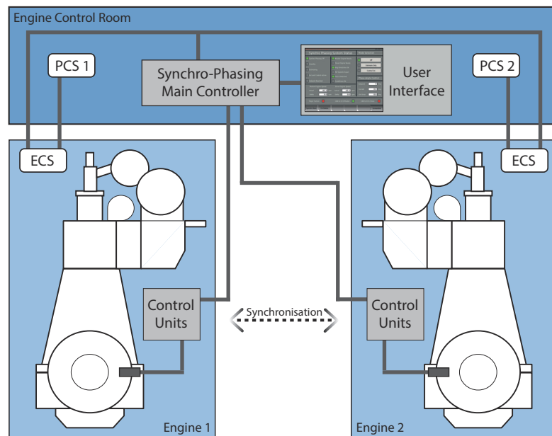
Figure 6-12 Synchro-Phasing system
