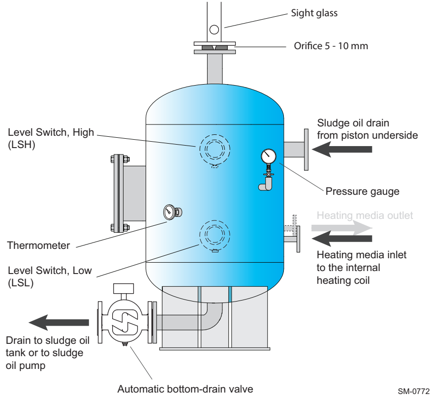
Figure 4-49 Design proposal of an automatically bottom-drained sludge oil trap
