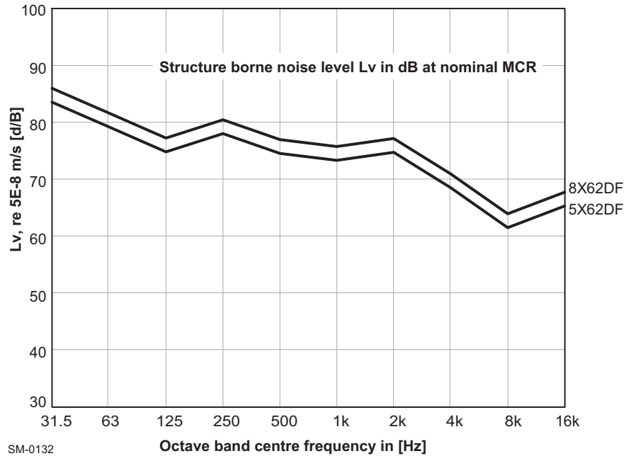
Figure 7-6 Structure-borne noise level at engine feet vertical
