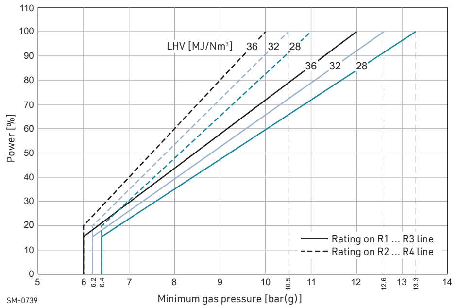
SM-0739 Figure 4-28 Design fuel gas supply pressure requirements
