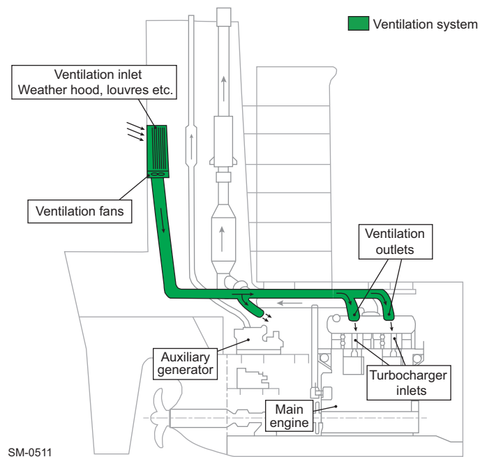
Figure 4-67 Ventilation system arrangement 1 — Engine room ventilation system
