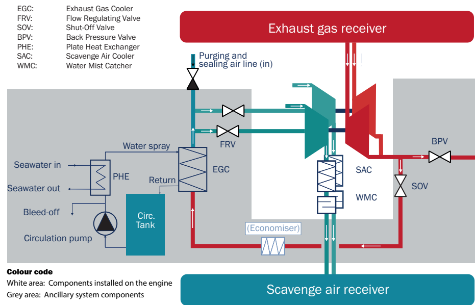
Figure 4-3 The iCER system with the exhaust gas return pipe routed to the turbocharger connection from below
