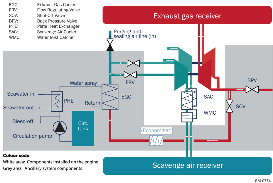
Figure 1-4 The iCER system with the exhaust gas return pipe routed to the turbo-charger connection from below
