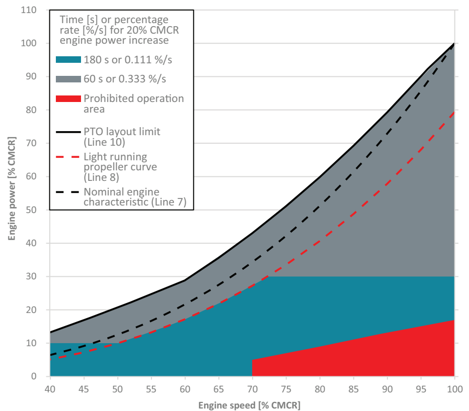
Figure 4-72 Maximum power increase rate for PTO application in gas mode
