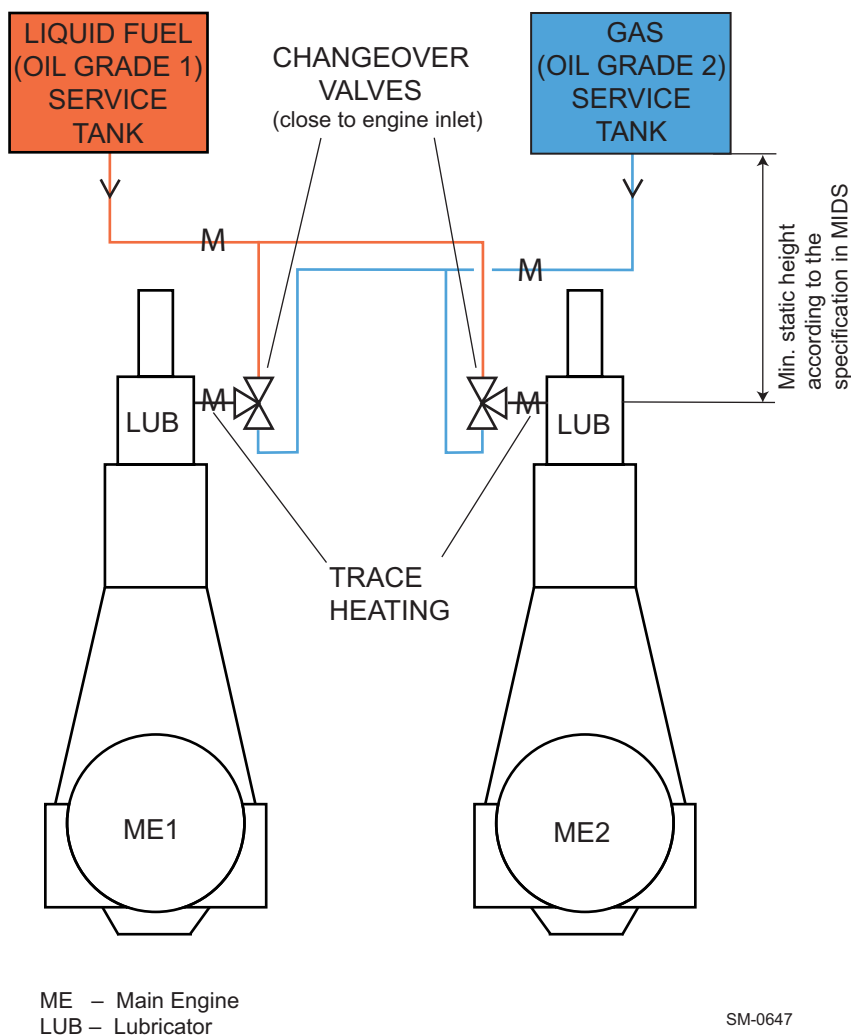
Figure 4-25 Dual cylinder lubricating oil installation, enabling independent gas and liquid fuel (maximum 0.50% m/m sulphur) operation with a manual changeover valve
