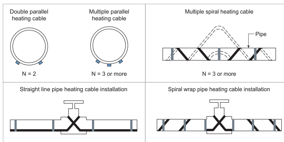
Figure 4-27 Trace heating cable arrangement
