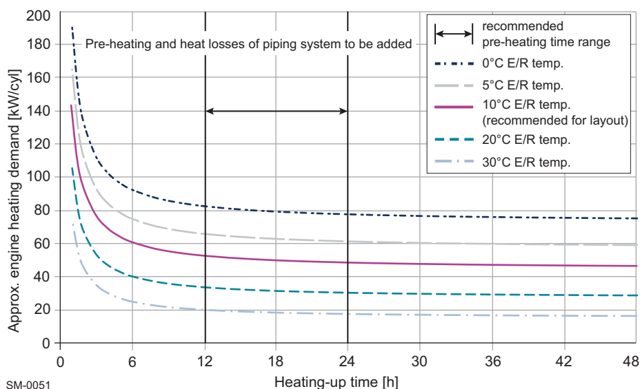
Figure 4-23 Pre-heating power requirement per cylinder
