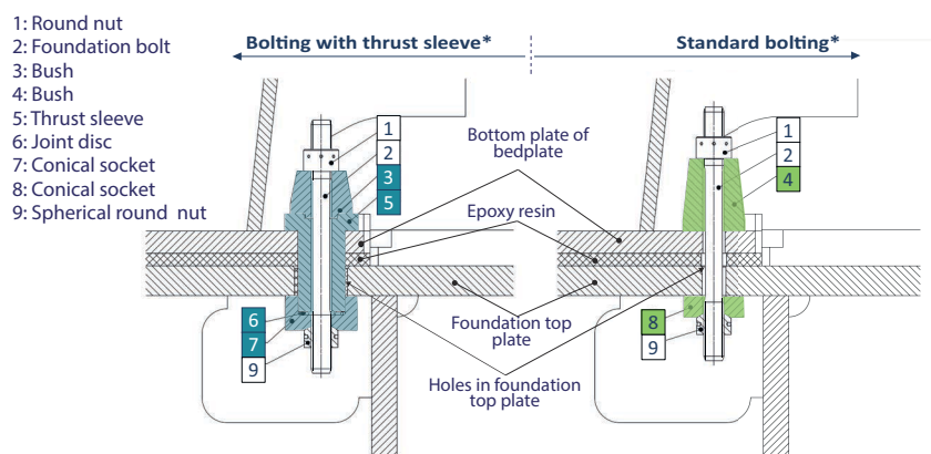
Figure 3-6 Foundation bolting
