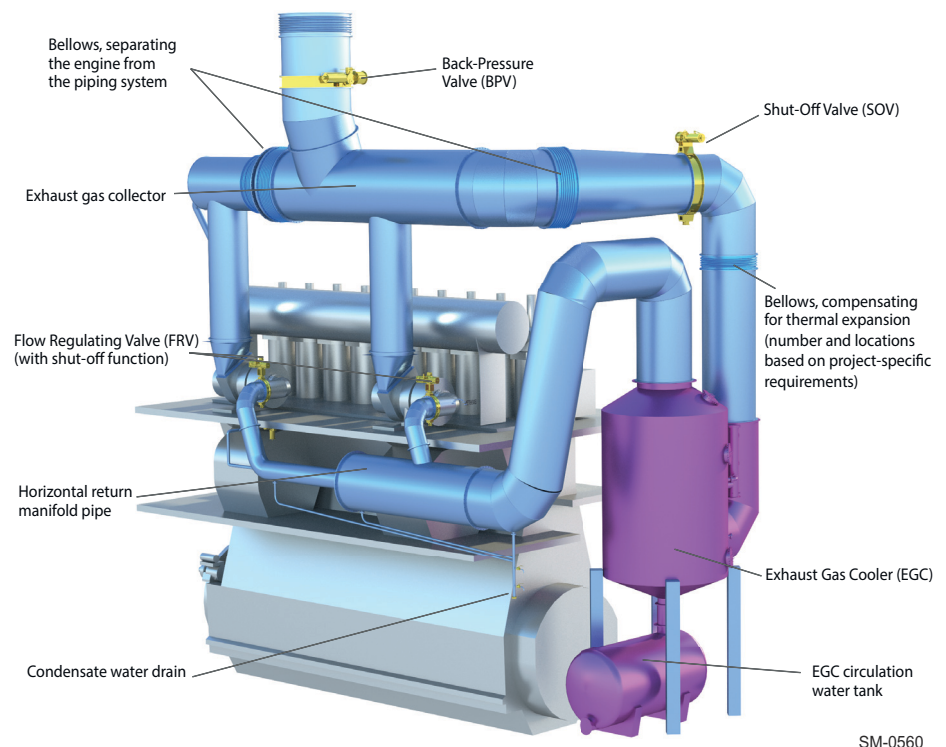
Figure 4-2 Overview of the components for the iCER system
