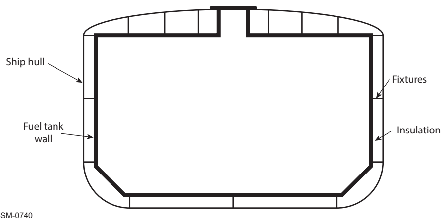
Figure 4-33 Section view of an integrated membrane tank
