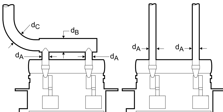
Figure 4-66 Determination of exhaust pipe diameter
