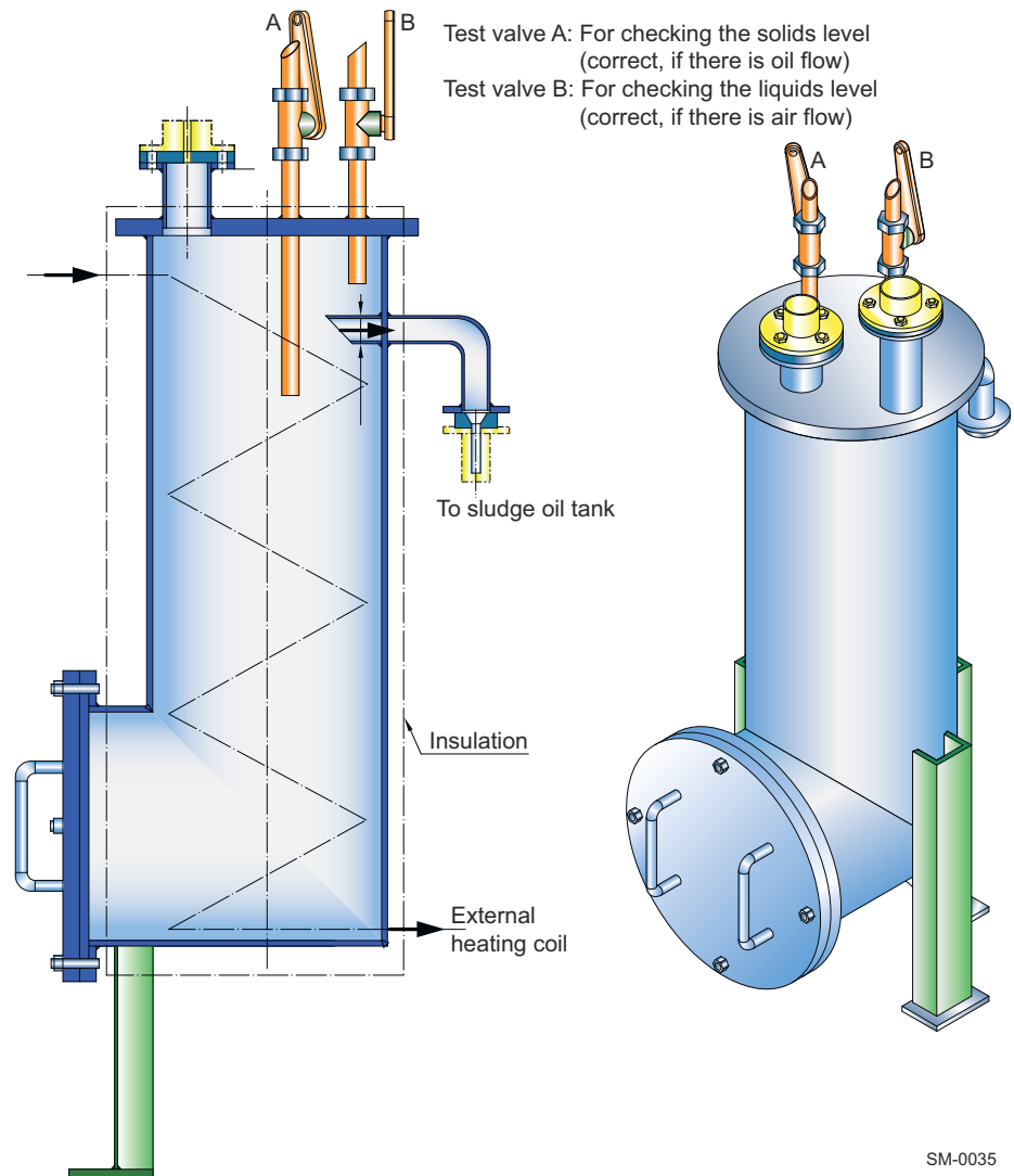
Figure 4-61 Design proposal of WinGD's sludge oil trap
