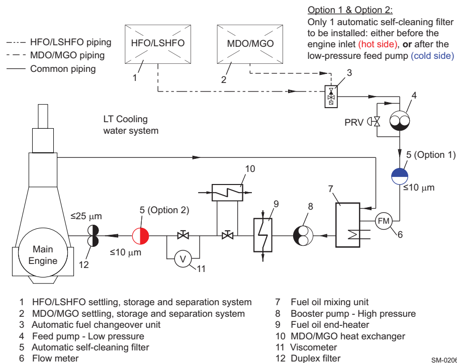
Figure 4-56 Fuel oil filter arrangement 'A'
