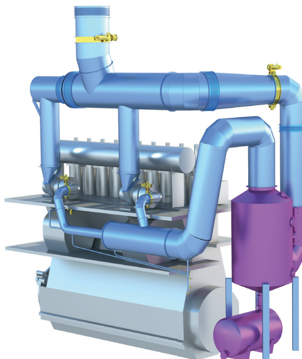
Figure 4-14 Example of an exhaust gas piping arrangement
