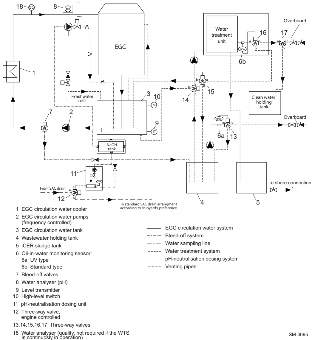
Figure 4-6 The iCER drainage system valid for all iCER operating mode options
