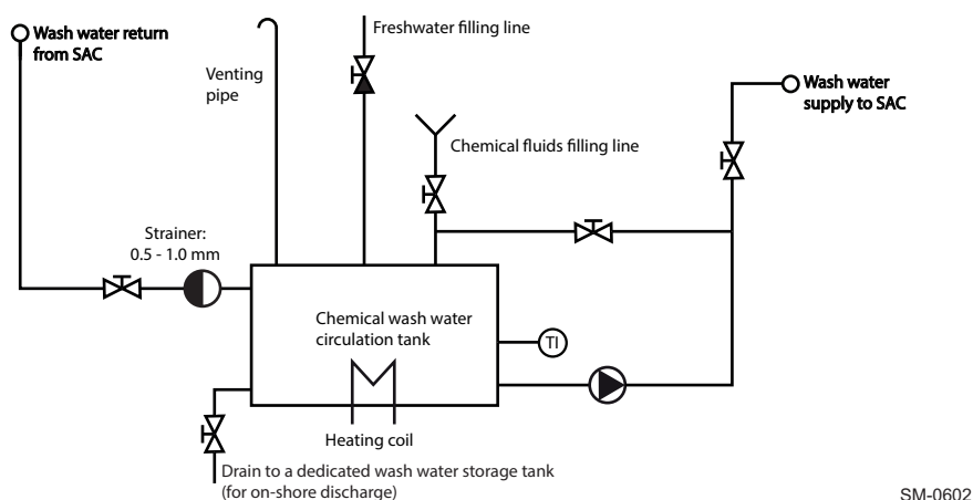
Figure 4-65 Offline SAC washing system (external system)
