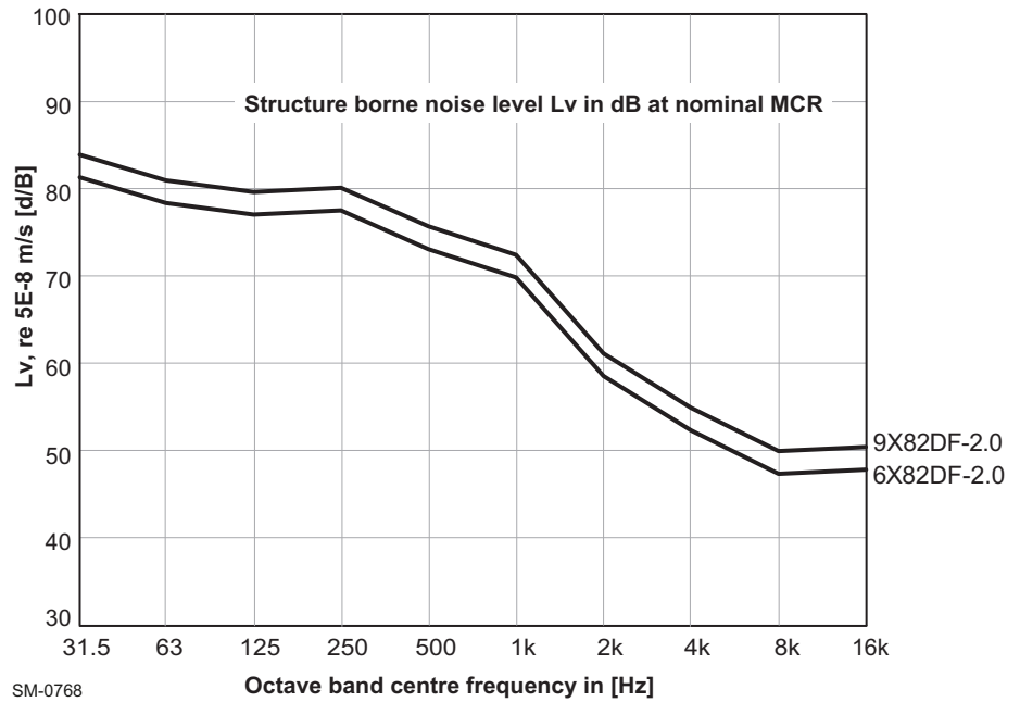
Figure 7-7 Structure-borne noise level at engine feet vertical
