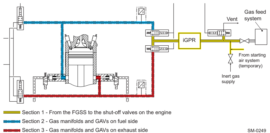
Figure 4-49 Gas leak test sequence (engines with iGPR)
