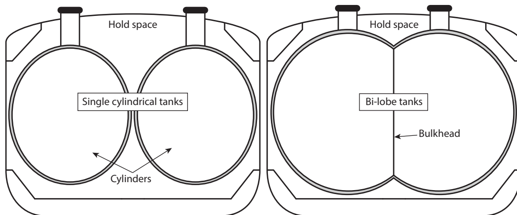
Figure 4-36 Section view of different free-standing Type C tanks installed below the deck
