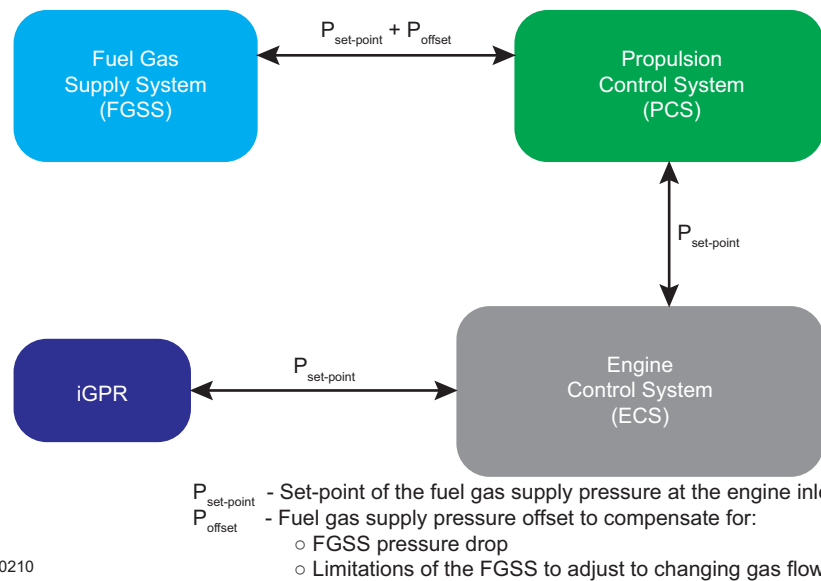
Figure 4-43 Fuel gas supply pressure control at the engine inlet (engines with iGPR)
