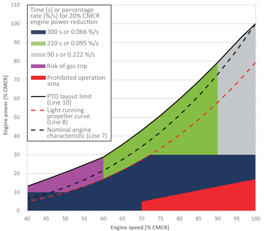
Figure 4-73 Maximum power decrease rate for PTO application in gas mode
