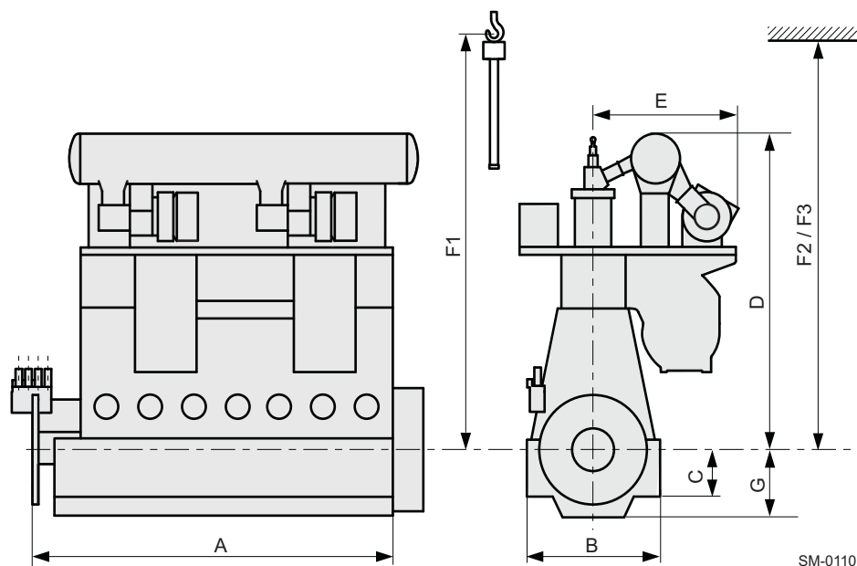
Figure 3-1 Engine dimensions
