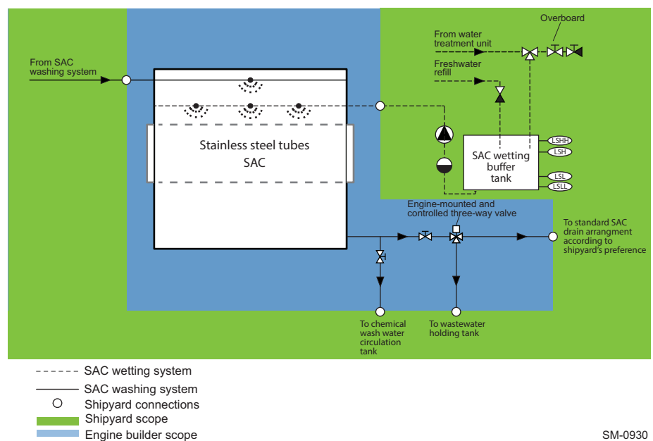
Figure 4-12 The SAC wetting system with the SAC wetting buffer tank arrangement
