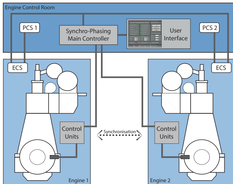
Figure 6-16 Synchro-Phasing system
