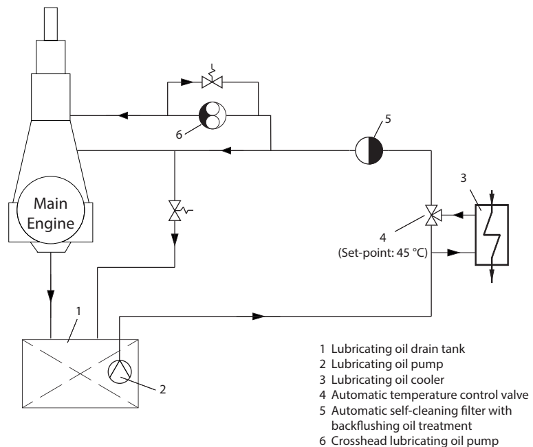
Figure 4-24 Lubricating oil system
