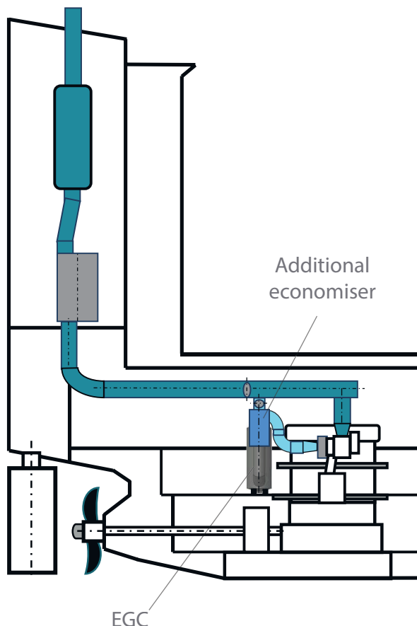
Figure 4-15 The short route arrangement
