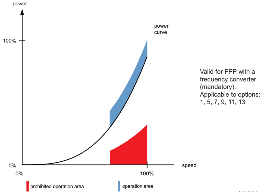
Figure 4-71 FPP with mandatory frequency converter
