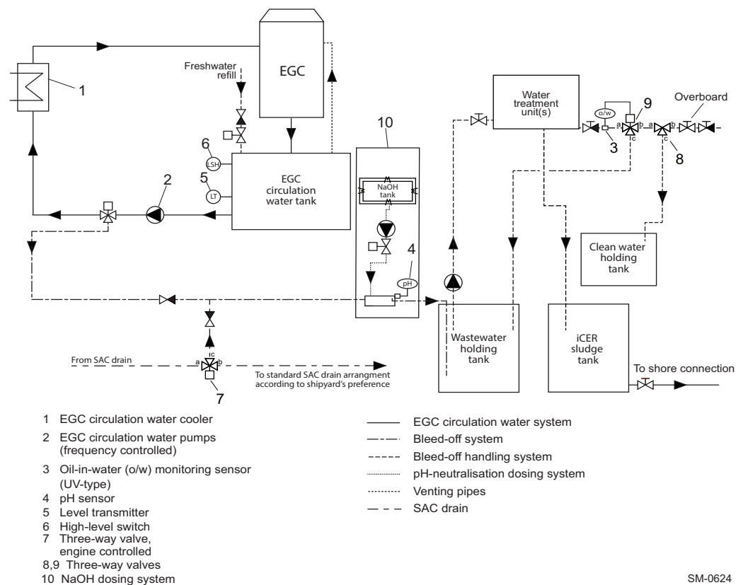
Figure 4-5 The iCER drainage system for installations which run the iCER system exclusively in gas mode
