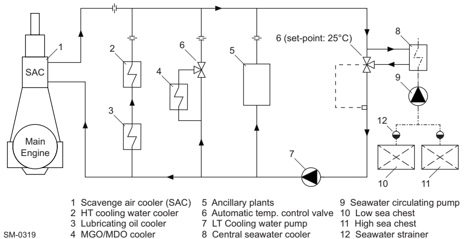
Figure 4-19 LT cooling water circuit — Single set-point temperature
