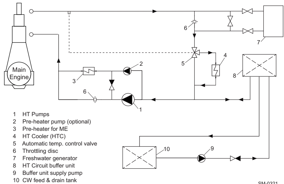
Figure 4-22 HT cooling water circuit
