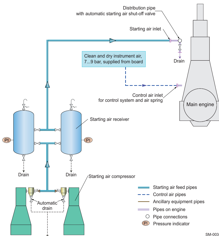
Figure 4-60 Air supply system
