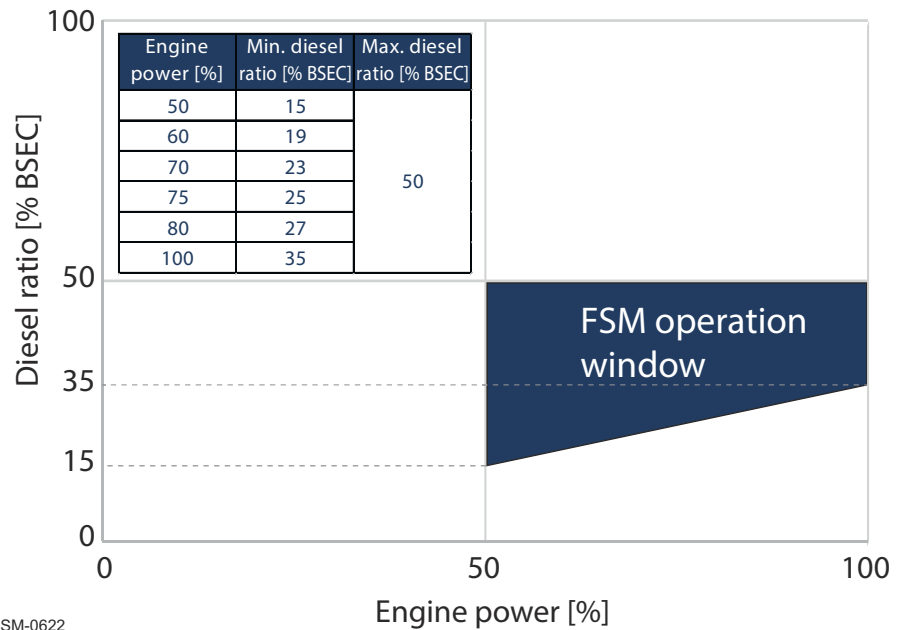
Figure 1-7 Fuel sharing mode — available operating window
