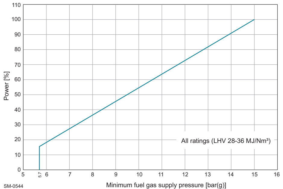
SM-0544 Figure 4-42 Design fuel gas supply pressure requirements
