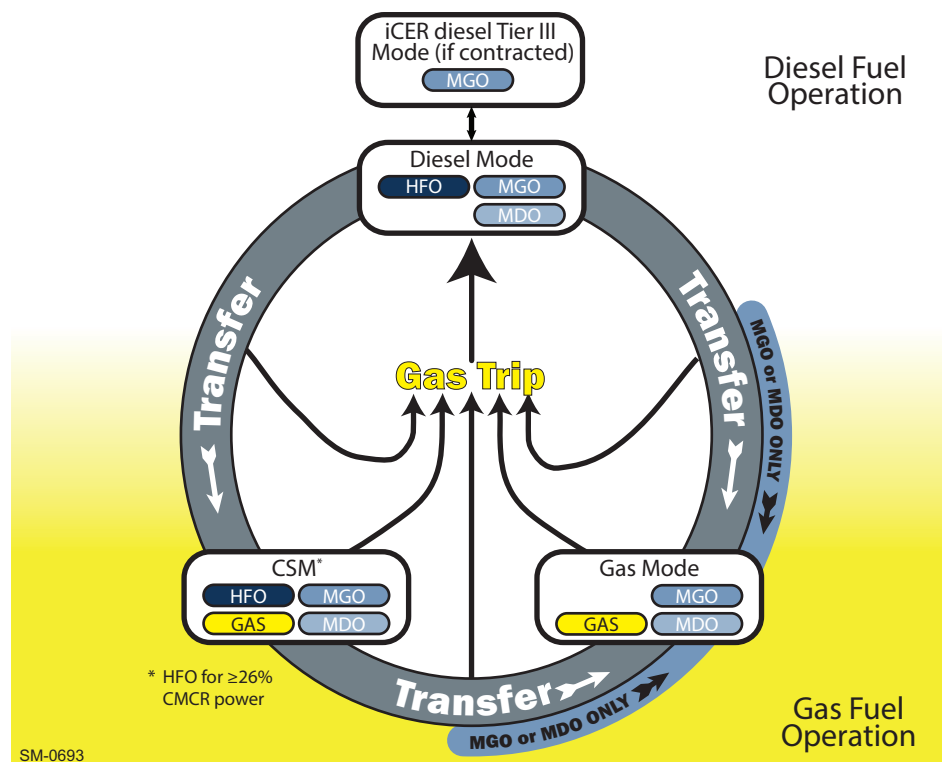
Figure 1-9 If FSM is not contracted, the fuel transfers and gas trips
