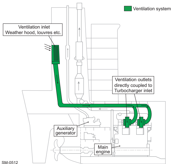
Figure 4-68 Ventilation system arrangement 2 — Direct engine ventilation system
