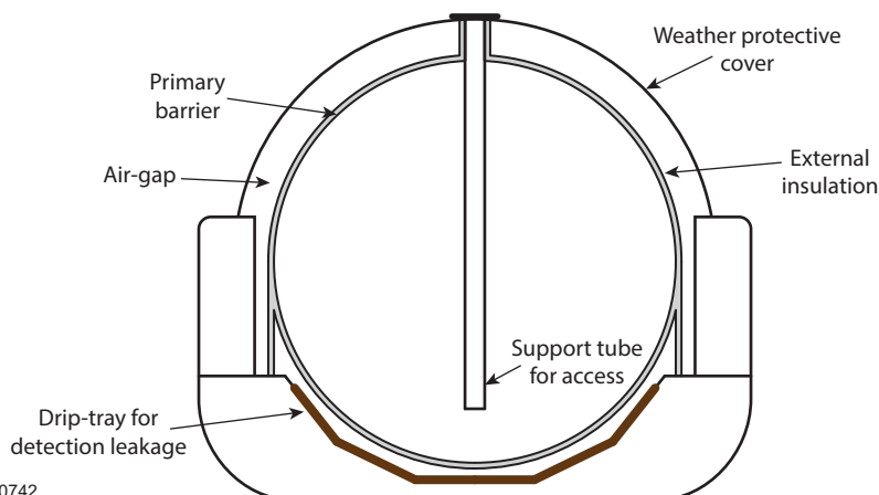
Figure 4-35 Section view of a free-standing Type B tank of moss design
