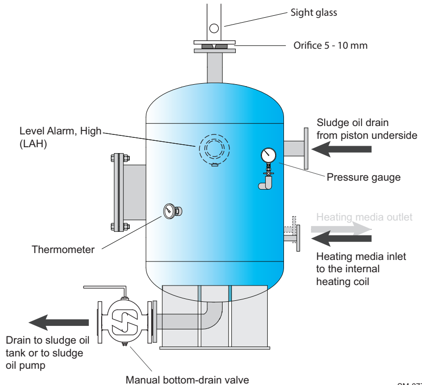
Figure 4-62 Design proposal of a manually bottom-drained sludge oil trap
