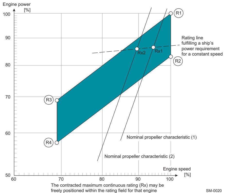
Figure 2-1 Rating field for the X82DF-2.0
