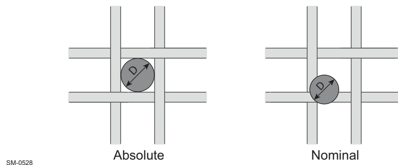
Figure 4-55 Mesh size difference between absolute and nominal
