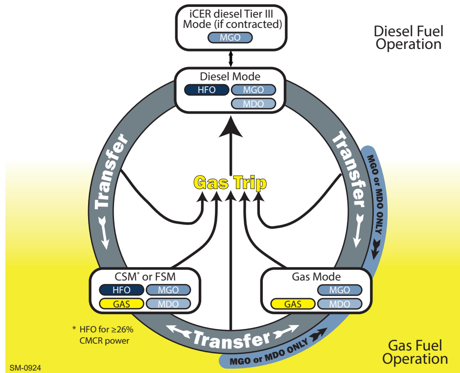
Figure 1-10 If FSM is contracted, the fuel transfers and gas trips
