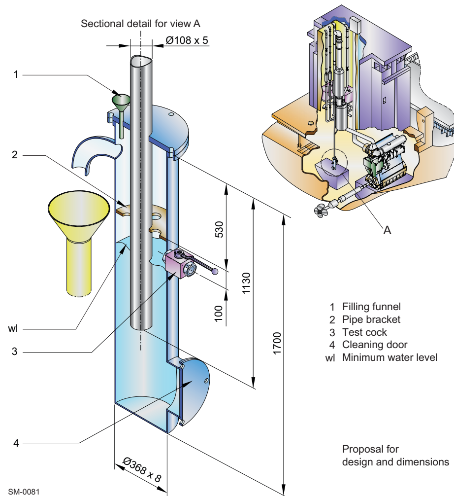
Figure 4-64 Arrangement of automatic water drain
