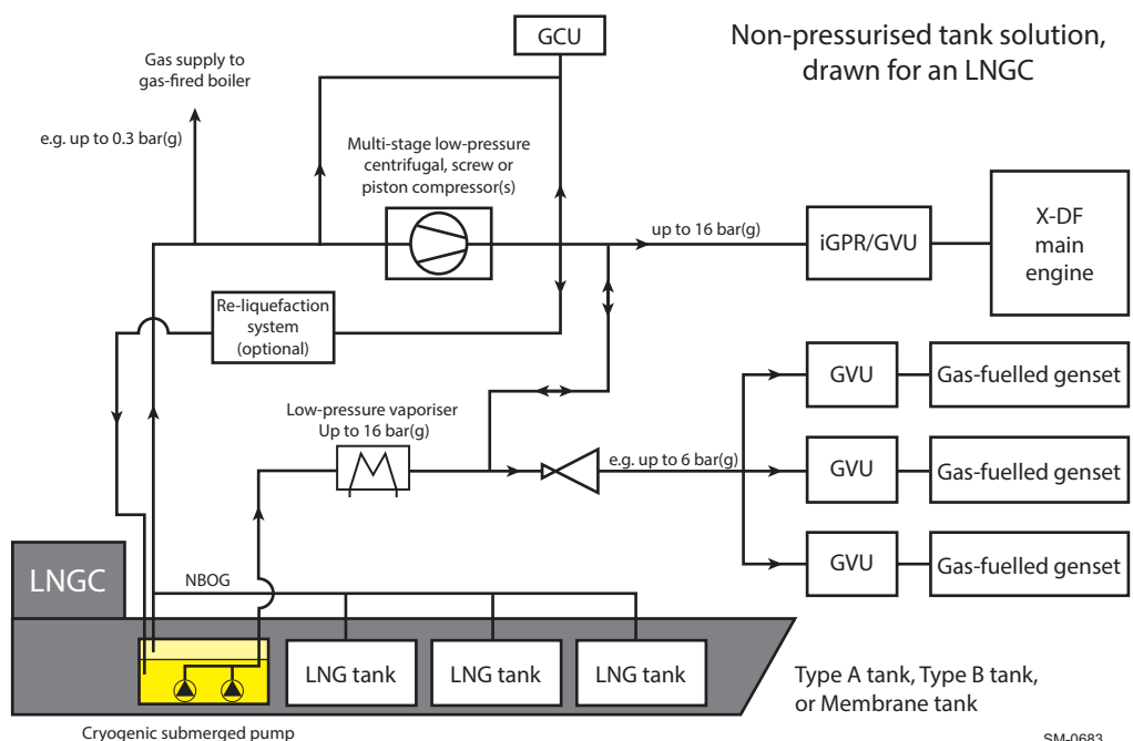
Figure 4-40 Non-pressurised tank solution, drawn for an LNGC
