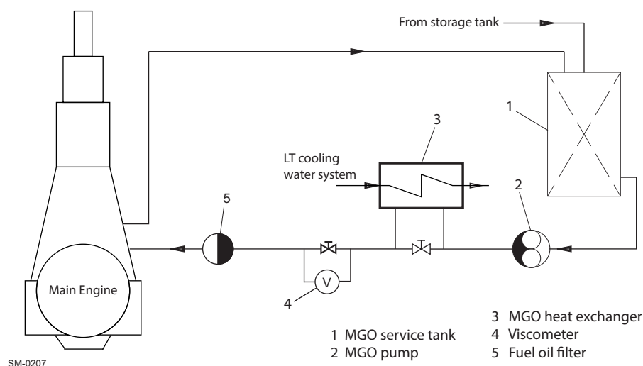
Figure 4-51 Pilot fuel oil system
