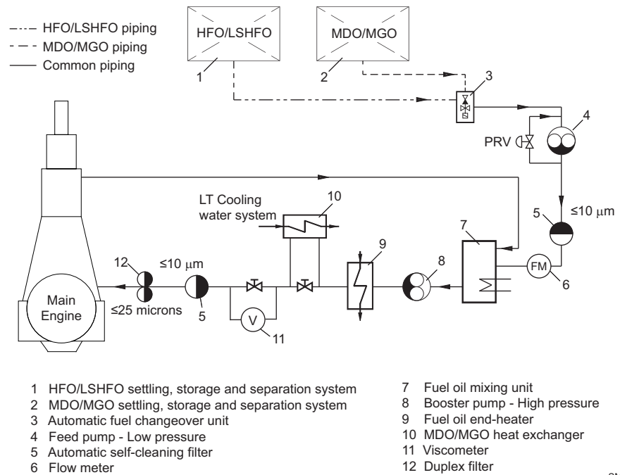
Figure 4-53 Fuel oil system
