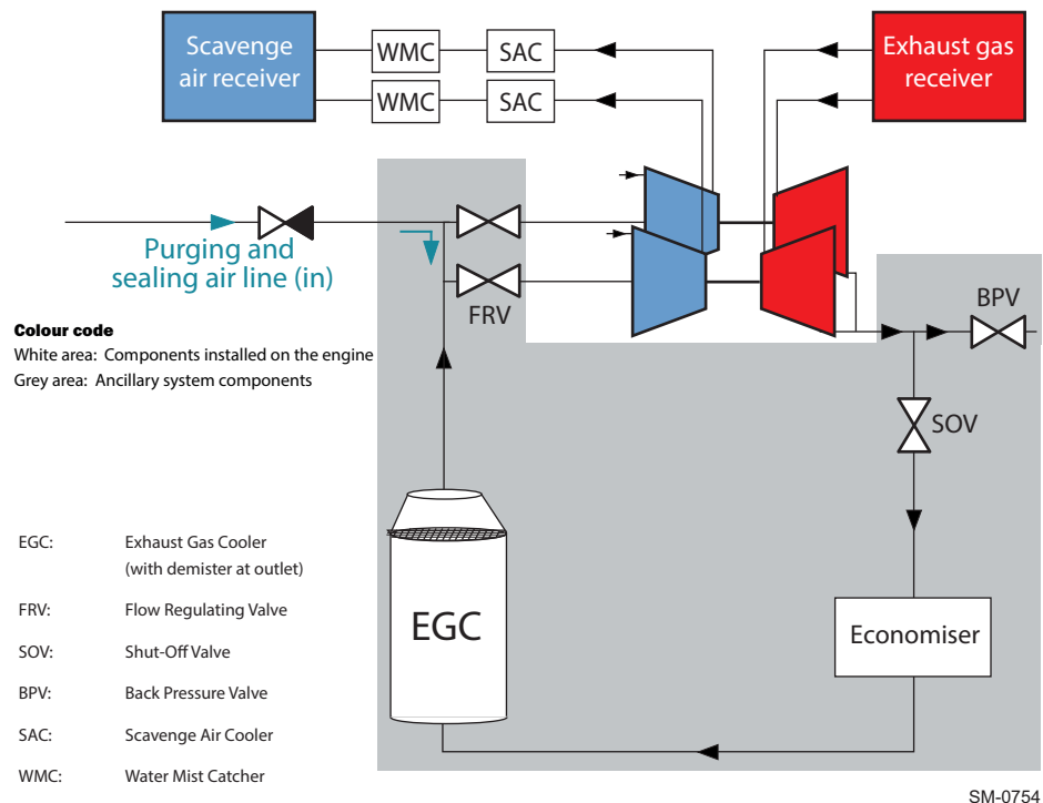
Figure 4-13 The iCER exhaust gas system with the exhaust gas return pipe routed to the turbocharger connection from below
