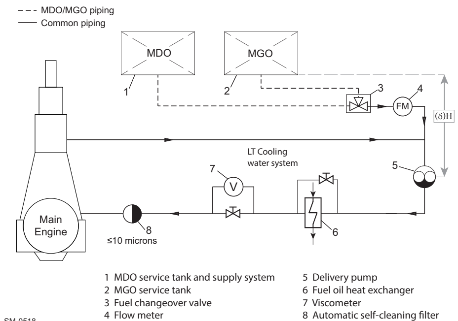
Figure 4-58 Fuel oil system — Arrangement with only MDO/MGO or MGO
