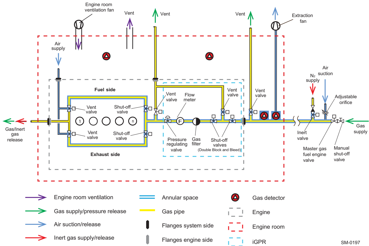
Figure 4-46 Fuel gas supply system with the iGPR
