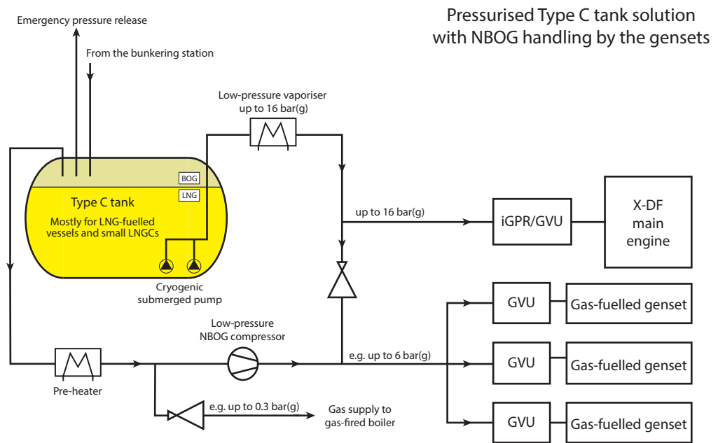
Figure 4-38 Pressurised Type C tank solution with NBOG handling by the gensets
