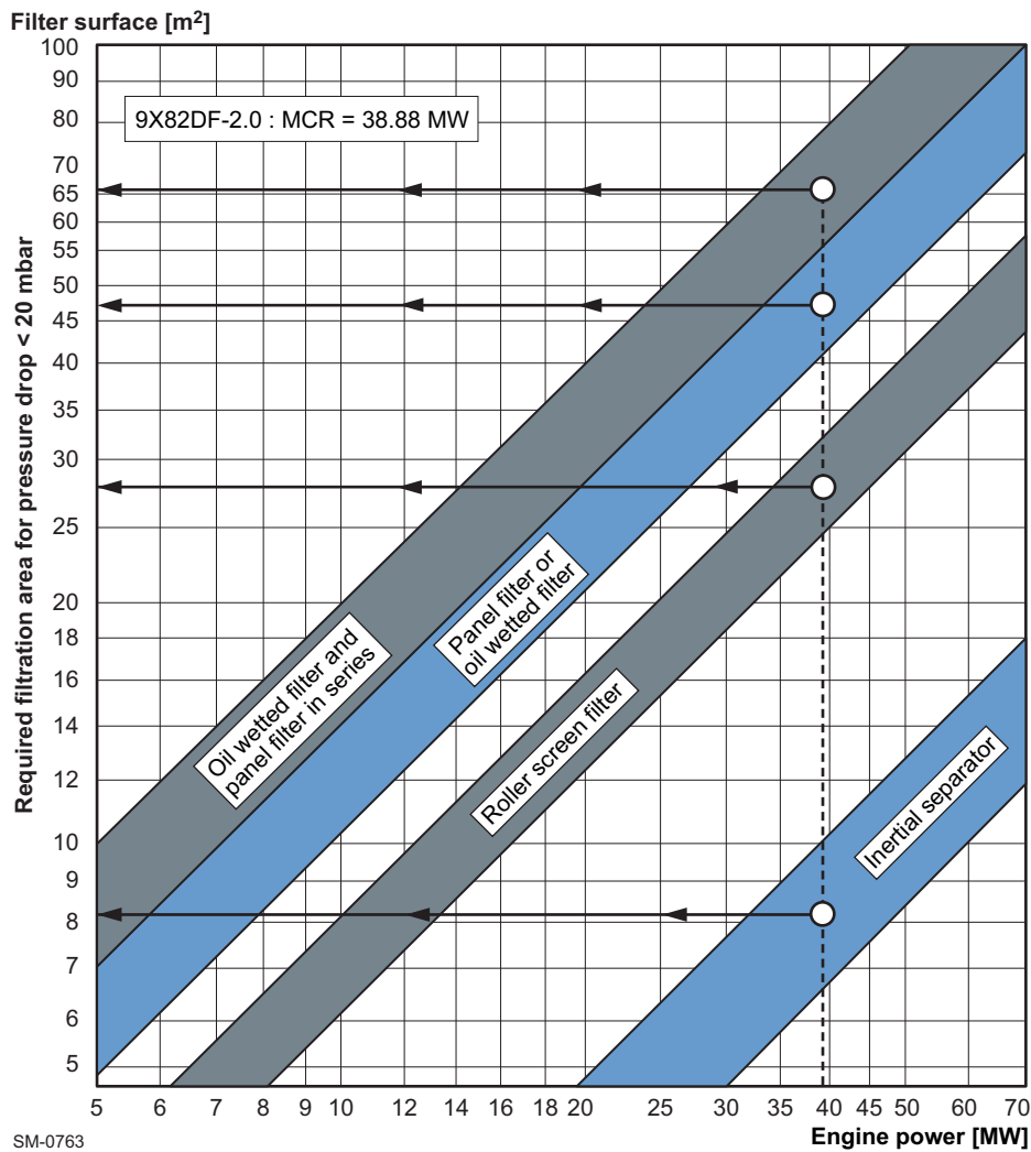
Figure 4-69 Air filter size (example for 9-cyl. engine)
