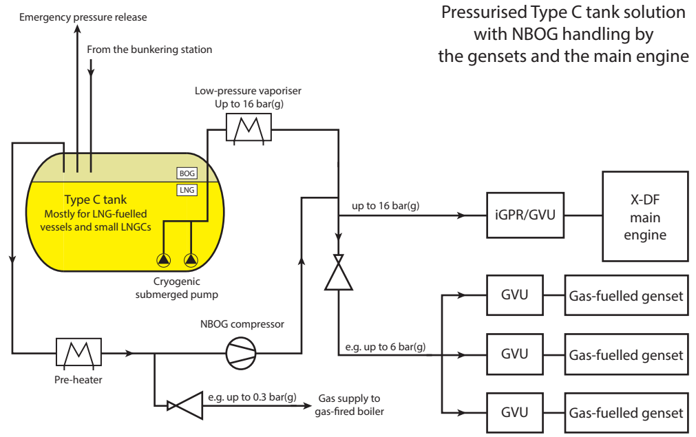
Figure 4-39 Pressurised Type C tank solution with NBOG handling by the gensets and the main engine
