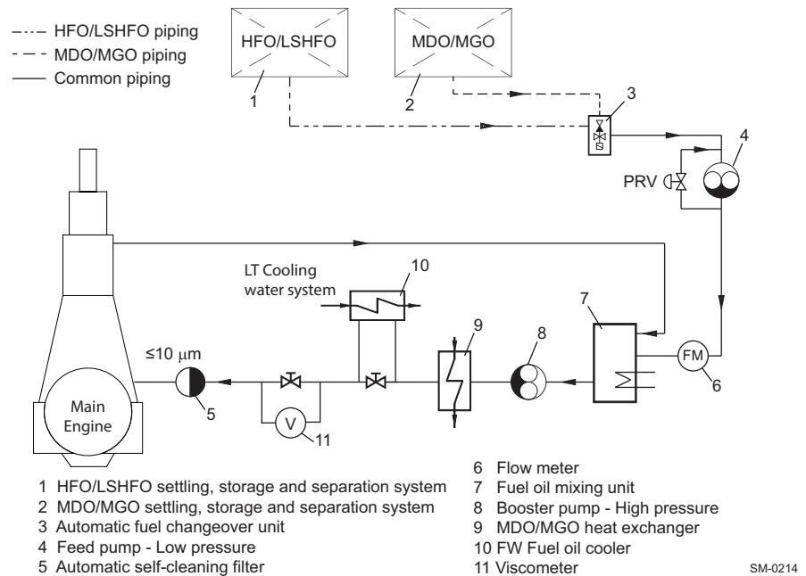
Figure 4-57 Fuel oil filter arrangement ‘B’
