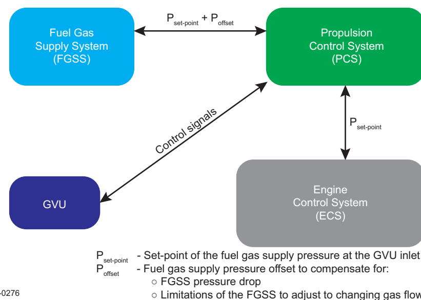
Figure 4-44 Fuel gas supply pressure control at the GVU inlet (engines with GVU)
