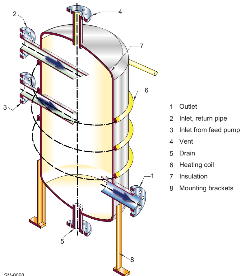
Figure 4-54 Mixing unit
