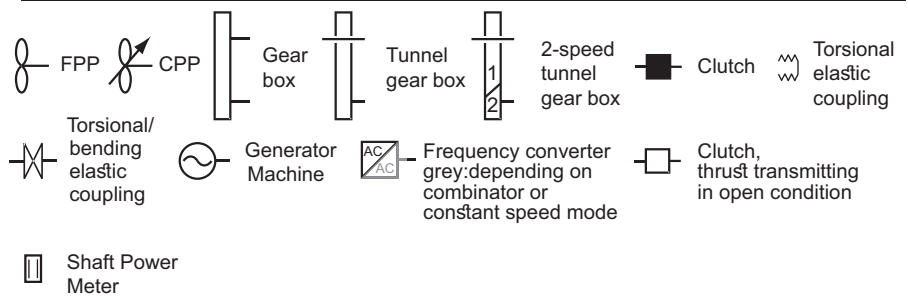
Figure 4-70 Arrangements for PTO, PTI, PTH
