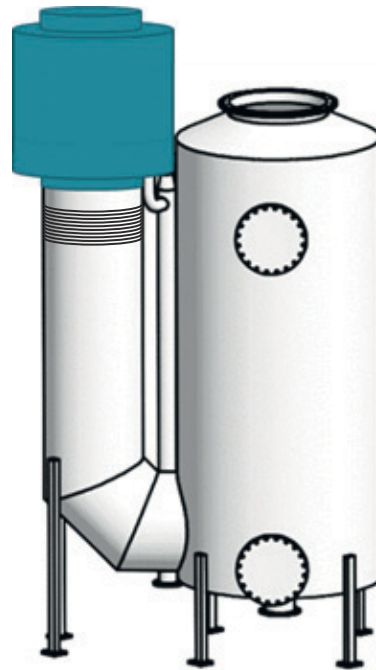
Figure 4-17 Arrangement of the additional economiser (Source: Alfa Laval)
