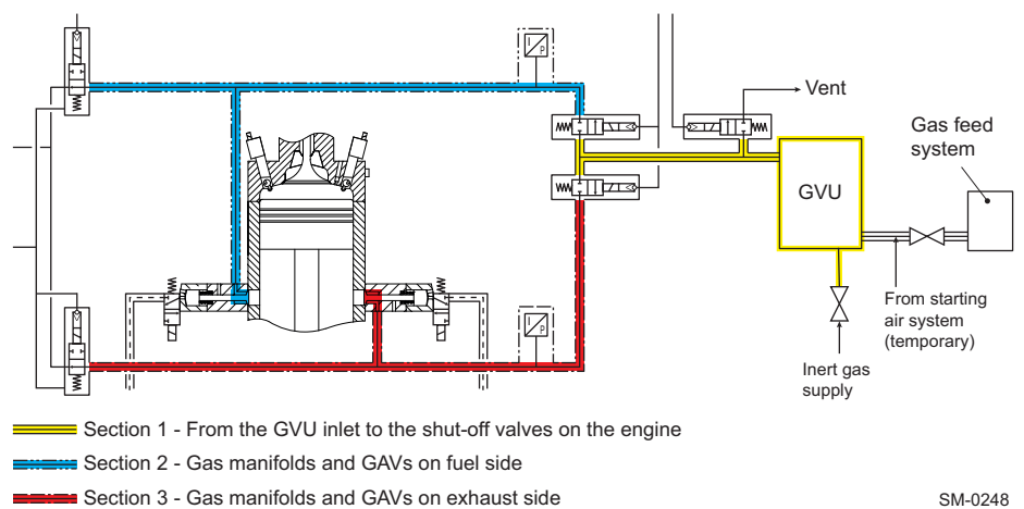
Figure 4-50 Gas leak test sequence (engines with GVU)
