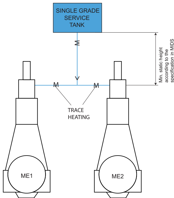
Figure 4-26 Cylinder lubricating oil system for fuel with ultra low sulphur content (maximum 0.10% m/m sulphur) or alternatively, a single grade cylinder lubricating oil is applied for fuel with very low sulphur content (maximum 0.50% m/m sulphur)
