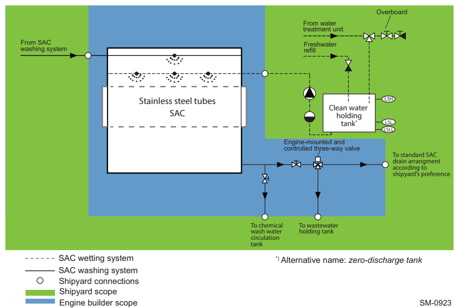
Figure 4-11 The SAC wetting system with the clean water holding tank arrangement
