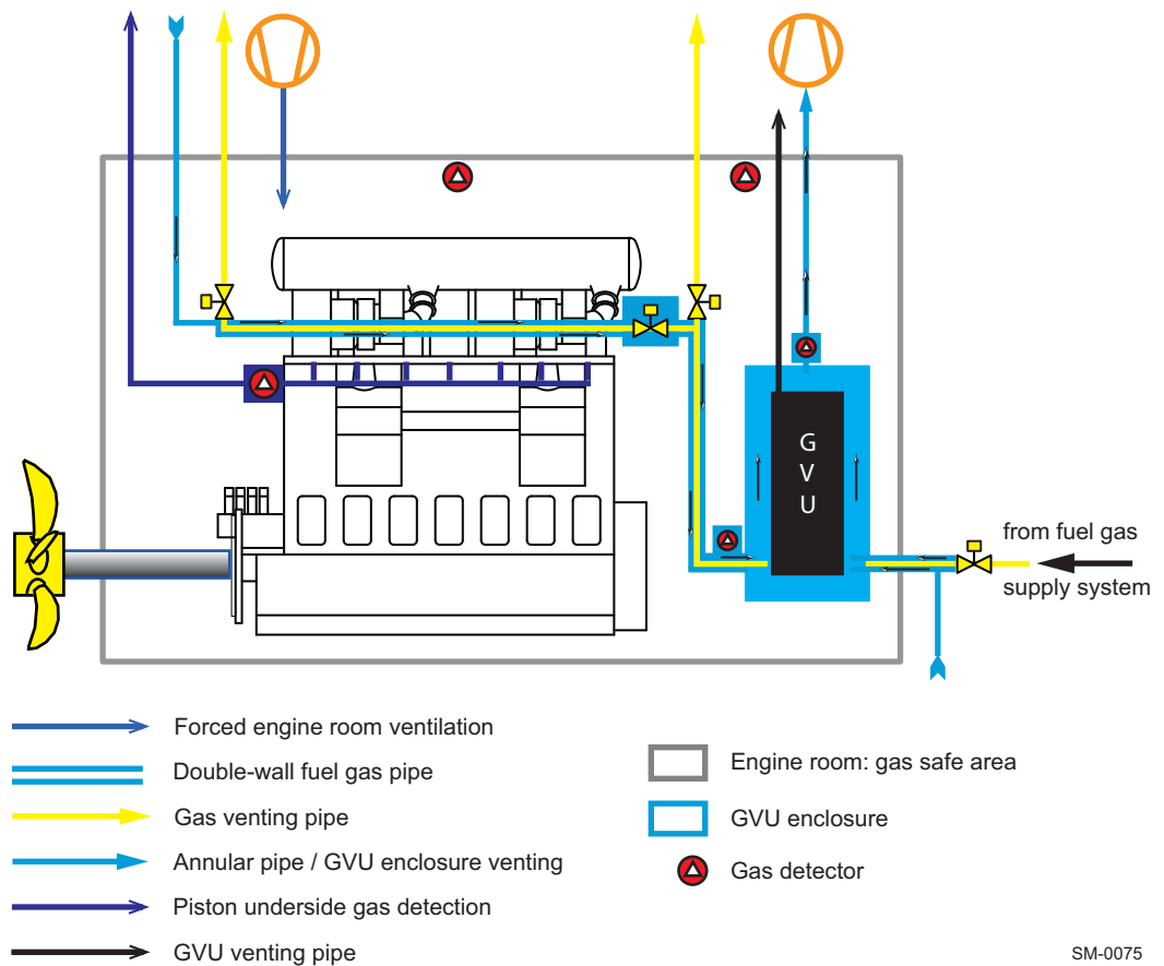
Figure 4-48 The GVU-ED™ from Wärtsilä
