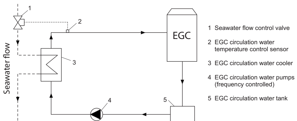
Figure 4-4 The EGC circulation water system
