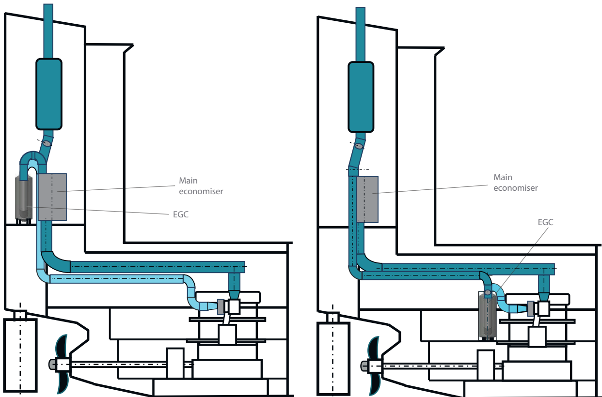
Figure 4-16 The long route arrangement
