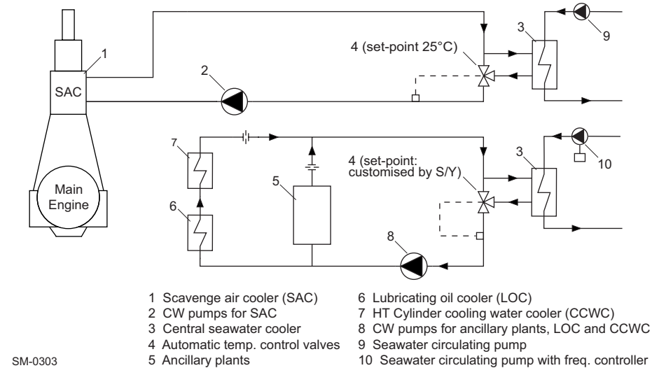
Figure 4-21 Separate SAC and LT cooling circuits
