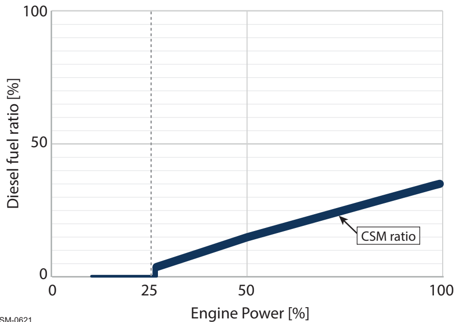
SM-0621 Figure 1-6 Diesel fuel ratio during active CSM
