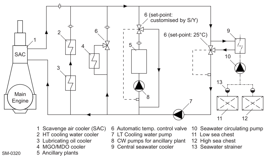
Figure 4-20 LT cooling water circuit — Dual set-point temperatures
