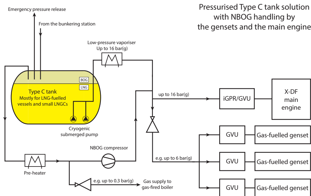
Figure 4-23 Pressurised Type C tank solution with NBOG handling by the gensets and the main engine
