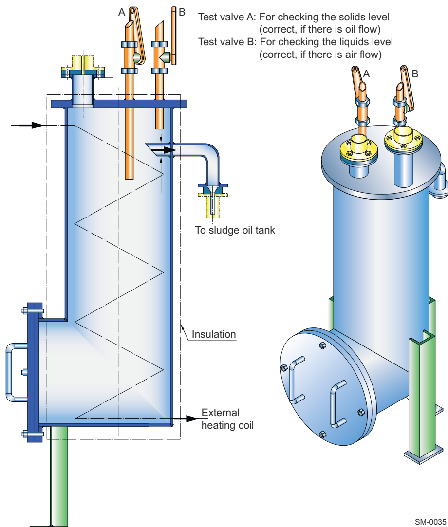
Figure 4-45 Design proposal of WinGD's sludge oil trap
