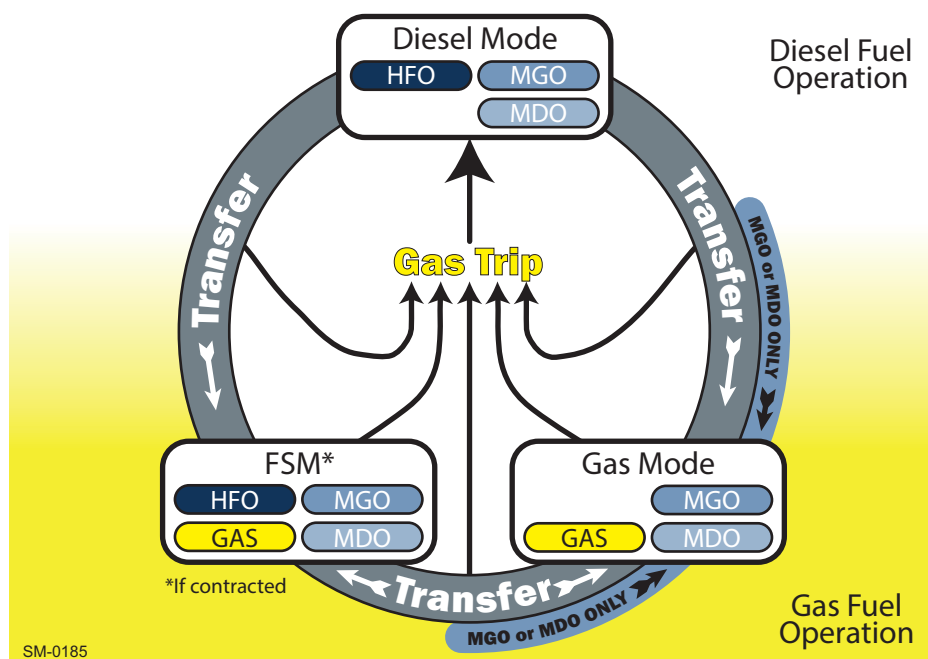
Figure 1-7 Fuel transfers and gas trips
