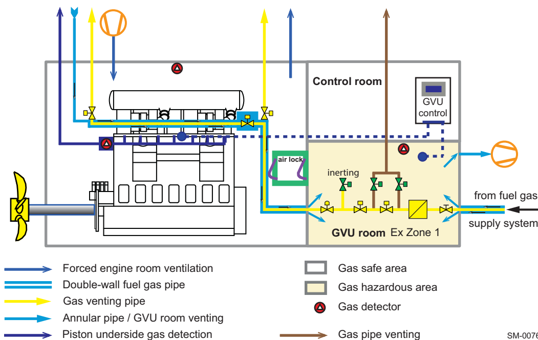
Figure 4-31 The GVU-OD™ from Wärtsilä
