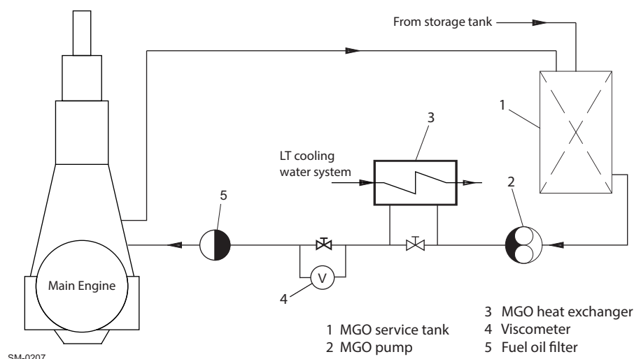
Figure 4-35 Pilot fuel oil system
