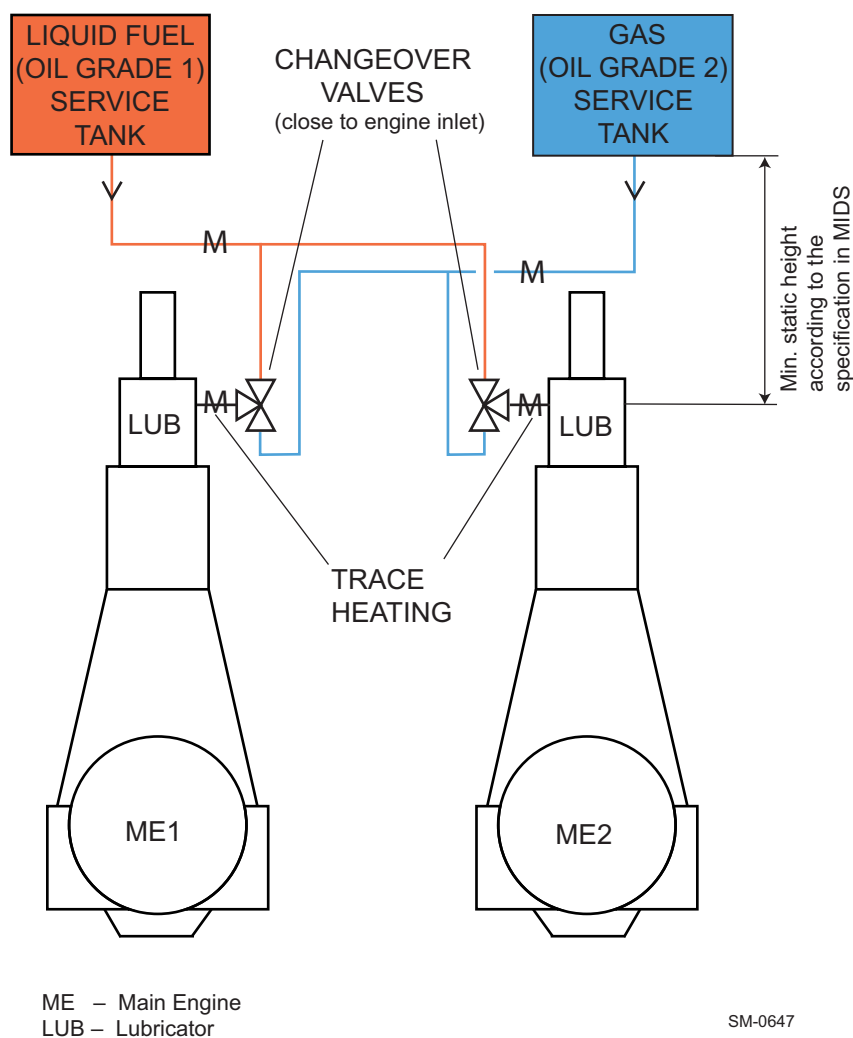
Figure 4-9 Dual cylinder lubricating oil installation, enabling independent gas and liquid fuel (maximum 0.50% m/m sulphur) operation with a manual changeover valve
