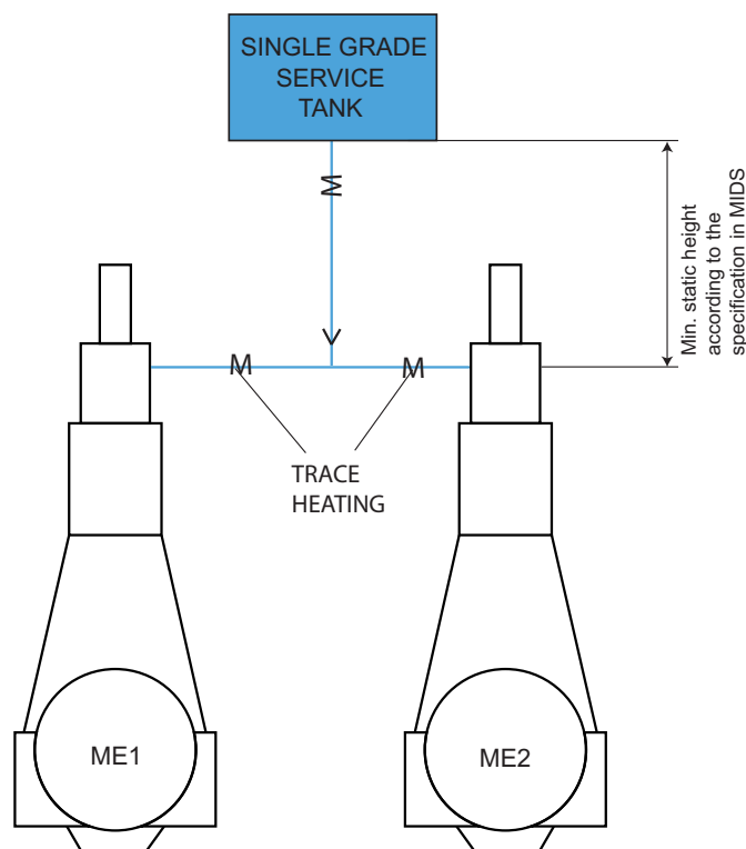
Figure 4-10 Cylinder lubricating oil system for fuel with ultra low sulphur content (maximum 0.10% m/m sulphur) or alternatively, a single grade cylinder lubricating oil is applied for fuel with very low sulphur content (maximum 0.50% m/m sulphur)
