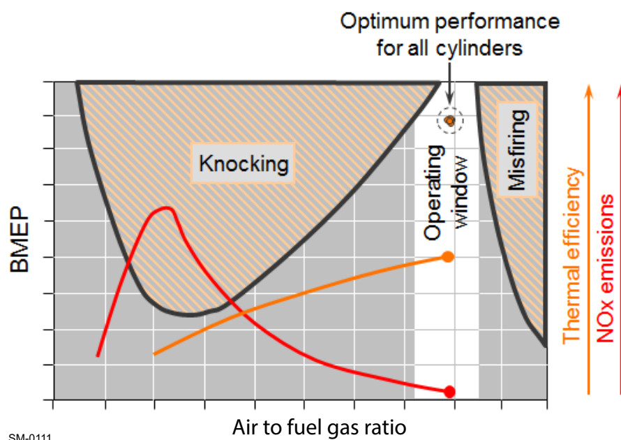
Figure 4-15 Lean-burn operation window
