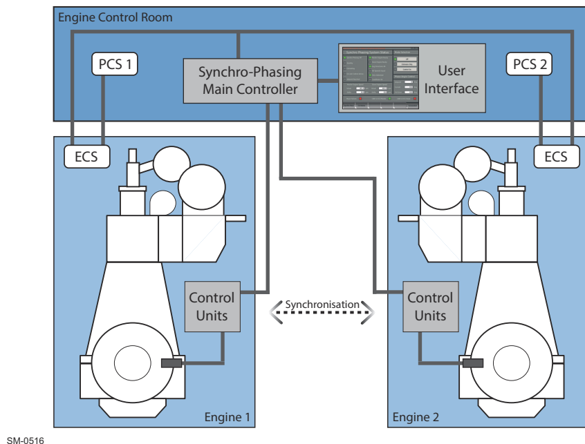
Figure 6-18 Synchro-Phasing system
