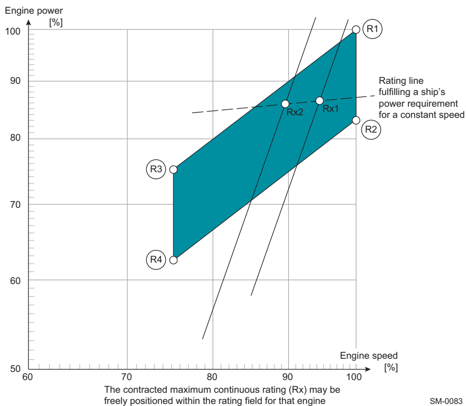
Figure 2-1 Rating field for the X52DF-1.1
