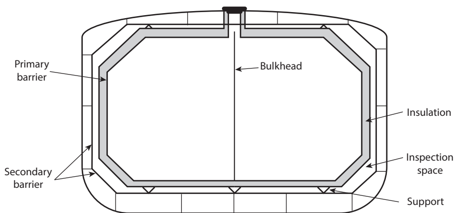
Figure 4-18 Section view of a free-standing Type A tank
