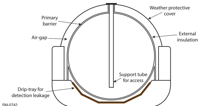
Figure 4-19 Section view of a free-standing Type B tank of moss design
