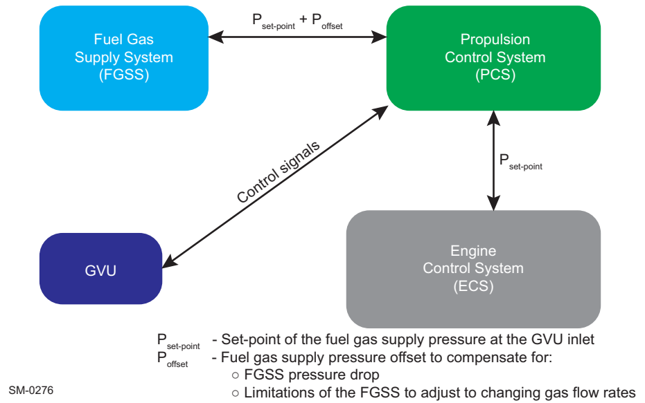
Figure 4-28 Fuel gas supply pressure control at the GUV inlet (engines with GUV)
