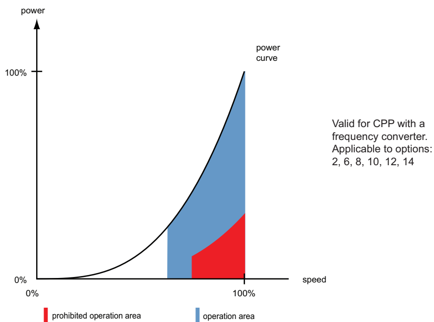
Figure 4-55 CPP in combination with an optional frequency converter
