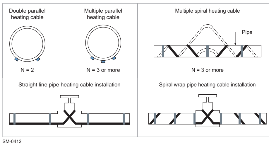
Figure 4-11 Trace heating cable arrangement
