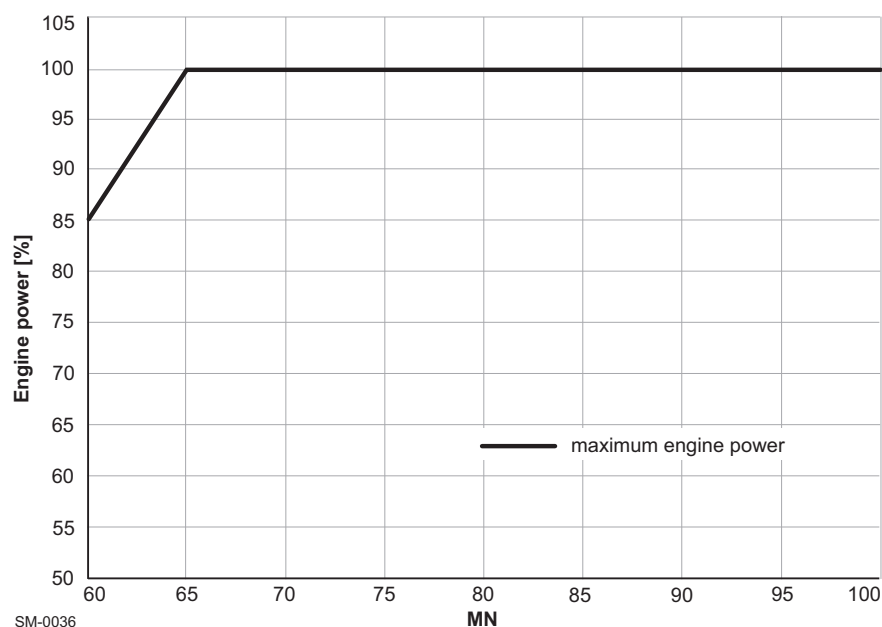
Figure 4-16 Maximum achievable power
