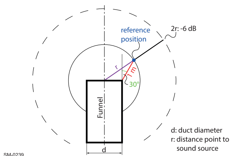
Figure 7-8 Exhaust noise reference point
