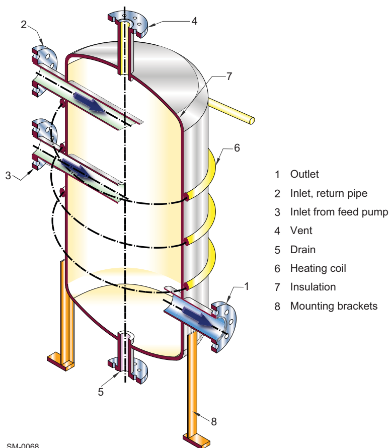
Figure 4-38 Mixing unit
