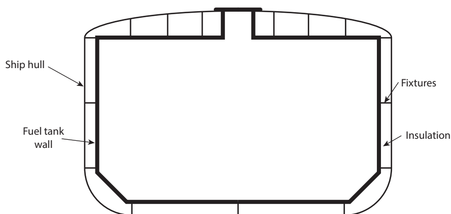
Figure 4-17 Section view of an integrated membrane tank
