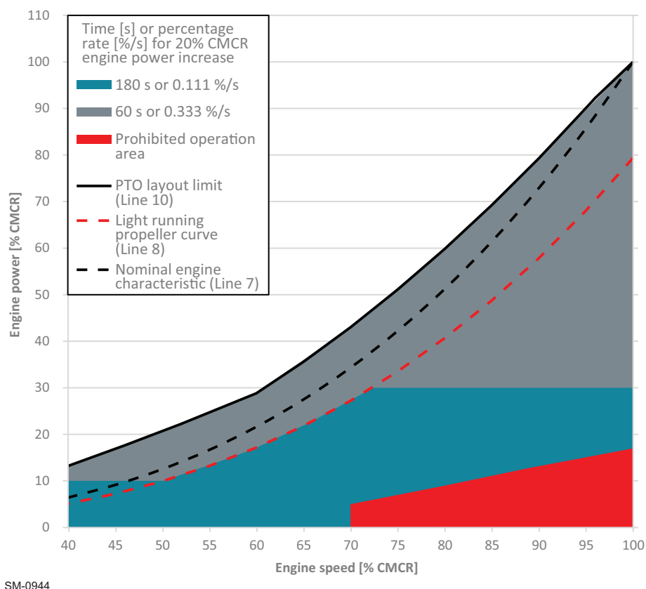
Figure 4-58 Maximum power increase rate for PTO application in gas mode
