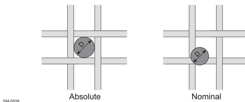
Figure 4-39 Mesh size difference between absolute and nominal
