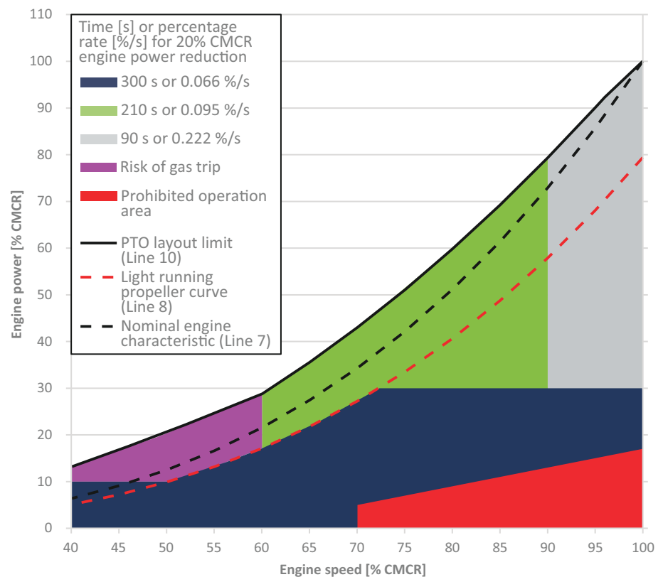
Figure 4-59 Maximum power decrease rate for PTO application in gas mode
