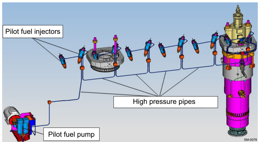
Figure 4-36 Pilot fuel high-pressure system
