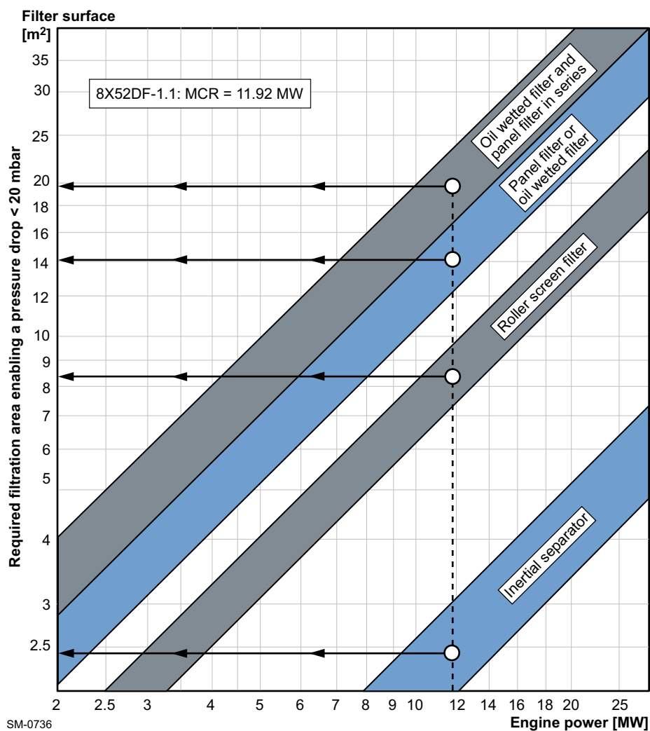
Figure 4-52 Air filter size (example for 8-cyl. engine)
