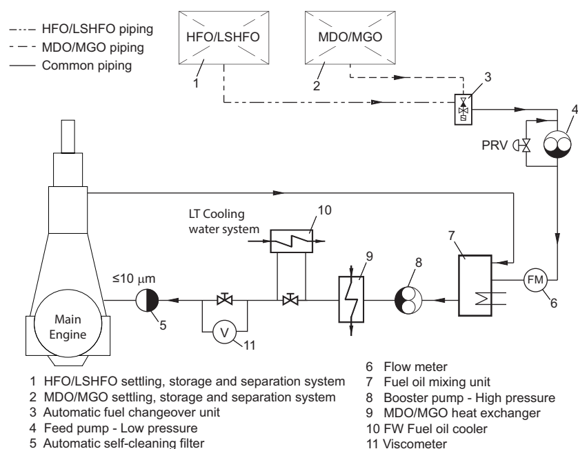
Figure 4-41 Fuel oil filter arrangement 'B'
