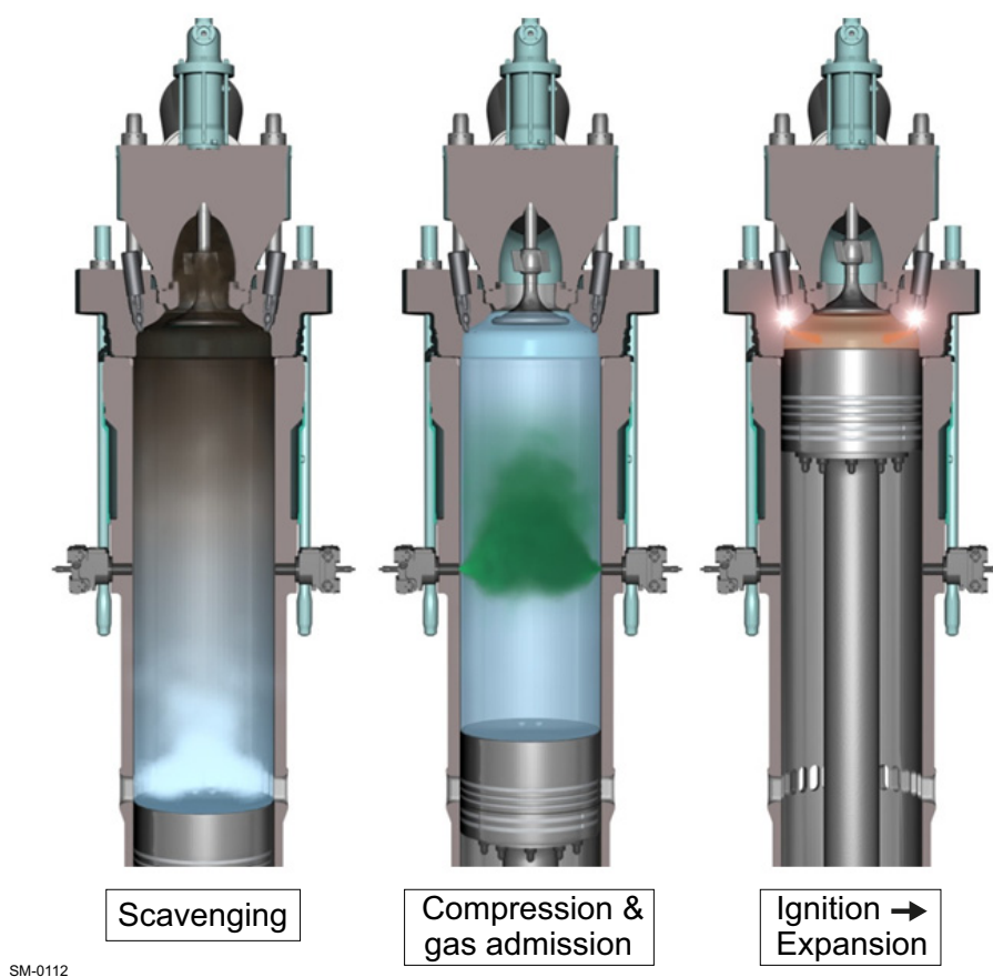
Figure 4-14 Lean burn with pilot ignition
