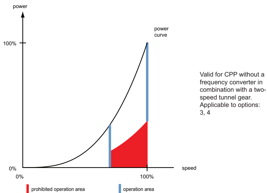
Figure 4-57 CPP with two fixed operation speeds without frequency converter
