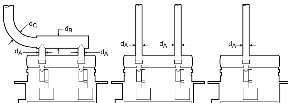
Figure 4-49 Determination of exhaust pipe diameter
