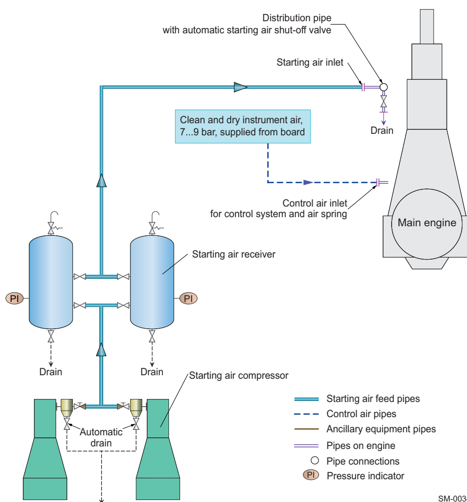
Figure 4-44 Air supply system
