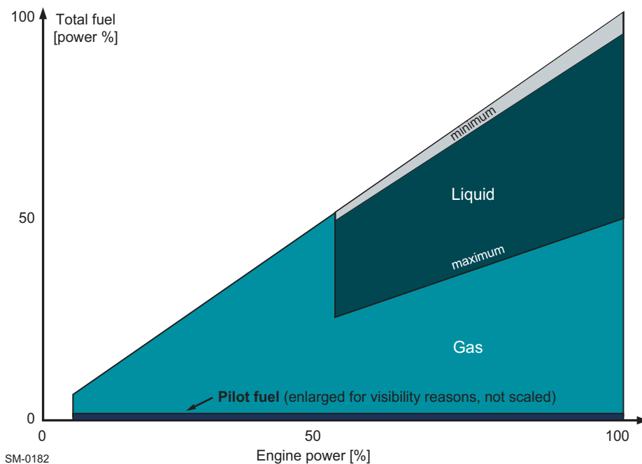
Figure 1-6 Fuel sharing mode — energy amount of different ratios of fuel
