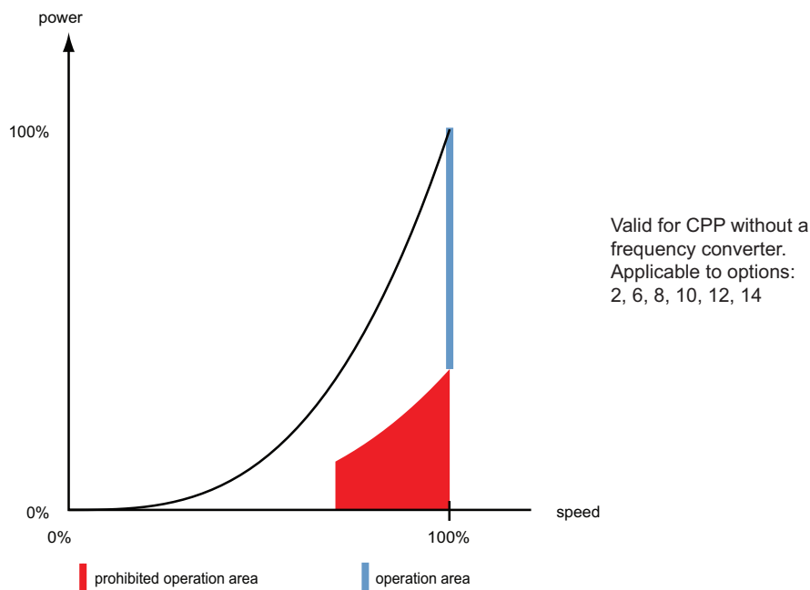
Figure 4-56 CPP in constant speed operation without frequency converter
