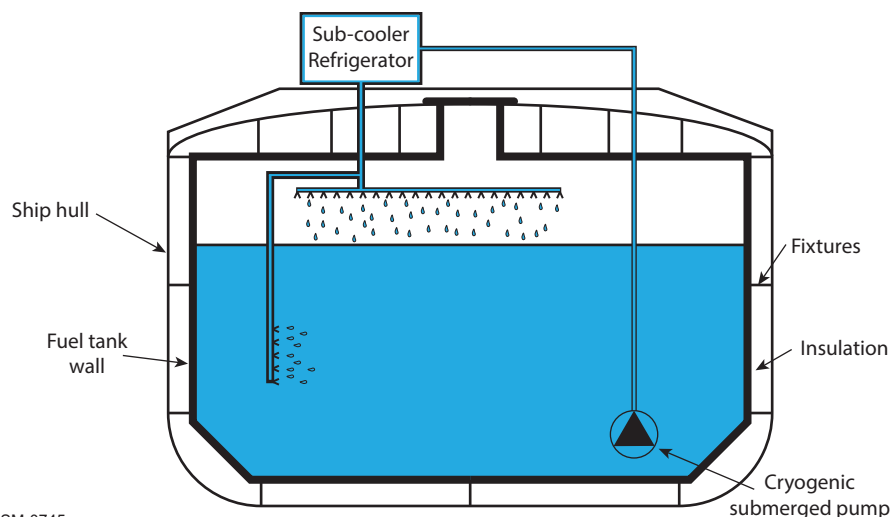
Figure 4-25 An LNG sub-cooler within an integrated tank
