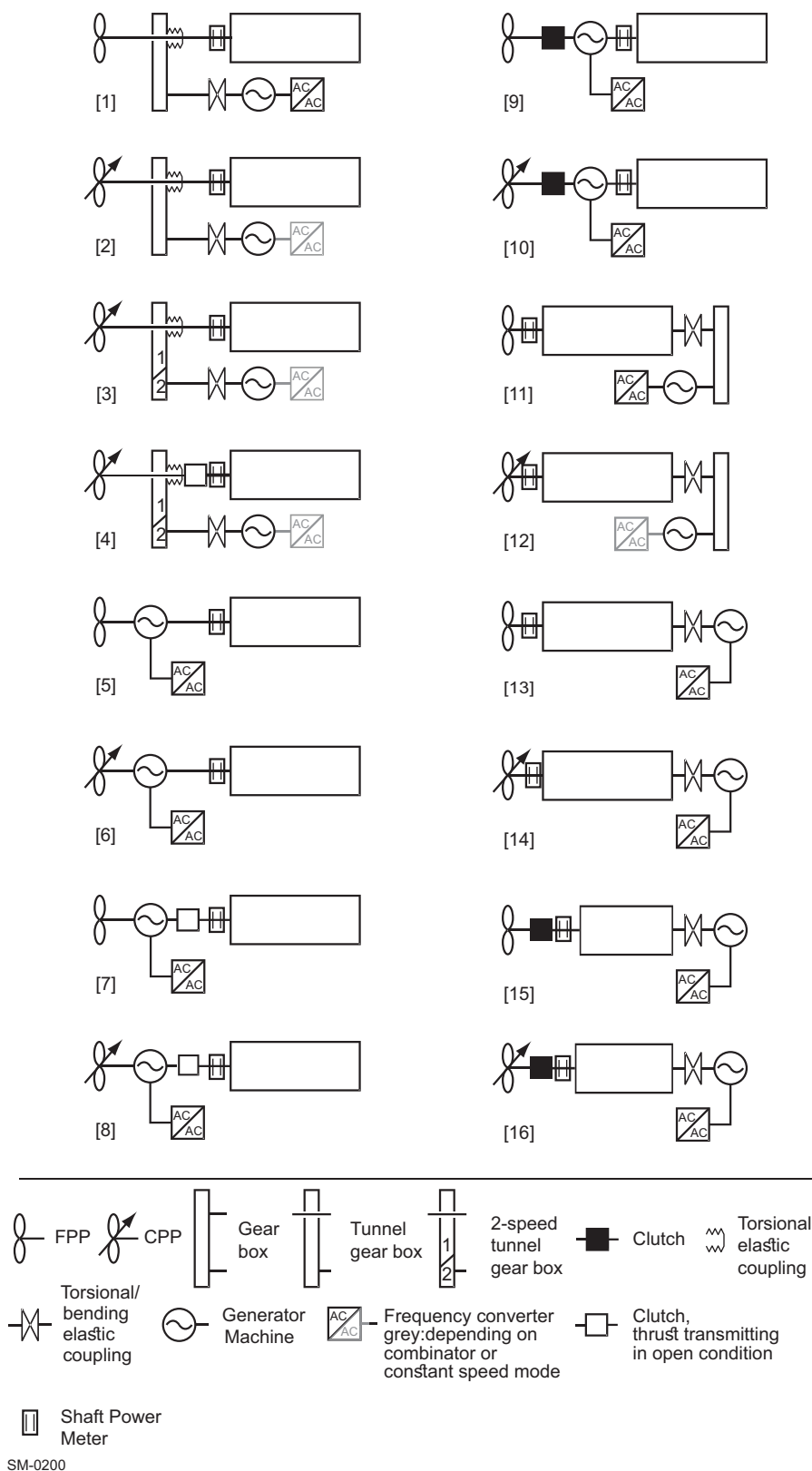
Figure 4-53 Arrangements for PTO, PTI, PTH
