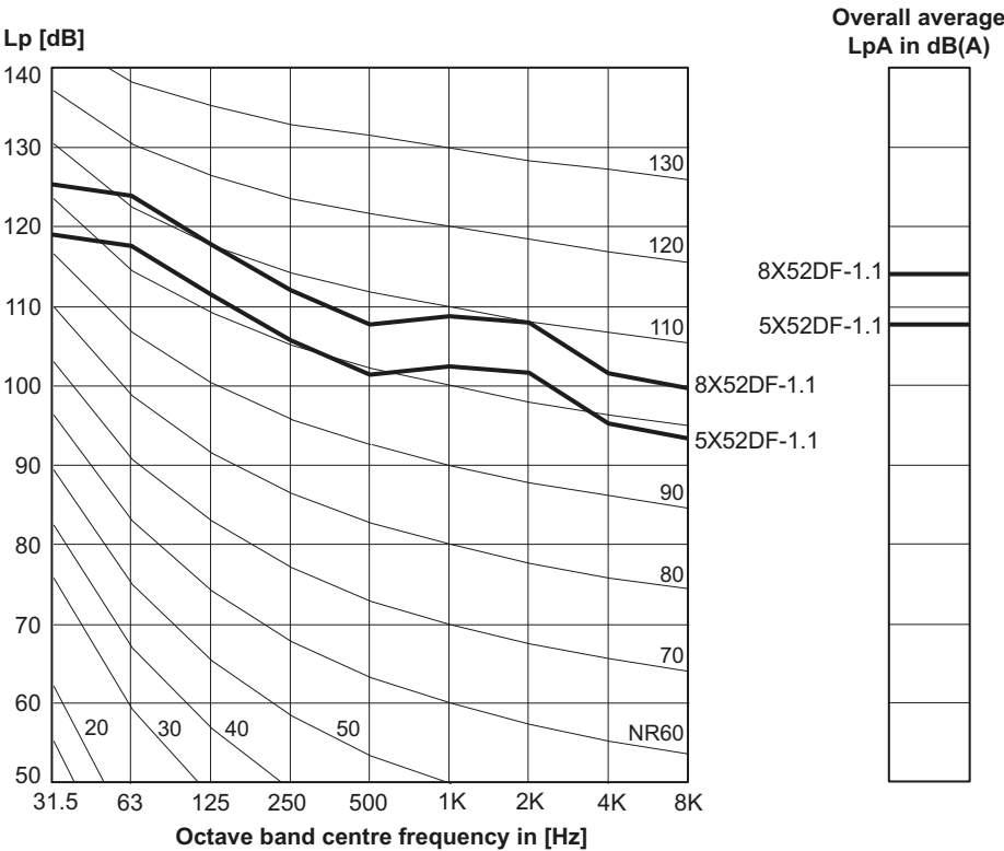
Figure 7-9 Sound pressure level at funnel top of exhaust gas system
