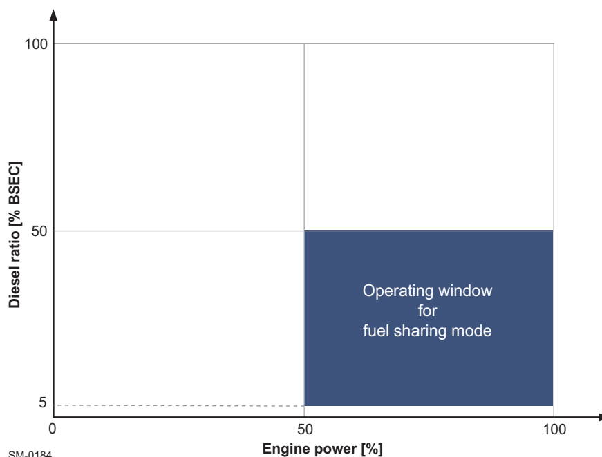
Figure 1-5 Fuel sharing mode — available operating window
