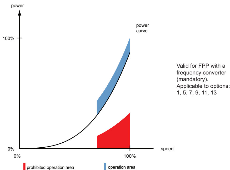
Figure 4-54 FPP with mandatory frequency converter
