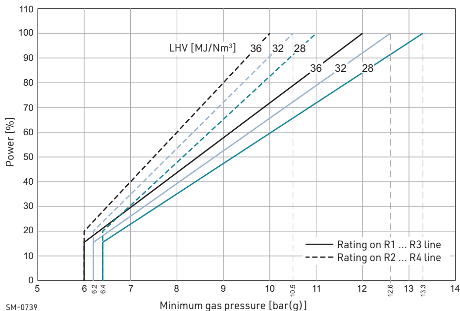
Figure 4-26 Design fuel gas supply pressure requirements
