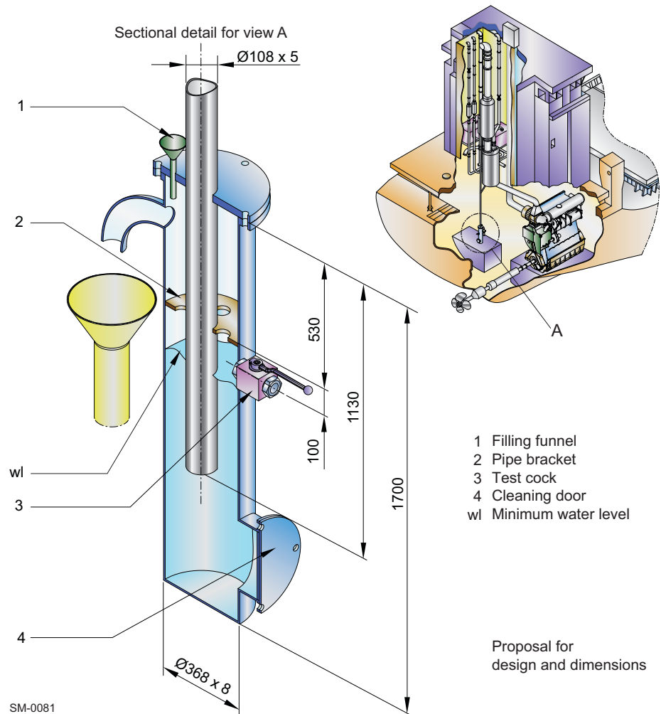
Figure 4-48 Arrangement of automatic water drain
