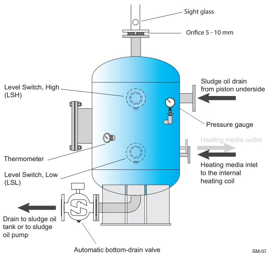
Figure 4-47 Design proposal of an automatically bottom-drained sludge oil trap
