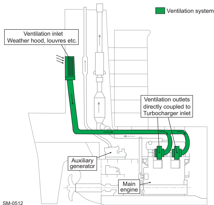
Figure 4-51 Ventilation system arrangement 2 — Direct engine ventilation system
