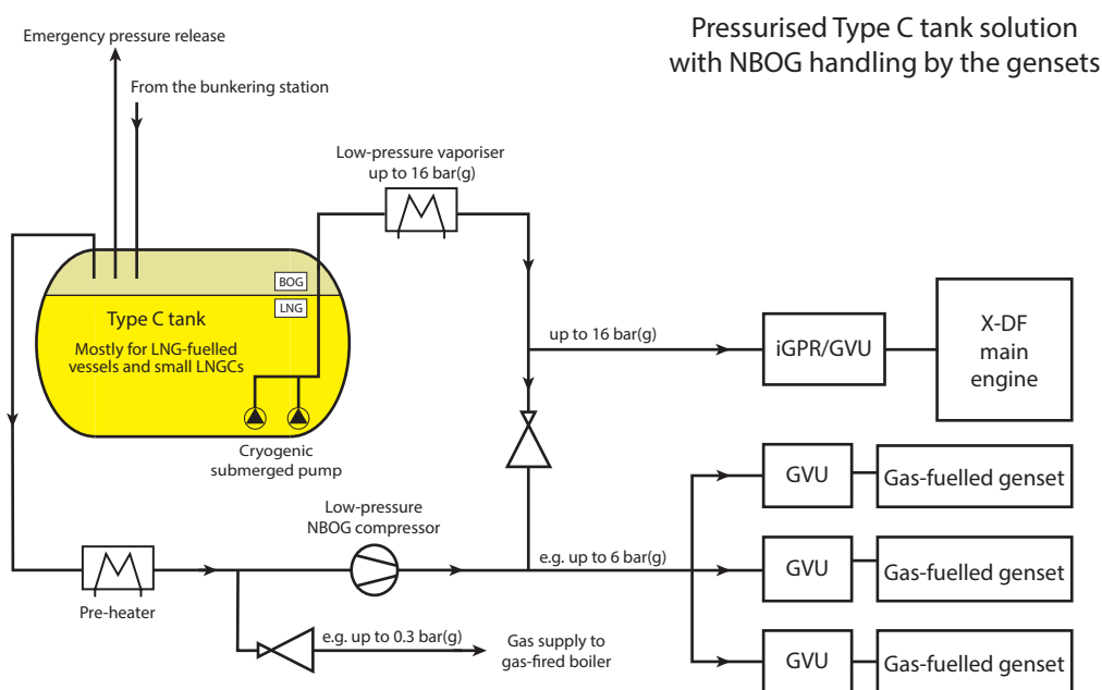
Figure 4-22 Pressurised Type C tank solution with NBOG handling by the gensets
