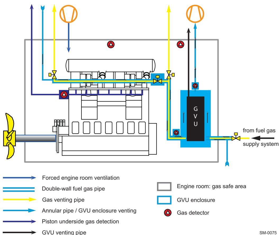
Figure 4-32 The GVU-ED™ from Wärtsilä
