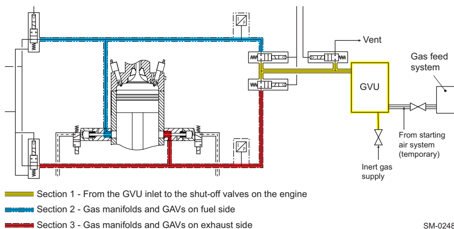
Figure 4-34 Gas leak test sequence (engines with GUV)
