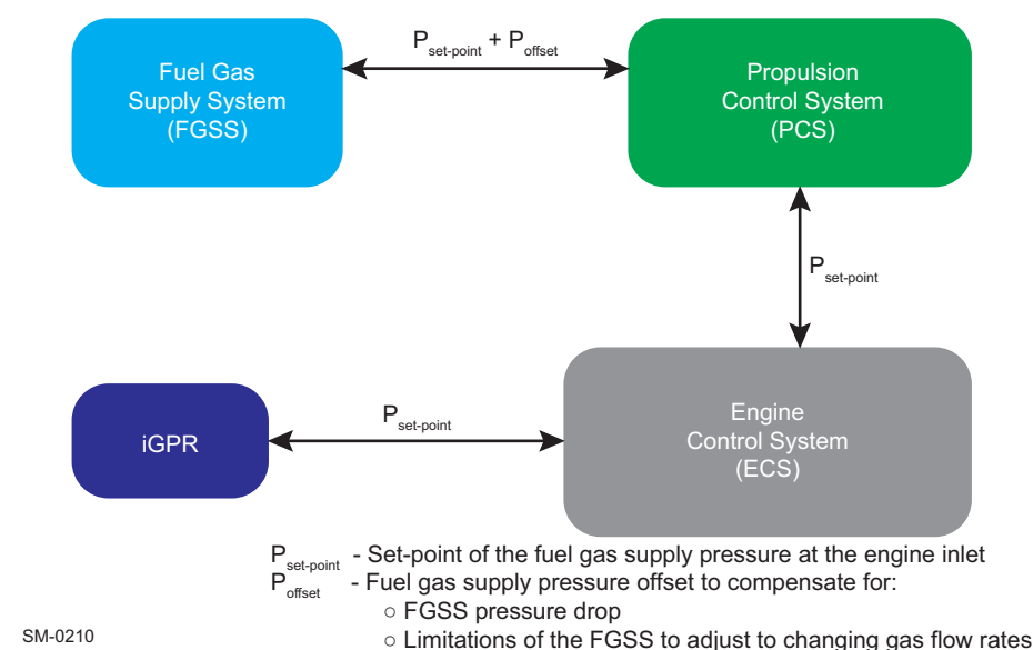
Figure 4-27 Fuel gas supply pressure control at the engine inlet (engines with iGPR)
