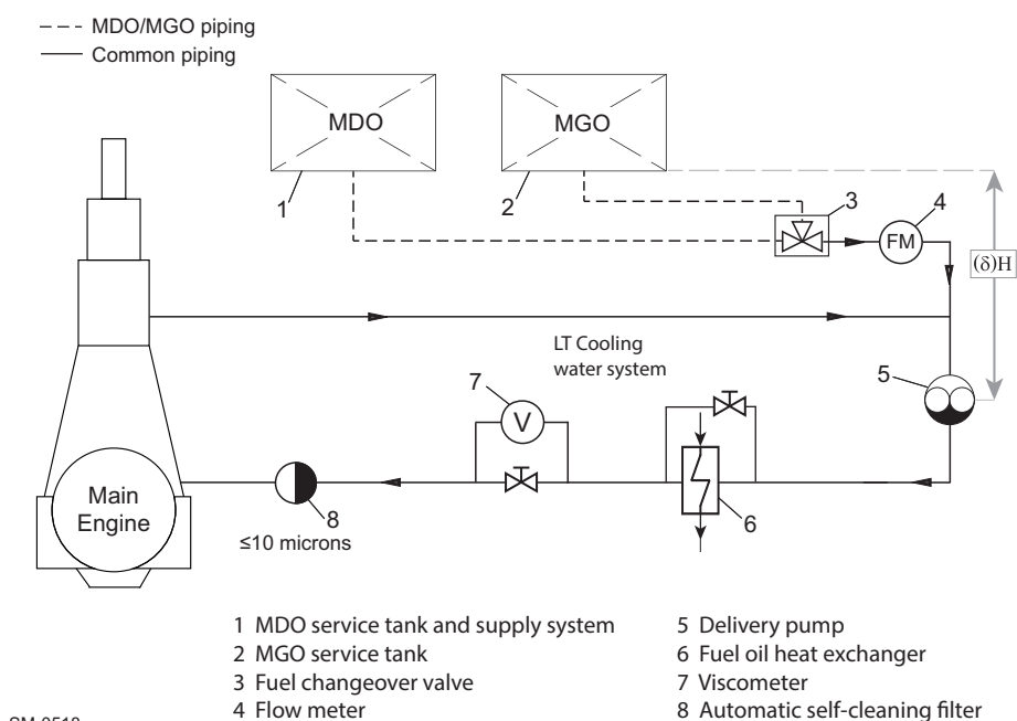
Figure 4-42 Fuel oil system — Arrangement with only MDO/MGO or MGO
