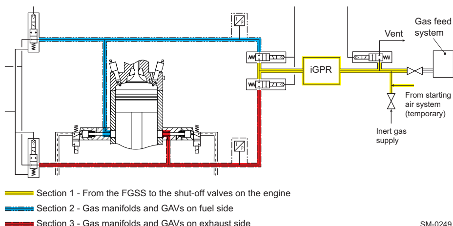
Figure 4-33 Gas leak test sequence (engines with iGPR)
