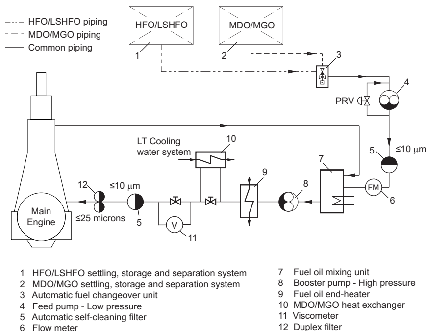
Figure 4-37 Fuel oil system
