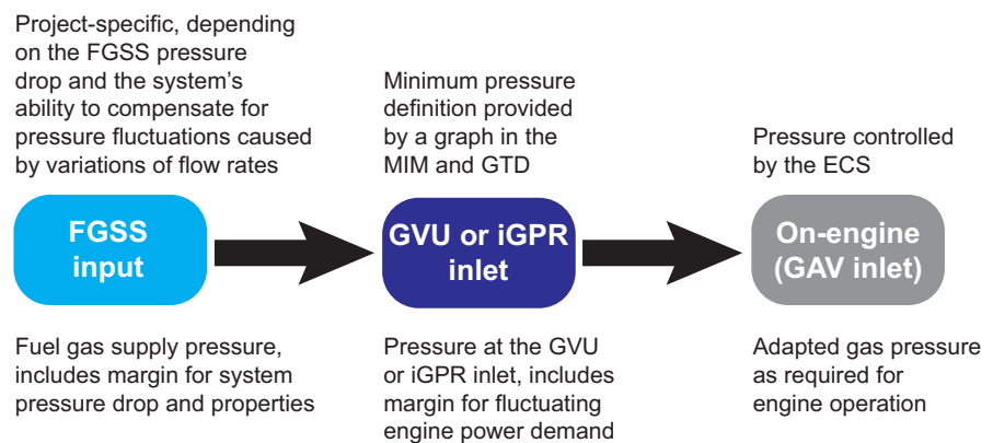
Figure 4-29 Fuel gas pressure level definitions
