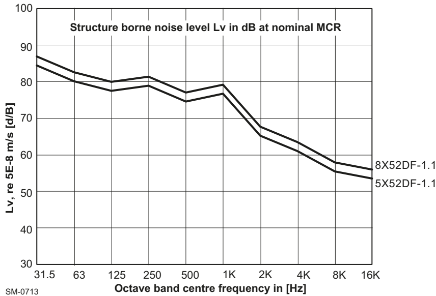
Figure 7-10 Structure-borne noise level at engine feet vertical
