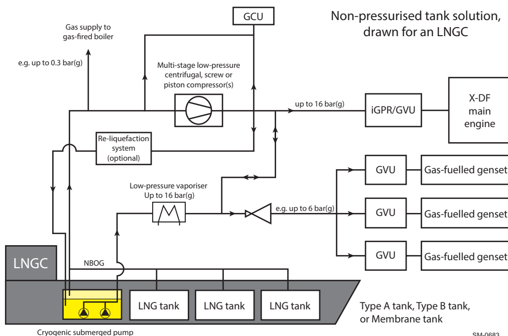
Figure 4-24 Non-pressurised tank solution, drawn for an LNGC
