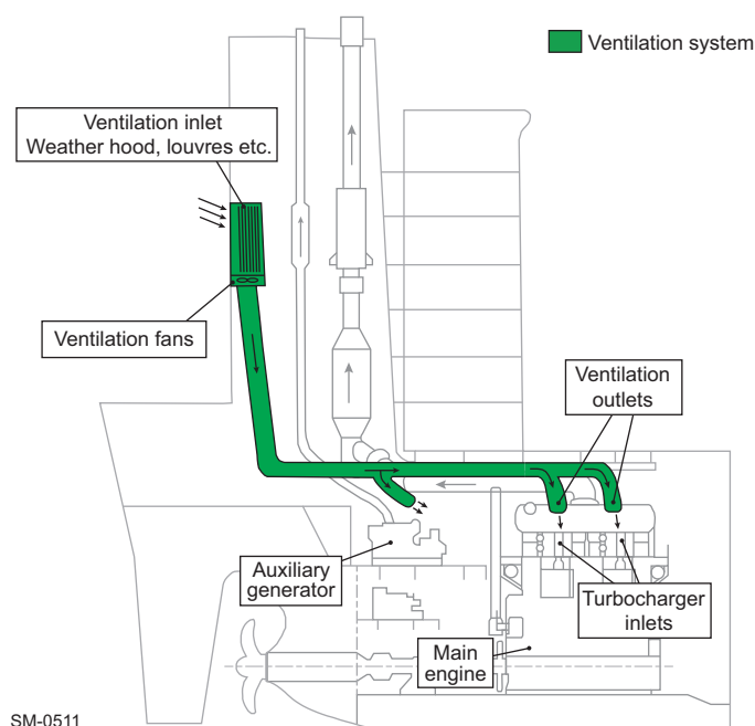
Figure 4-50 Ventilation system arrangement 1 — Engine room ventilation system
