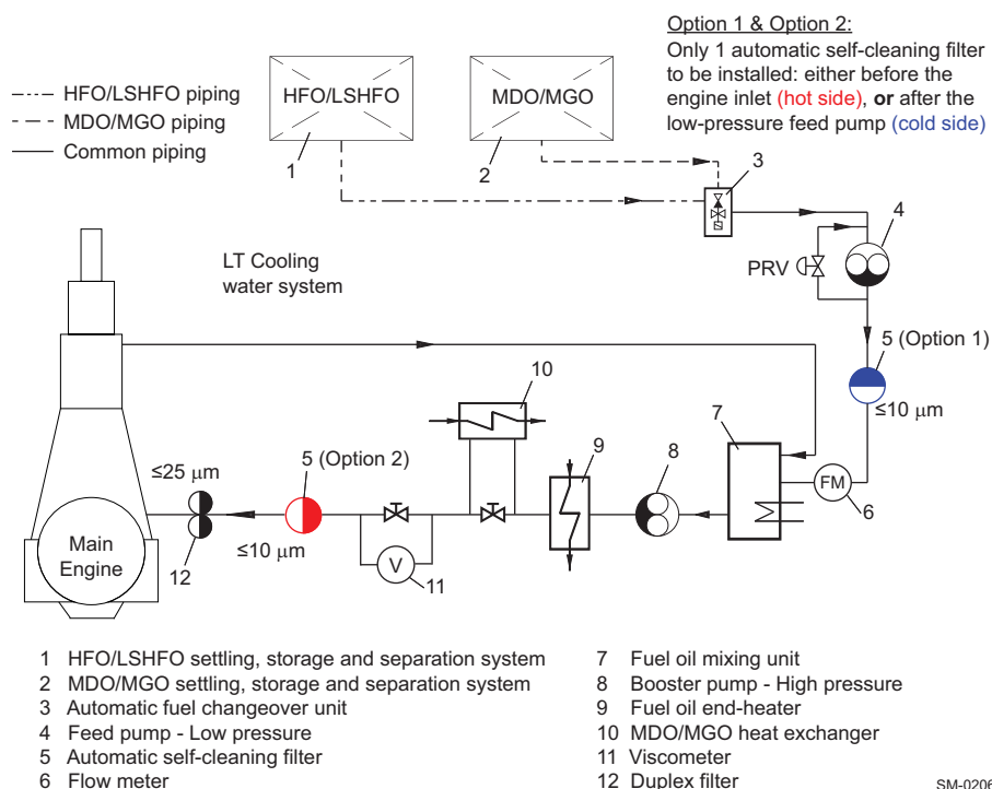
Figure 4-40 Fuel oil filter arrangement 'A'
