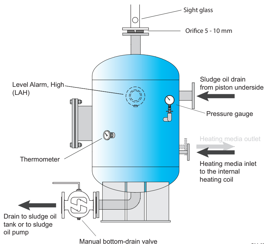
Figure 4-46 Design proposal of a manually bottom-drained sludge oil trap
