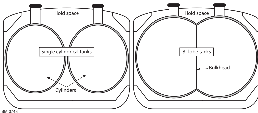
Figure 4-20 Section view of different free-standing Type C tanks installed below the deck
