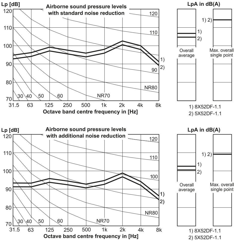
Figure 7-7 Sound pressure level at 1 m distance from engine
