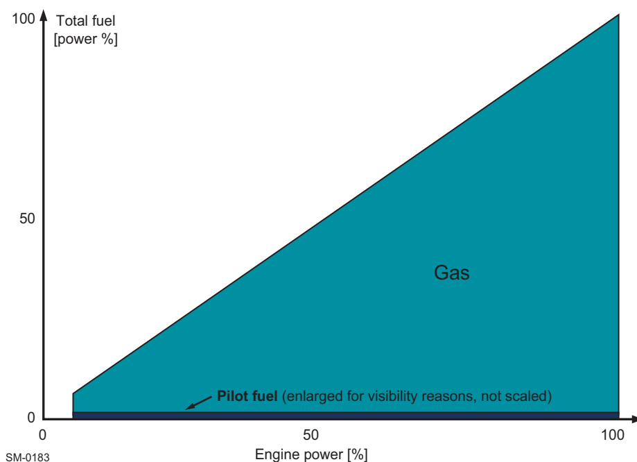
Figure 1-3 Gas mode operation
