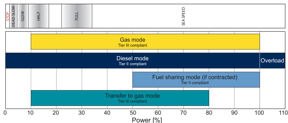
Figure 1-2 Operating modes of the X-DF engine
