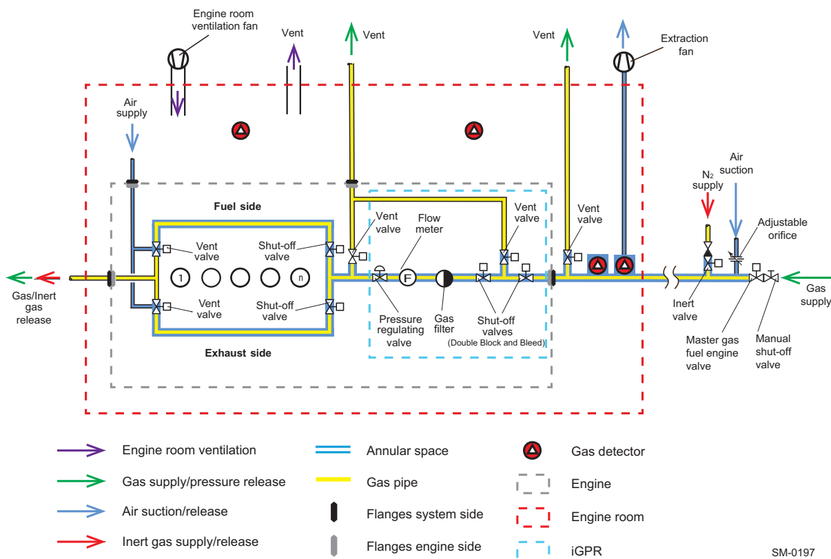
Figure 4-30 Fuel gas supply system with the iGPR
