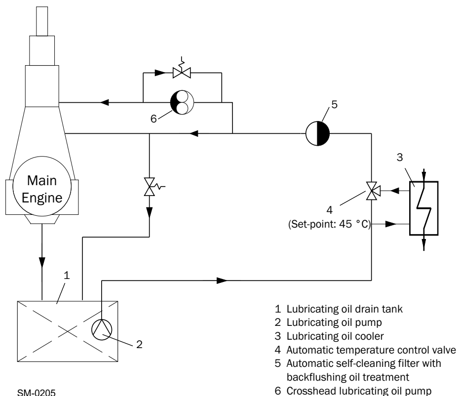
Figure 4-23 LO system
