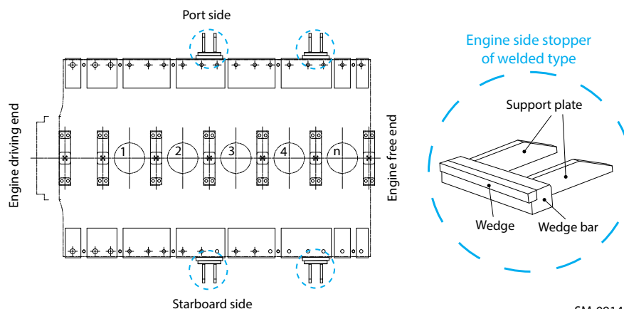
Figure 3-6 Welded type
