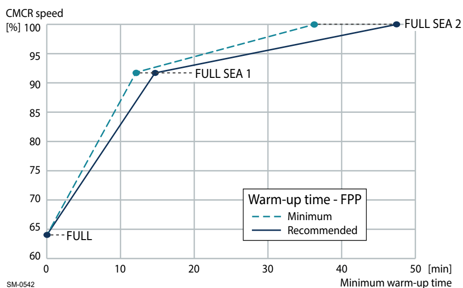
Figure 5-6 Full sea load steps in FPP load-up program
