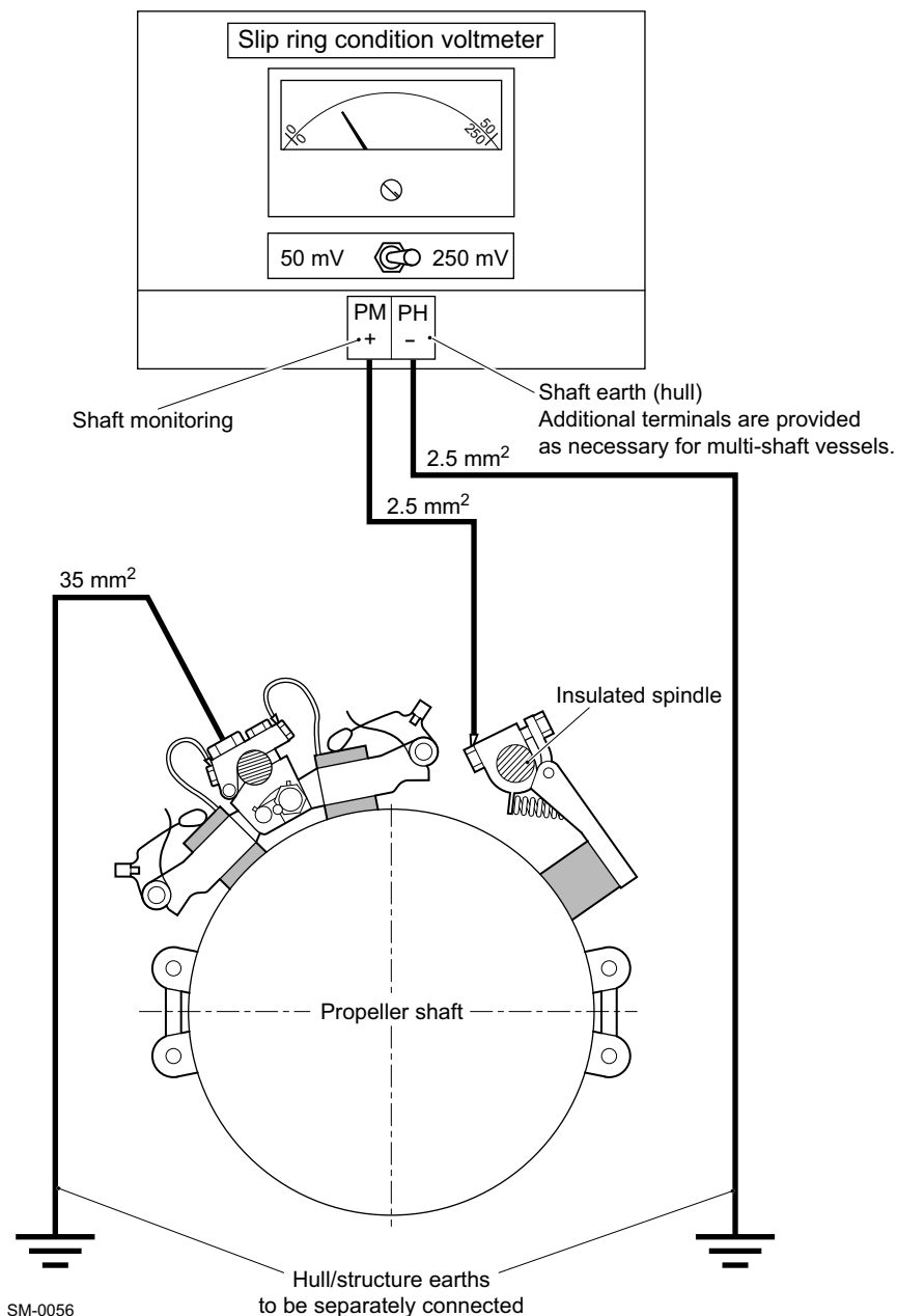
Figure 3-9 Typical shaft earthing with condition monitoring facility
