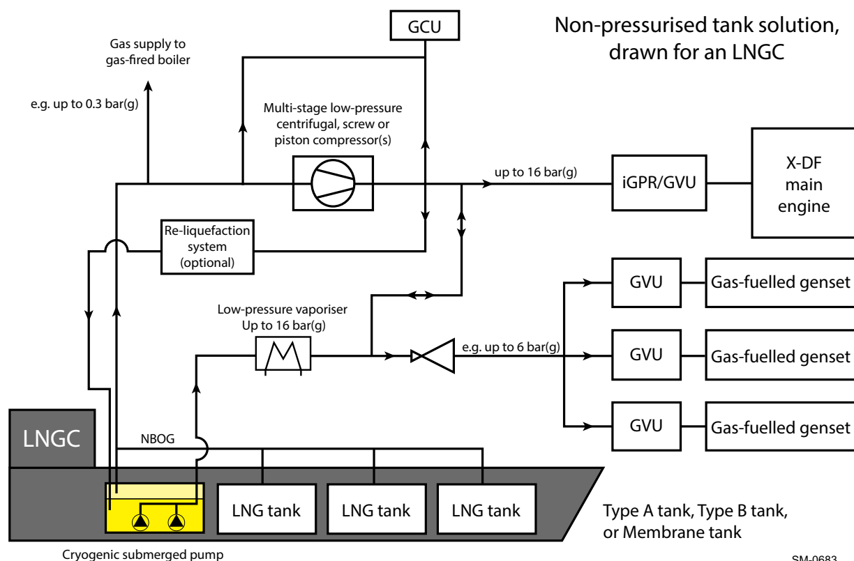
Figure 4-40 Non-pressurised tank solution, drawn for an LNGC
