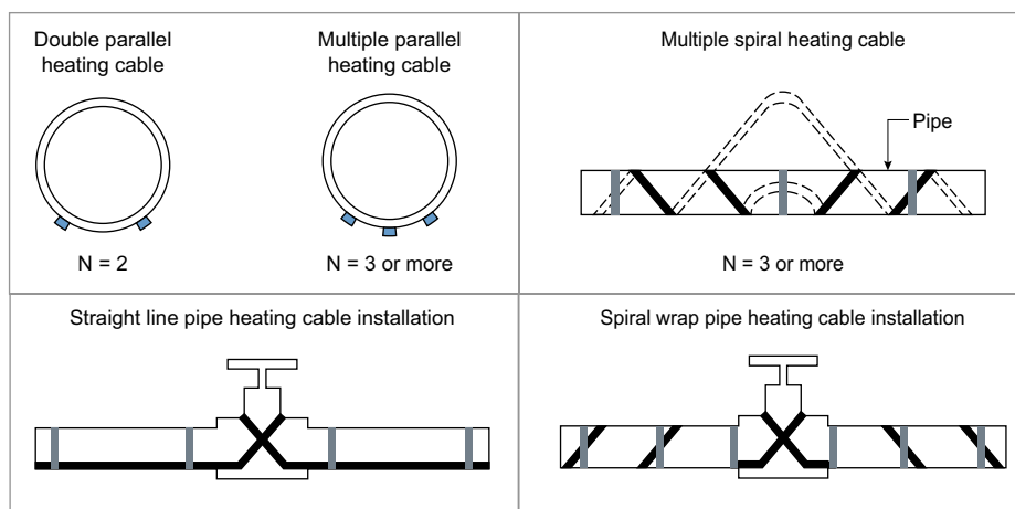
Figure 4-26 Trace heating cable arrangement
