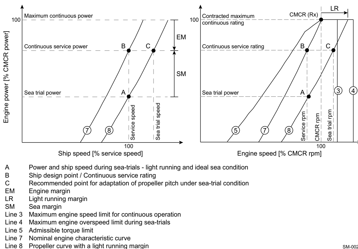
Figure 2-2 Propeller curves and operational points
