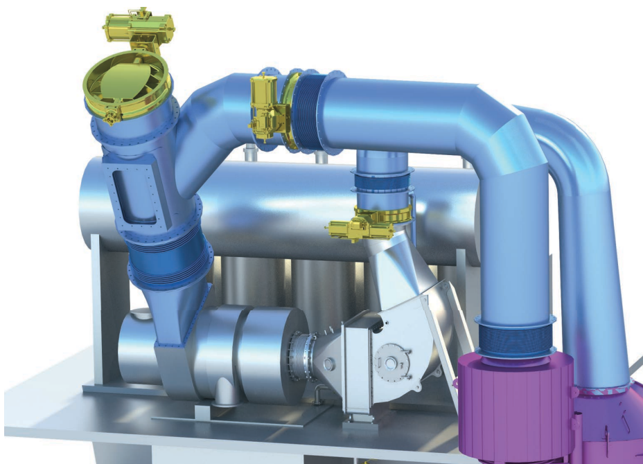
Figure 4-11 Example of an exhaust gas piping arrangement with one turbocharger
