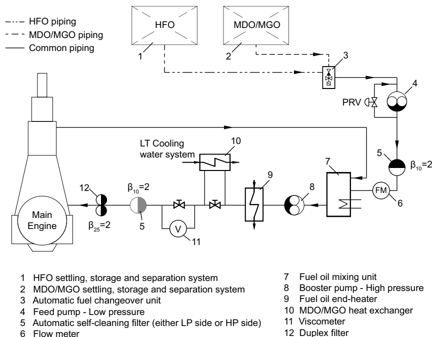
Figure 4-53 Fuel oil system
