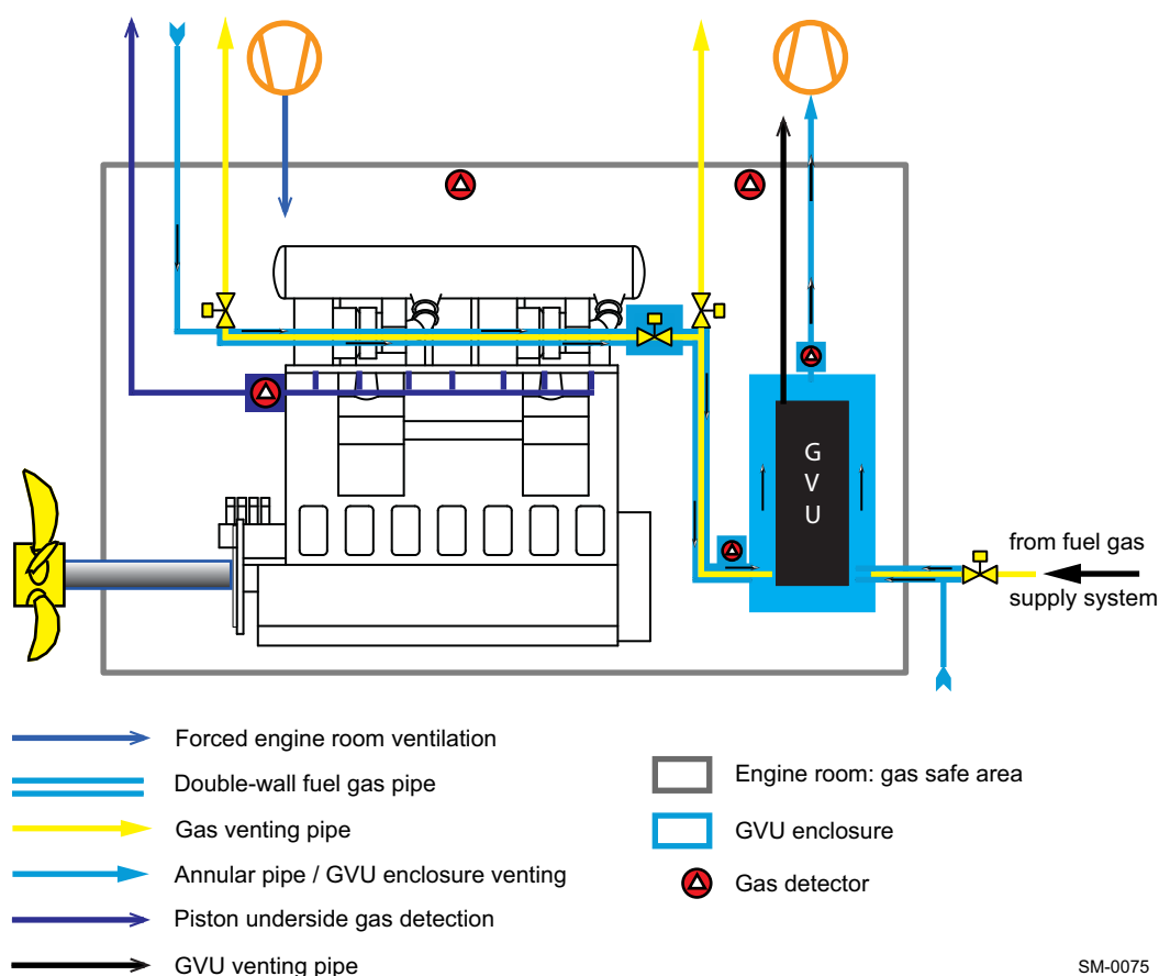
Figure 4-48 The GVU-ED™ from Wärtsilä
