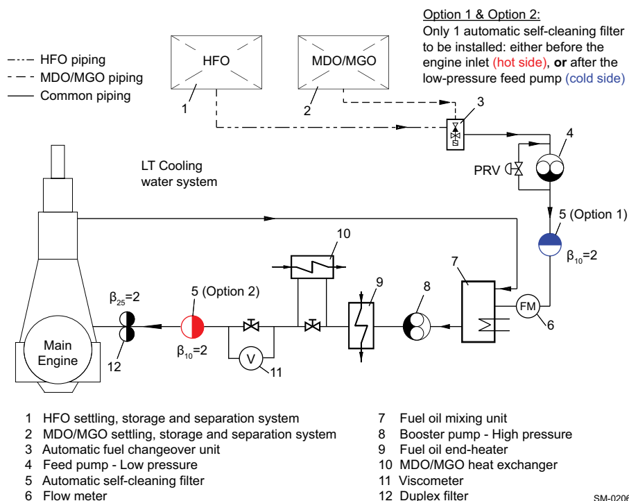
Figure 4-57 Fuel oil filter arrangement 'A'
