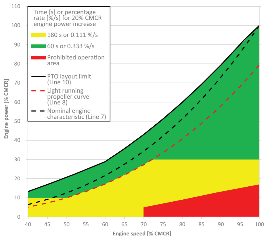
Figure 4-74 Maximum power increase rate for PTO application in gas mode
