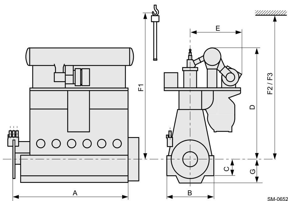
Figure 3-1 Engine dimensions
