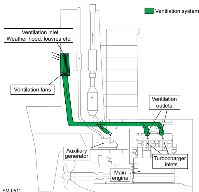
Figure 4-66 Ventilation system arrangement 1: Engine room ventilation system
