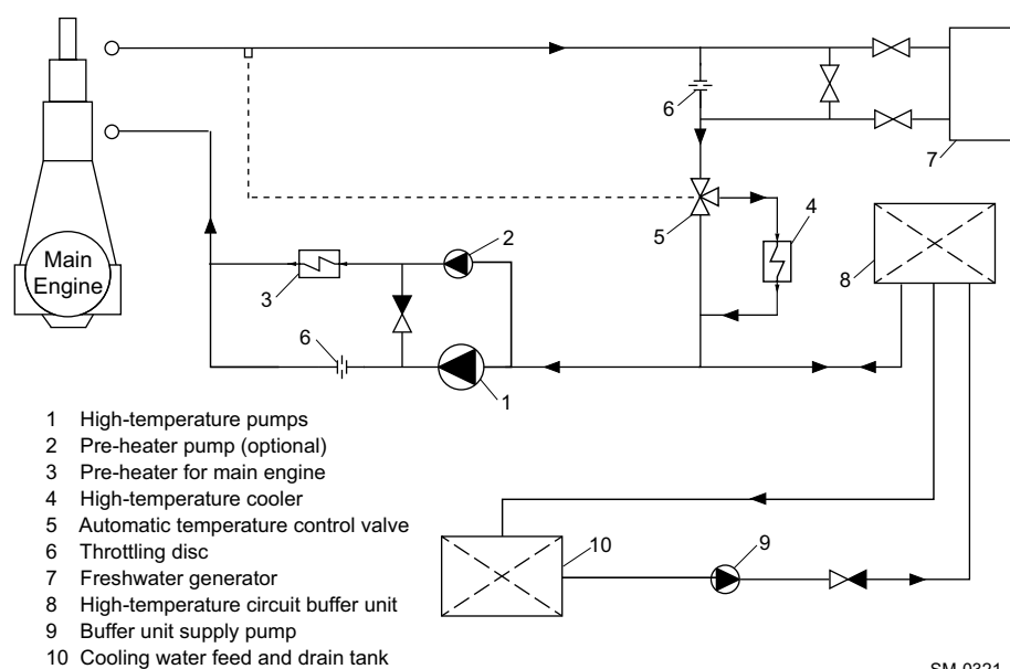
Figure 4-21 HT cooling water circuit
