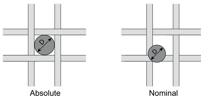
Figure 4-56 Mesh size difference between absolute and nominal
