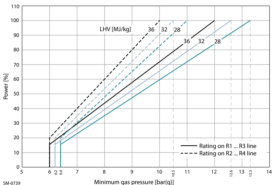
Figure 4-42 Design fuel gas supply pressure requirements
