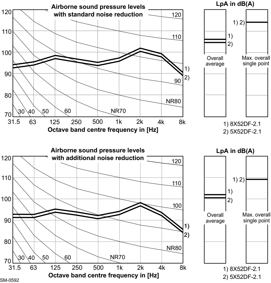
Figure 7-4 Sound pressure level at 1 m distance from the engine
