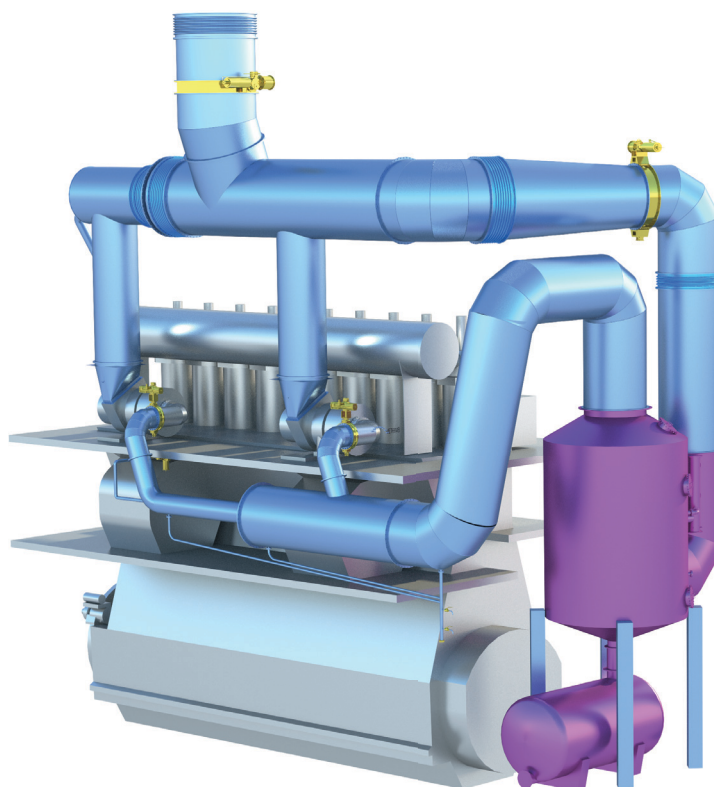
Figure 4-12 Example of an exhaust gas piping arrangement with two turbochargers
