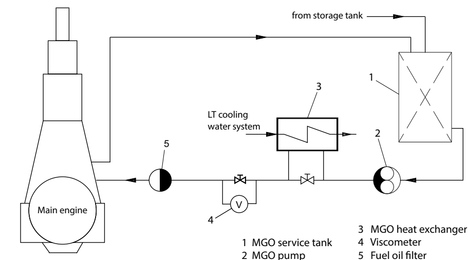
Figure 4-51 Pilot fuel oil system
