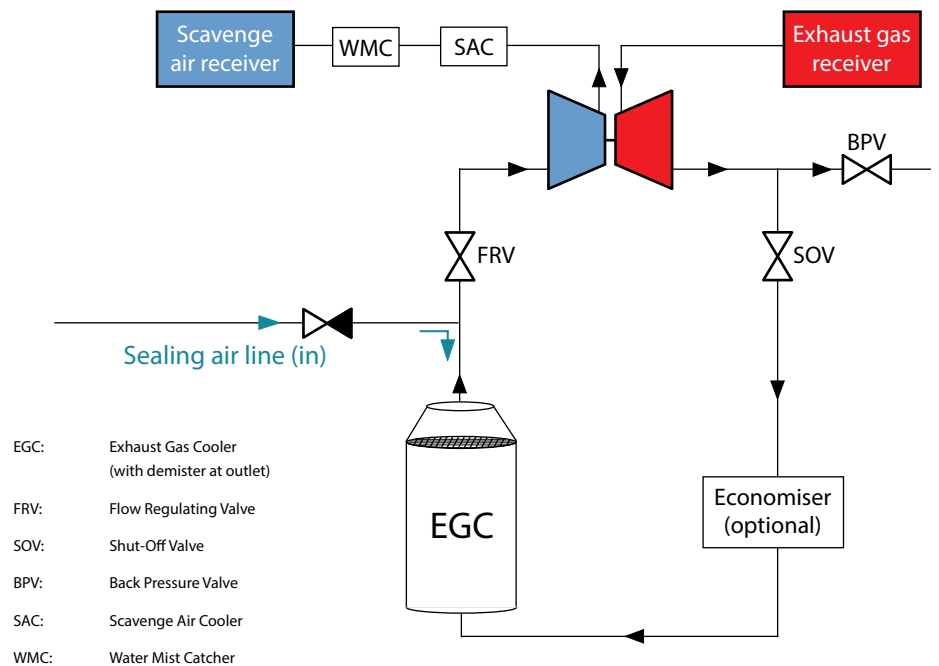
Figure 4-10 iCER exhaust gas system principle
