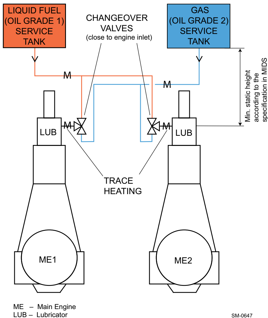
Figure 4-24 Dual cylinder LO installation, enabling independent gas and liquid fuel (max. 0.5% m/m sulphur) operation with a manual changeover valve
