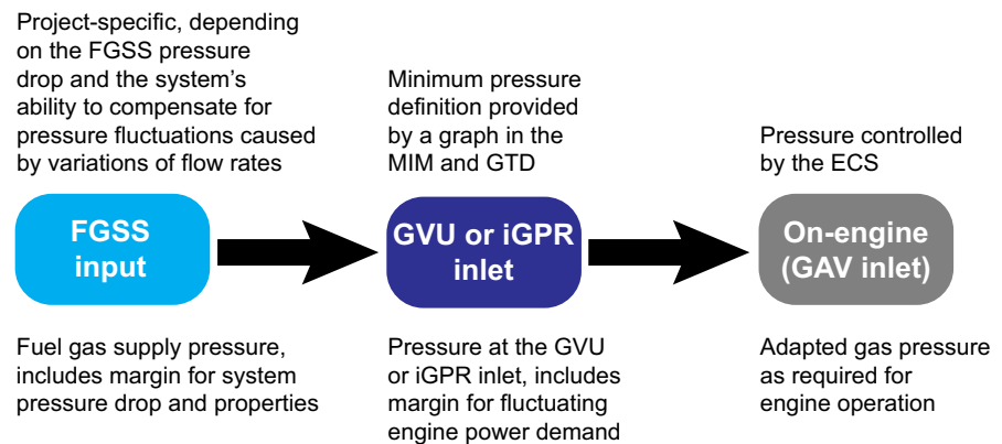
Figure 4-45 Fuel gas pressure level definitions
