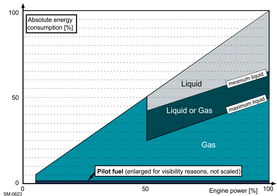
Figure 1-7 FSM: Energy amount of different ratios of fuel
