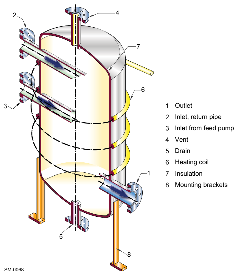
Figure 4-54 Mixing unit
