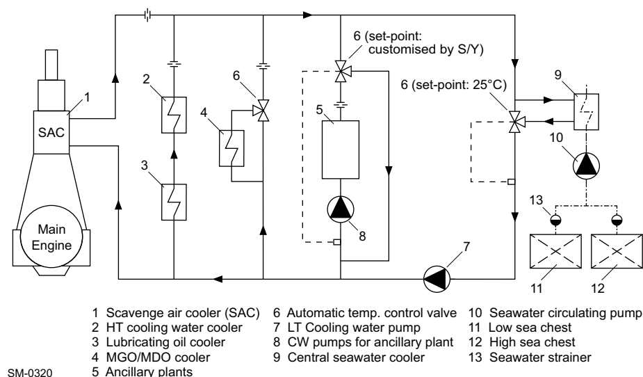
Figure 4-19 LT cooling water circuit: dual set-point temperatures
