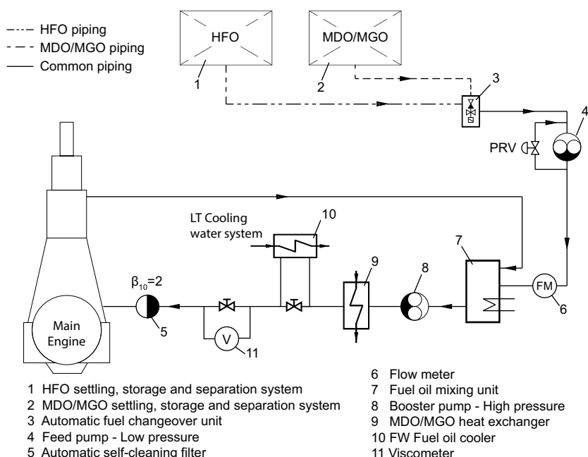
Figure 4-58 Fuel oil filter arrangement 'B'
