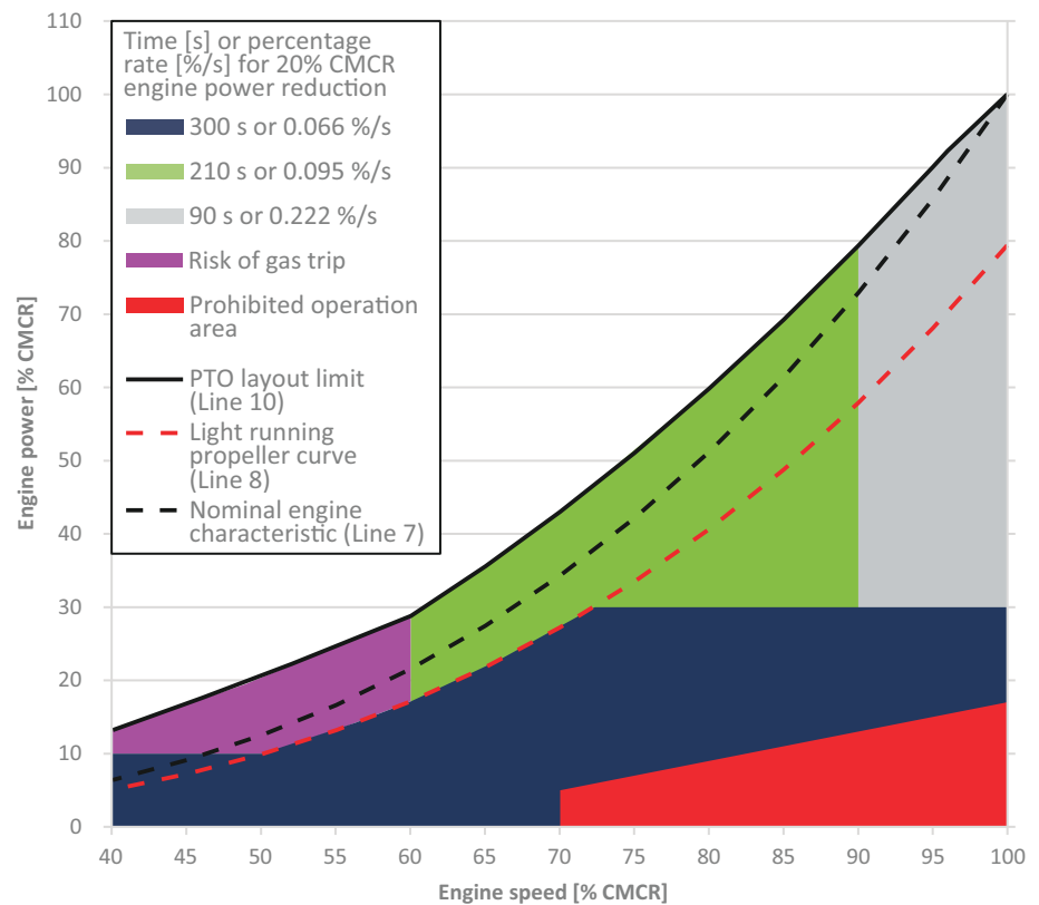
Figure 4-75 Maximum power decrease rate for PTO application in gas mode
