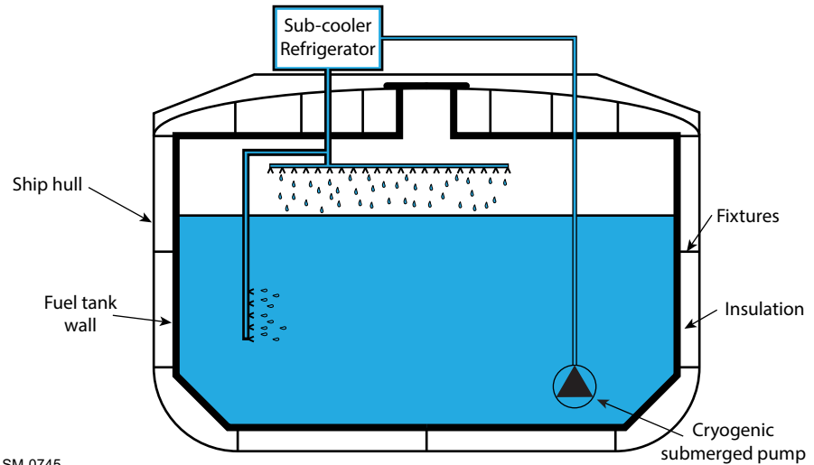
Figure 4-41 An LNG sub-cooler within an integrated tank
