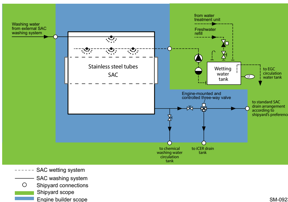
Figure 4-9 The SAC wetting system with the wetting water tank arrangement
