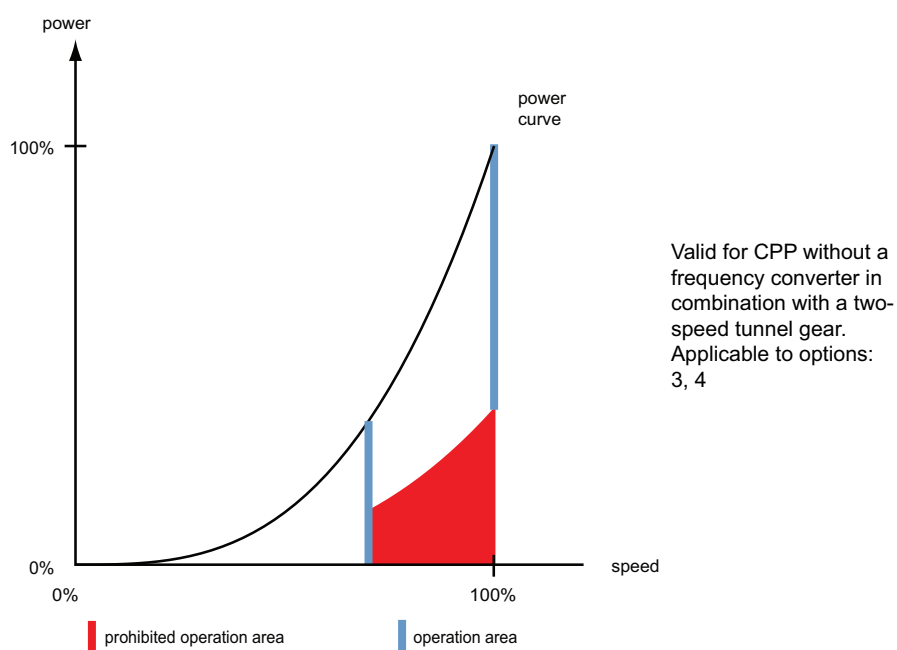
Figure 4-73 CPP with two fixed operation speeds without frequency converter
