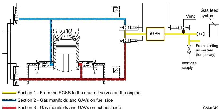
Figure 4-49 Gas leak test sequence (engines with iGPR)
