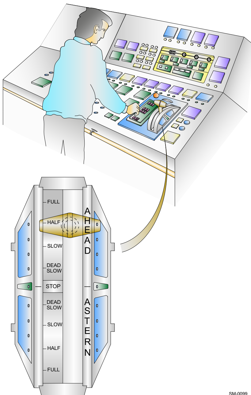
Figure 5-4 Propulsion control
