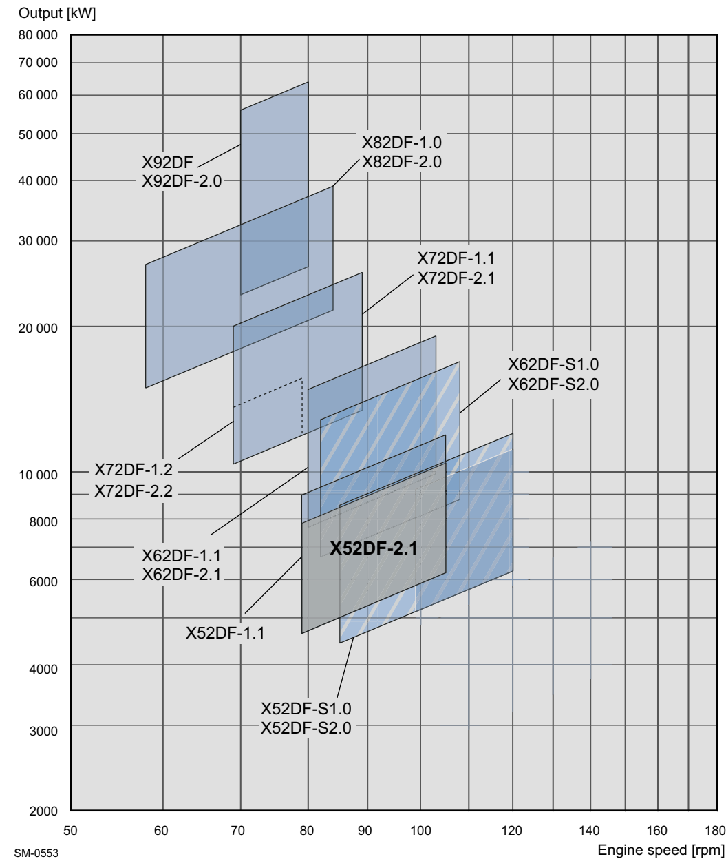
Figure 1-1 Power/speed range
