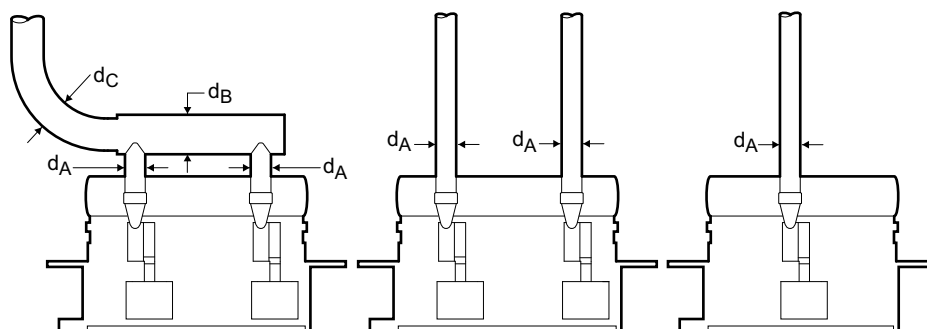
Figure 4-65 Determination of exhaust pipe diameter
