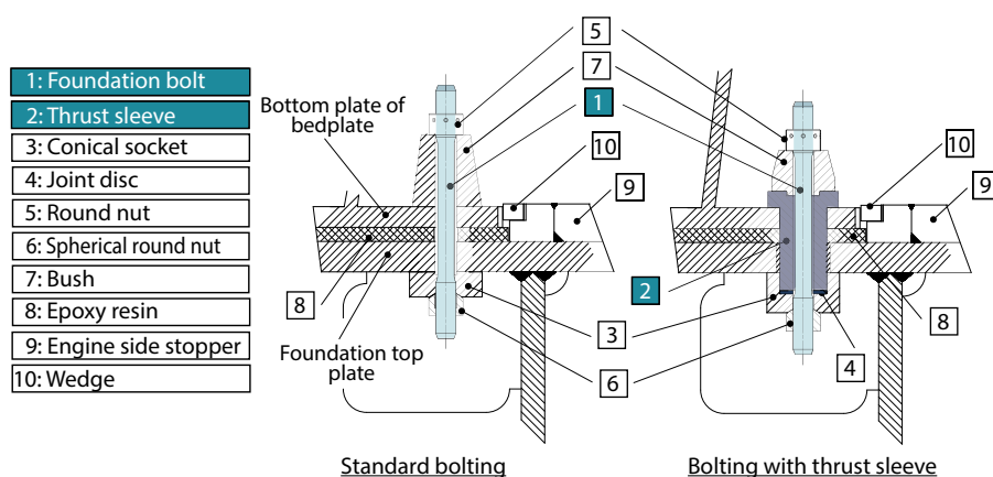
Figure 3-5 Foundation bolting
