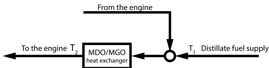
Figure 4-55 MDO/MGO heat exchanger
