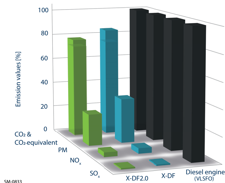
Figure 7-1 Emissions comparison between the X-DF2.0, X-DF and diesel engines
