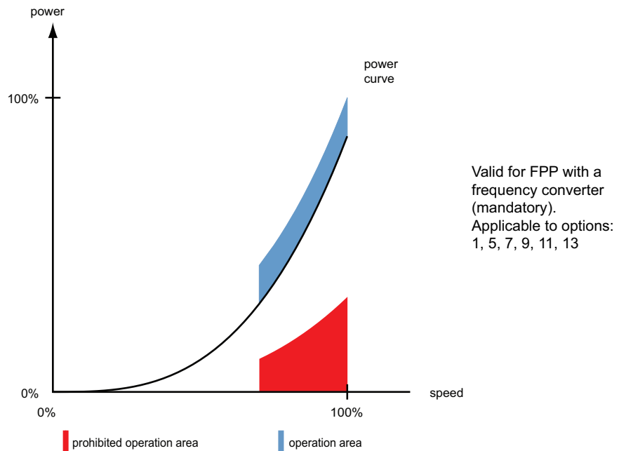
Figure 4-70 FPP with mandatory frequency converter
