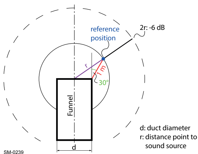
Figure 7-5 Exhaust noise reference point
