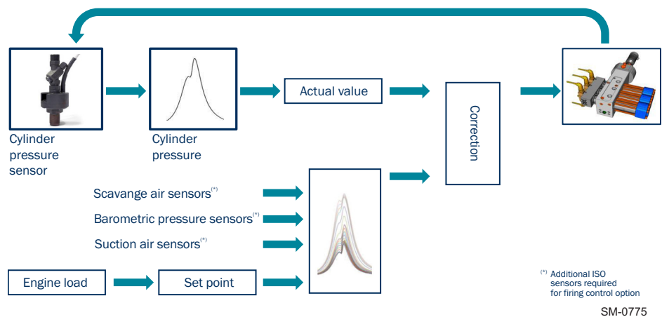
Figure 5-10 ICC system
