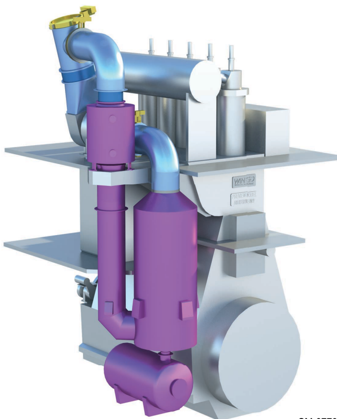
Figure 4-13 Example of an exhaust gas piping arrangement for the compact arrangement with one turbocharger
