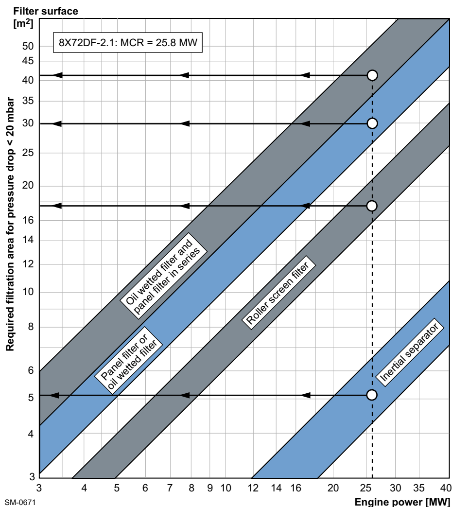
Figure 4-68 Air filter size (example for 8-cylinder engine)
