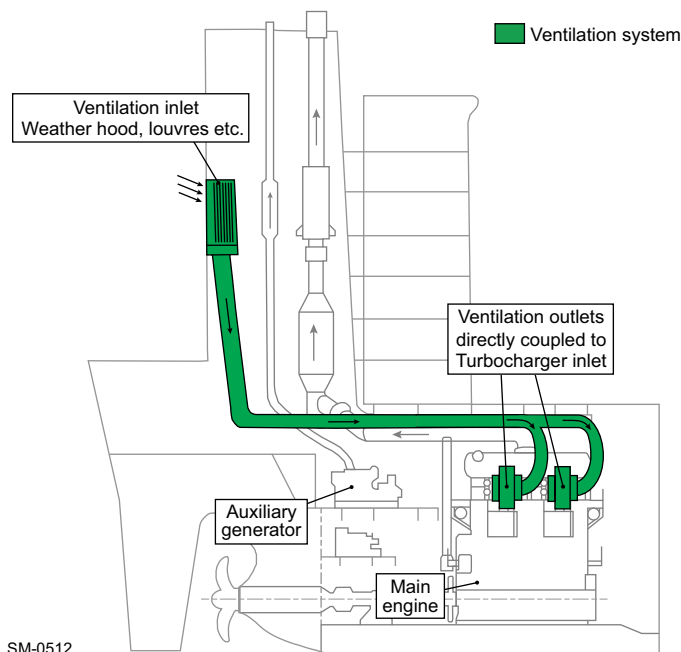
Figure 4-67 Ventilation system arrangement 2: Direct engine ventilation system
