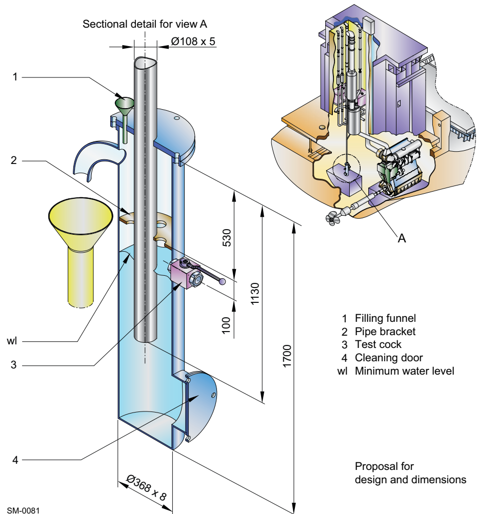
Figure 4-63 Arrangement of automatic water drain
