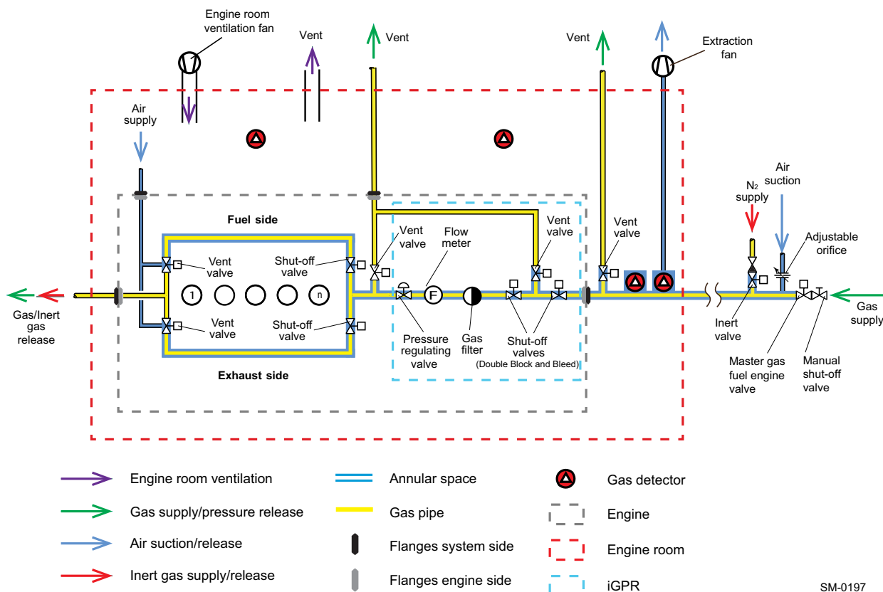
Figure 4-46 FGSS with the iGPR
