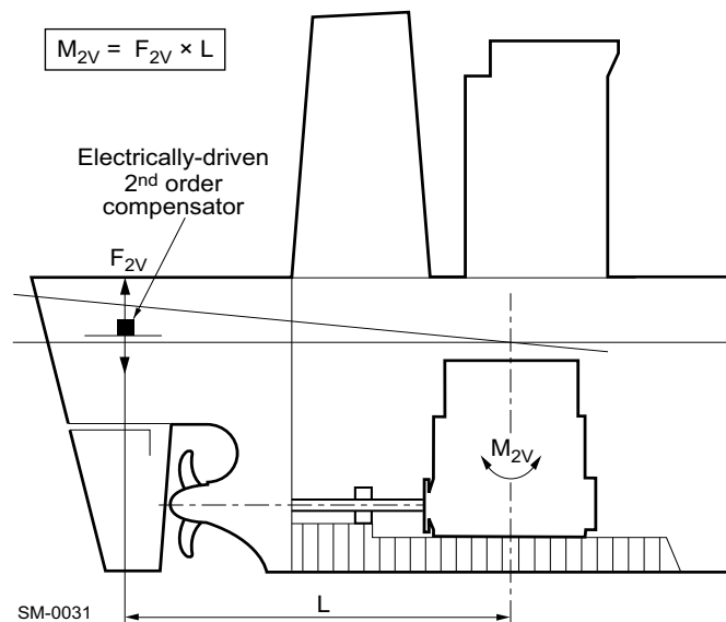
Figure 6-3 Location of an electrically-driven compensator
