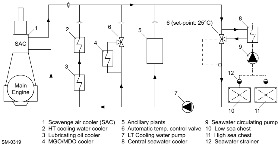
Figure 4-18 LT cooling water circuit: single set-point temperature
