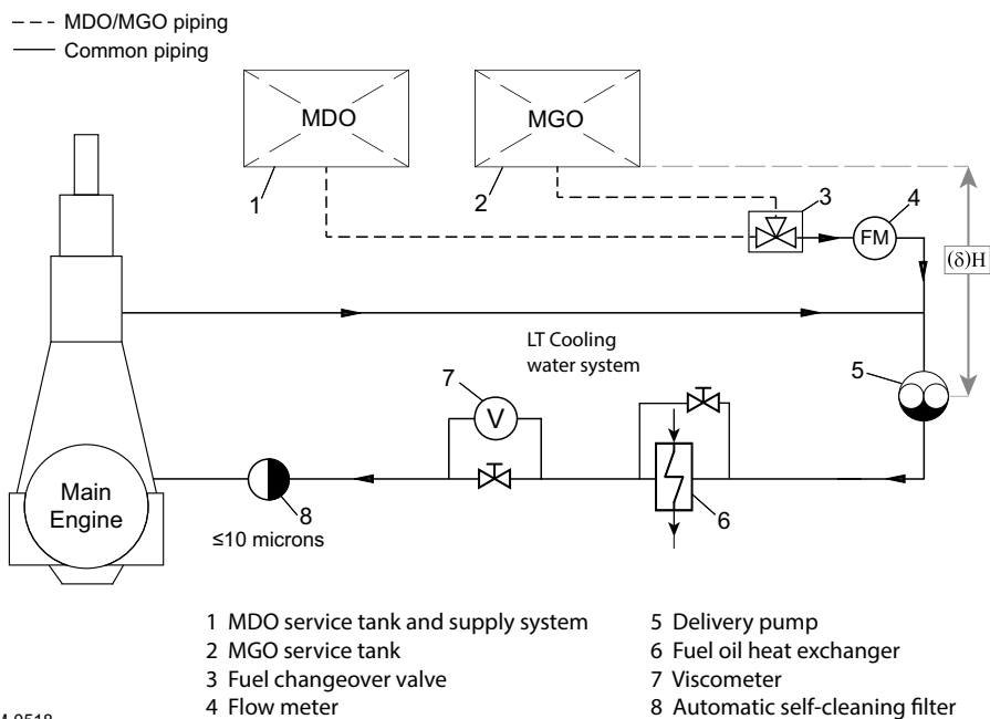
Figure 4-59 Fuel oil system — Arrangement with only MDO/MGO or MGO
