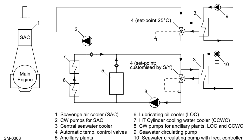
Figure 4-20 Separate SAC and LT cooling circuits
