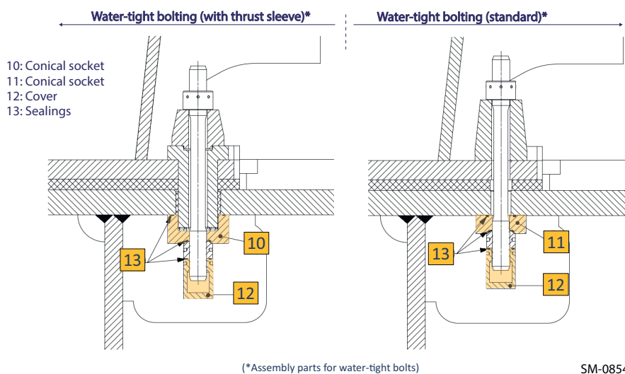
Figure 3-7 Proposed designs for water-tight bolting
