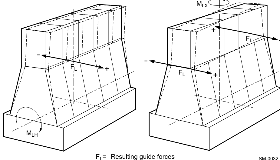
Figure 6-5 Lateral vibration: X-type and H-type
