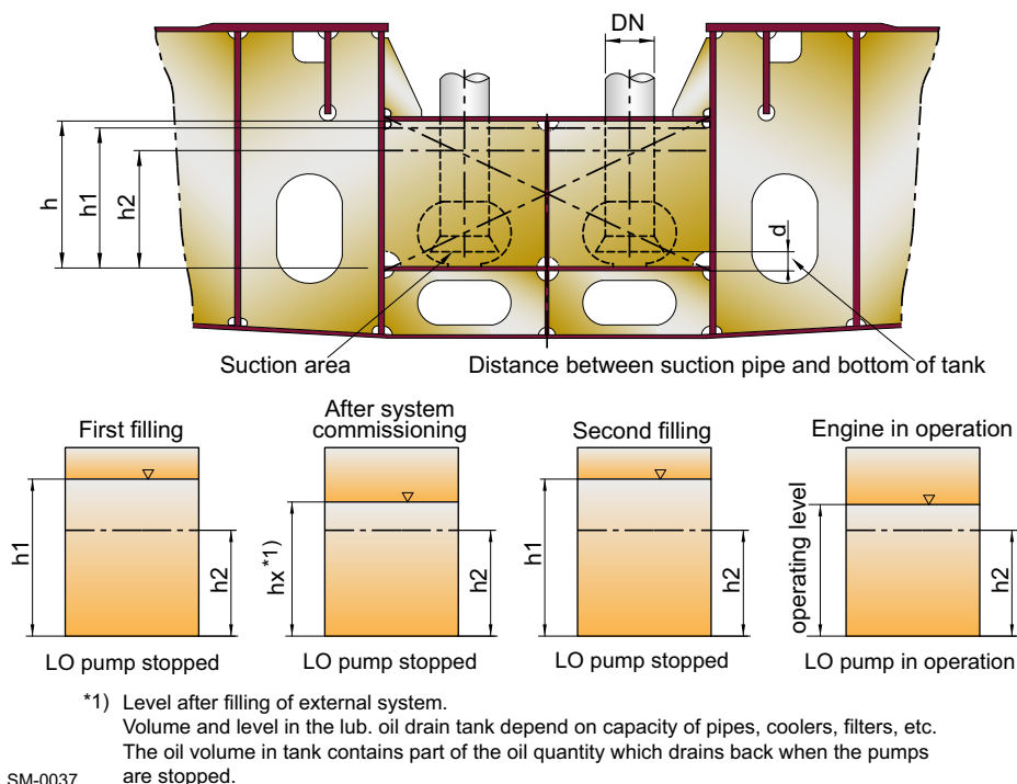
Figure 4-27 Dimensioning and filling process of LO drain tank
