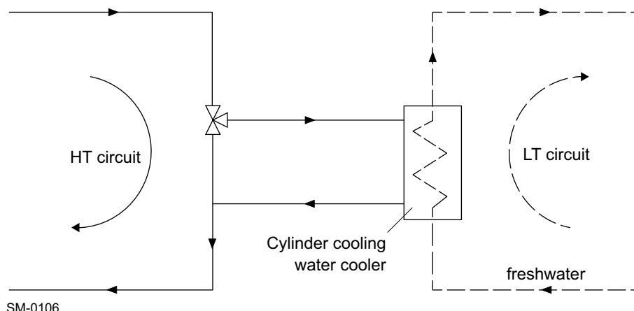
Figure 4-17 Separate HT cooling water circuit
