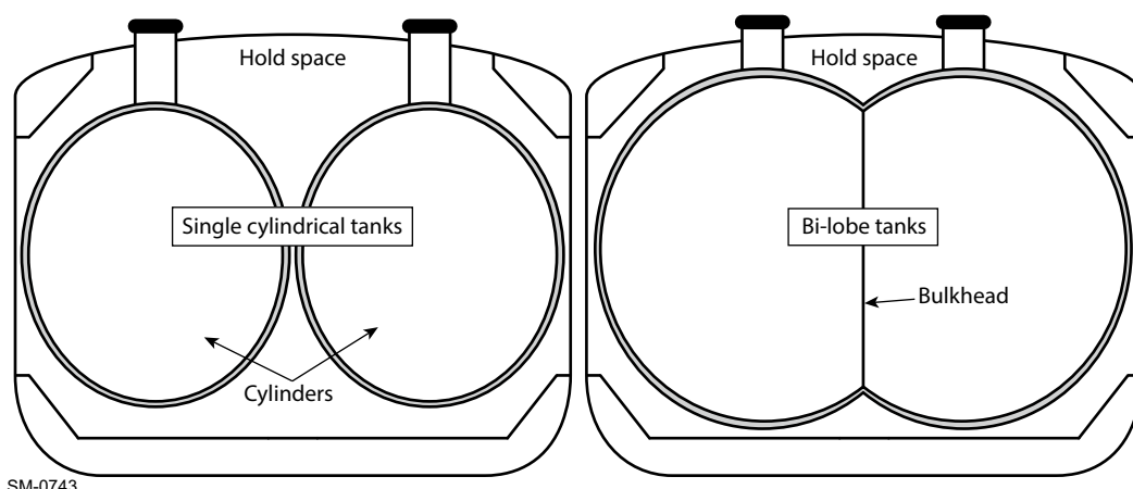
Figure 4-36 Section view of different free-standing Type C tanks installed below the deck
