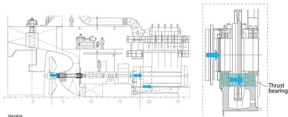
Figure 3-4 Force transmission to the engine foundation
