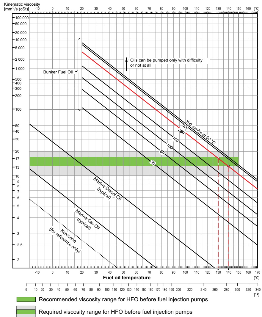
Figure 4-60 Fuel oil viscosity-temperature diagram
