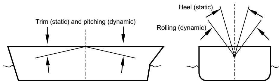
Figure 4-29 Inclination angles
