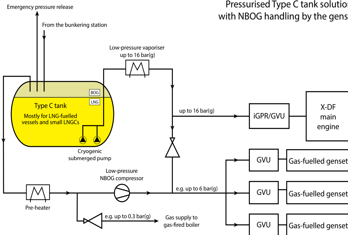
Figure 4-38 Pressurised Type C tank solution with NBOG handling by the gensets
