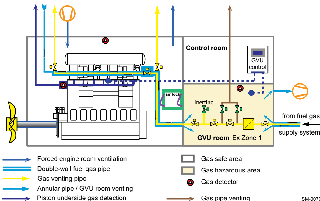
Figure 4-47 The GVU-OD™ from Wärtsilä
