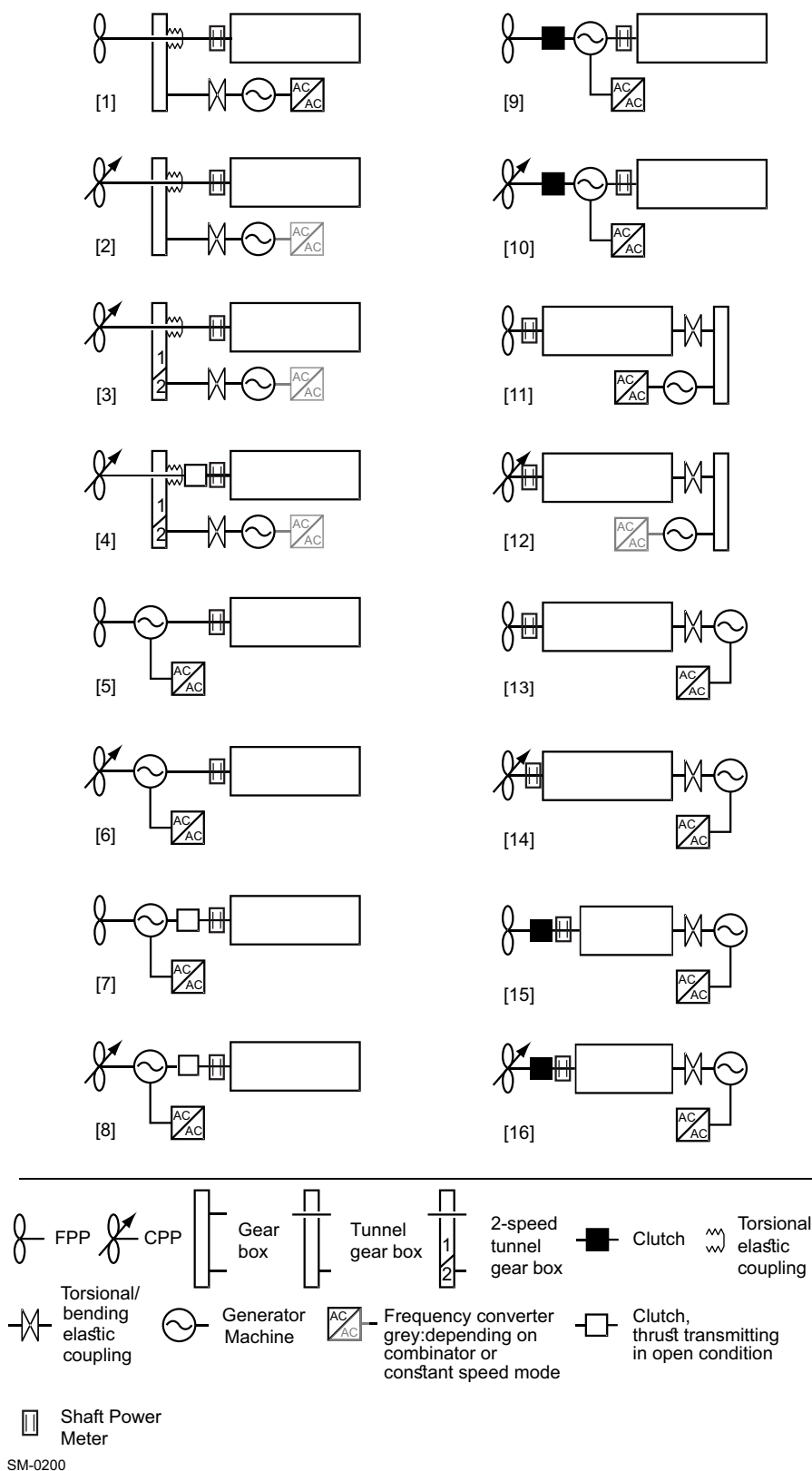
Figure 4-69 Arrangements for PTO, PTI, PTH
