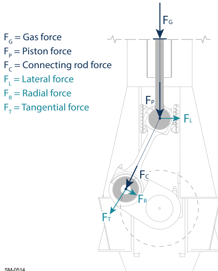
Figure 6-4 Forces through the engine
