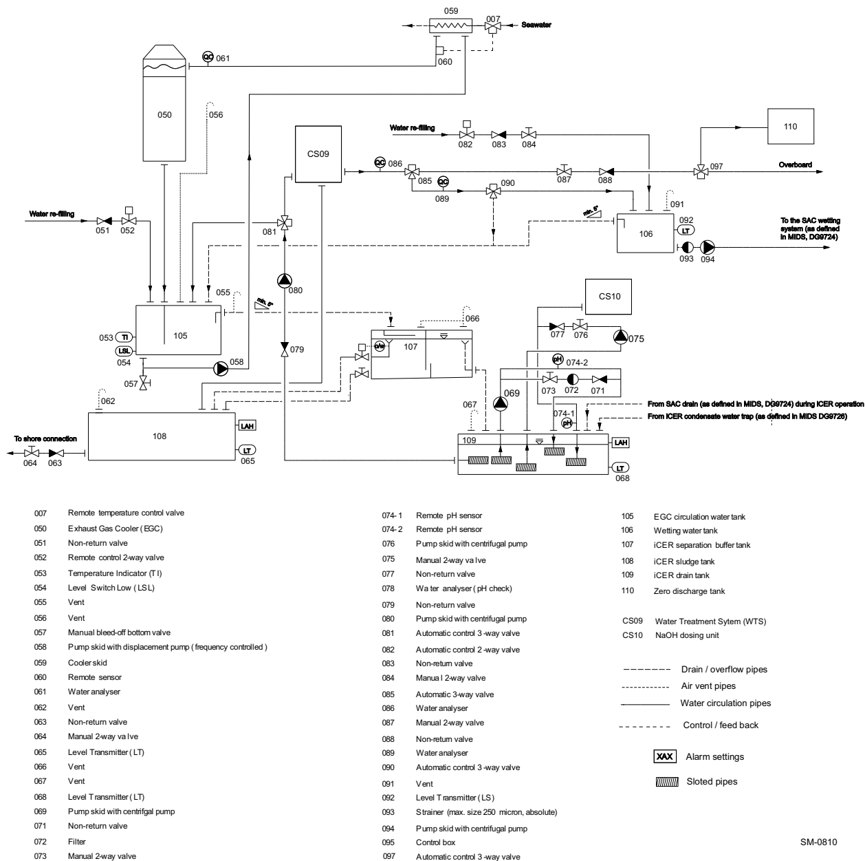
Figure 4-8 The iCER drainage system valid for all iCER operating mode options
