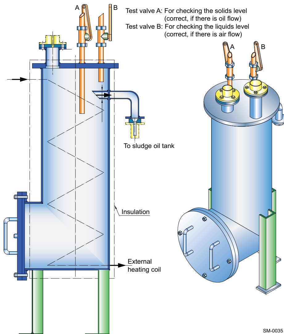
Figure 4-62 Design proposal of the WinGD sludge oil trap
