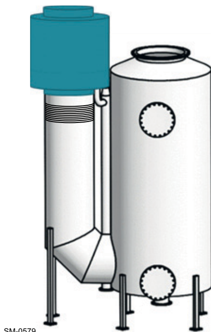
Figure 4-16 Arrangement of the additional economiser
