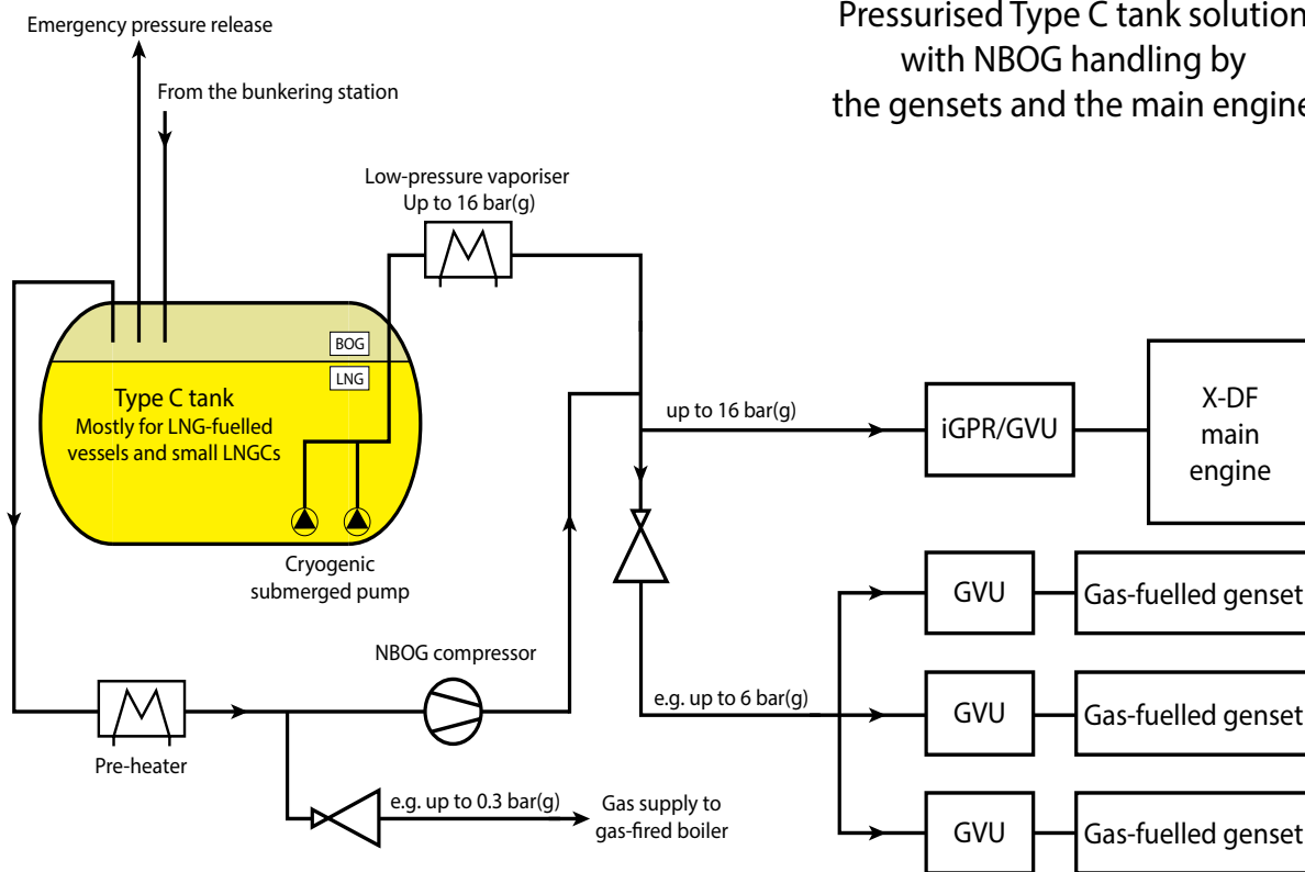
Figure 4-39 Pressurised Type C tank solution with NBOG handling by the gensets and the main engine
