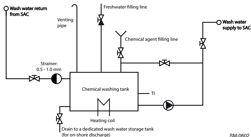
Figure 4-64 Offline SAC washing system (external system)
