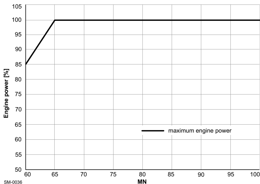
Figure 4-32 Maximum achievable power
