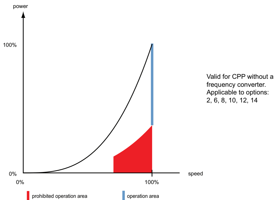
Figure 4-72 CPP in constant speed operation without frequency converter
