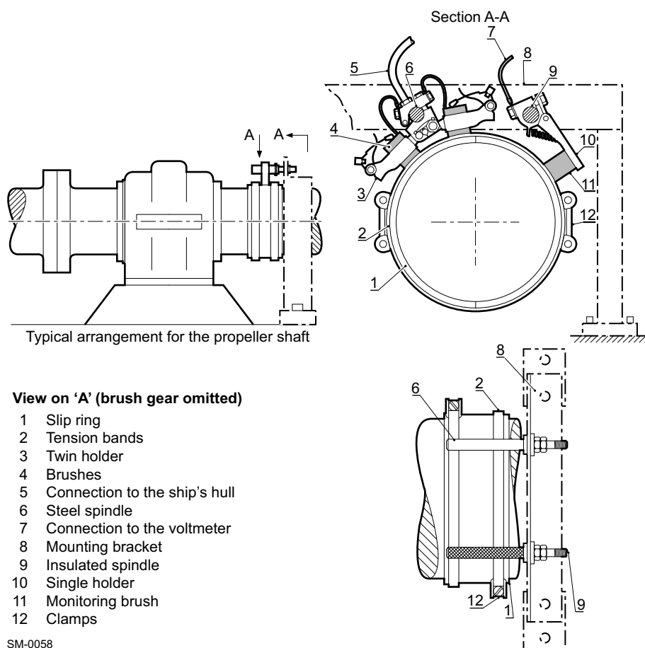
Figure 3-8 Typical shaft earthing arrangement
