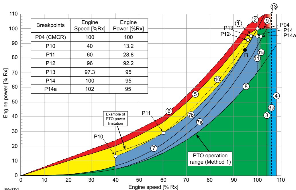
Figure 2-5 Power range limits for PTO operation: Method 1
