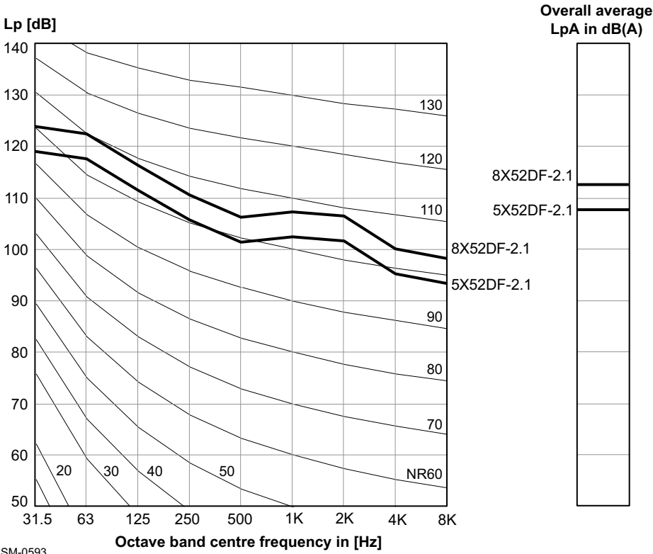
Figure 7-6 Sound pressure level at funnel top of exhaust gas system
