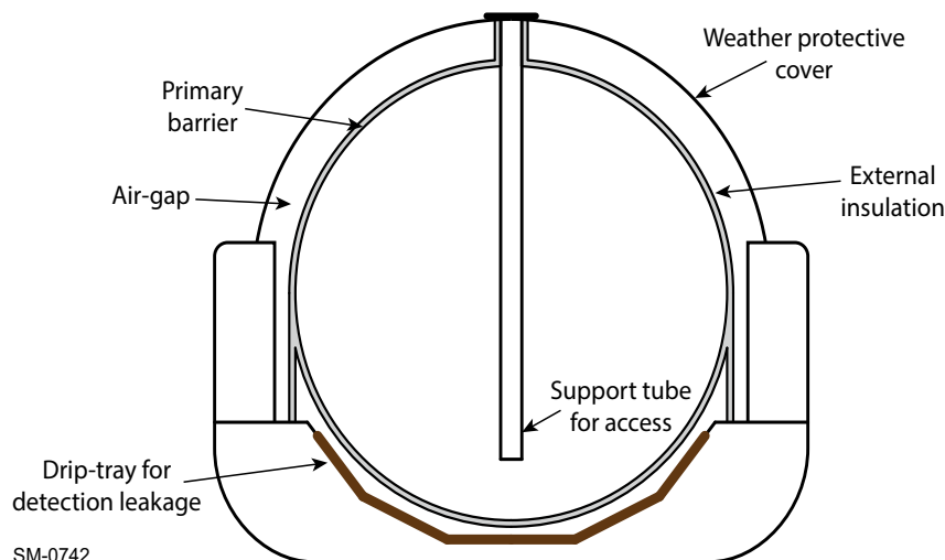
Figure 4-35 Section view of a free-standing Type B tank of moss design
