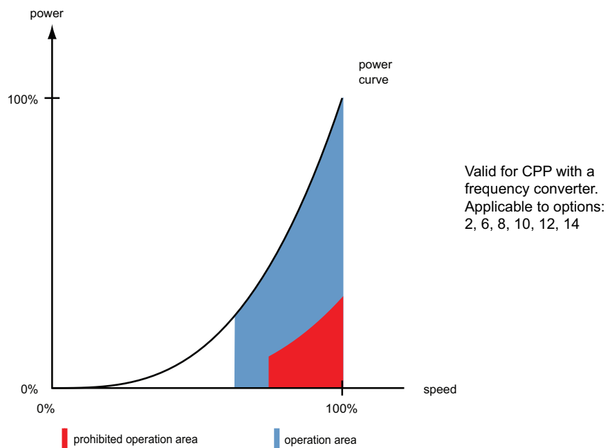
Figure 4-71 CPP in combination with an optional frequency converter
