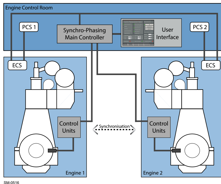
SM-0516 Figure 6-18 Synchro-Phasing System
