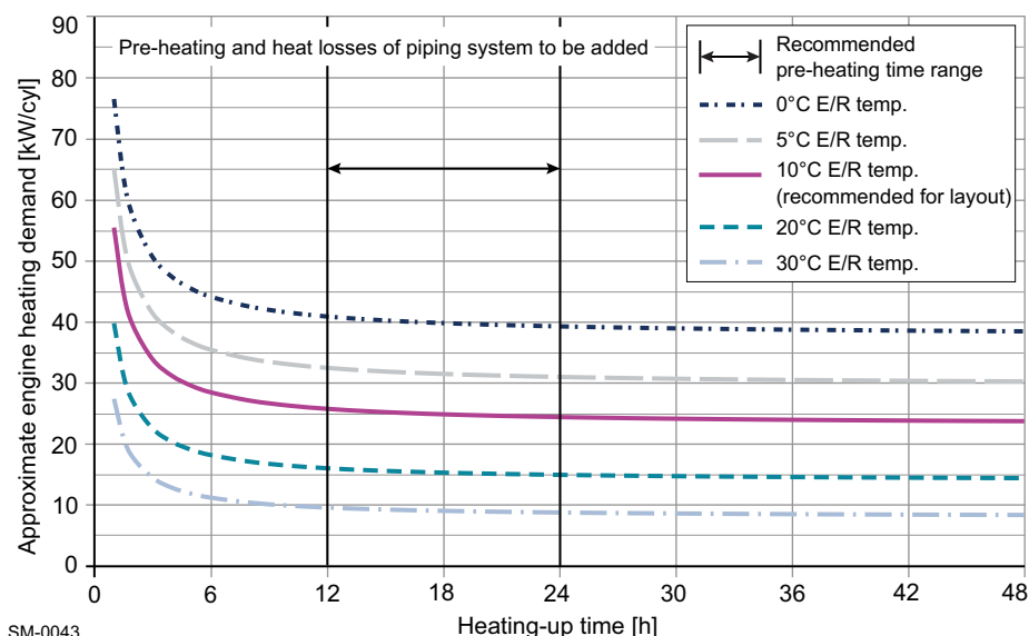
Figure 4-22 Pre-heating power requirement per cylinder
