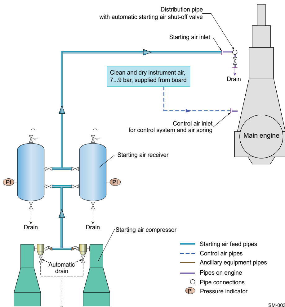
Figure 4-61 Air supply system
