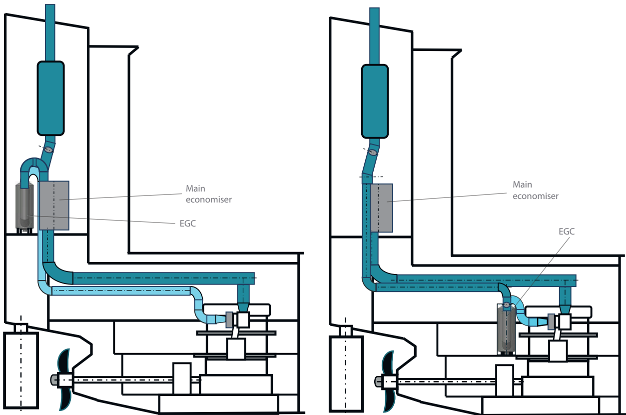
Figure 4-15 The long route arrangement
