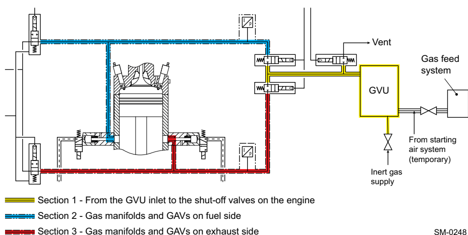
Figure 4-50 Gas leak test sequence (engines with GUV)
