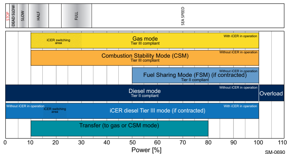
Figure 1-2 Operating modes (as per ISO conditions)
