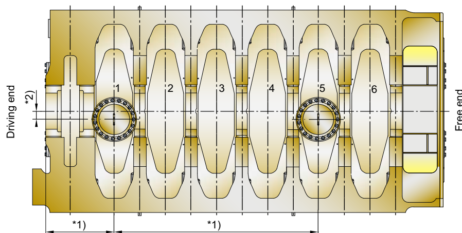
Figure 4-28 Arrangement of vertical LO drains for 6-cylinder engines
