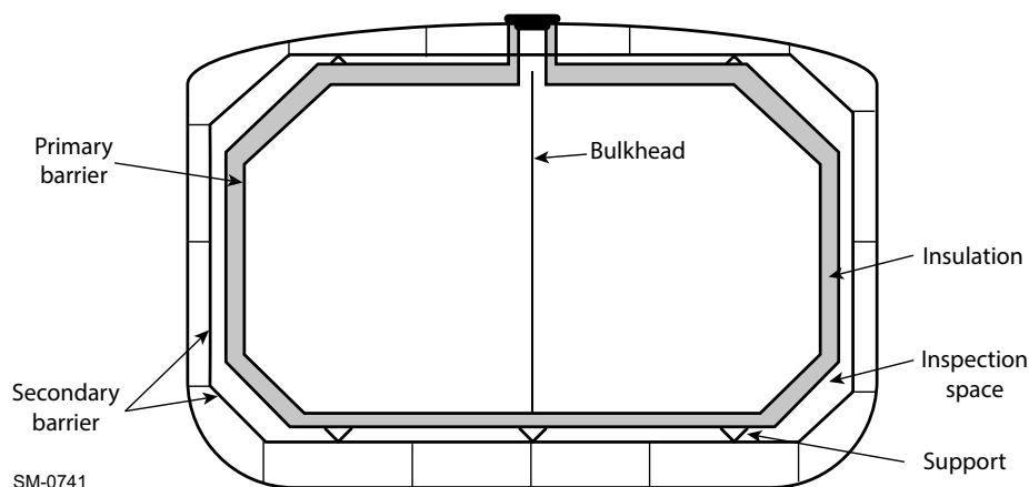
Figure 4-34 Section view of a free-standing Type A tank
