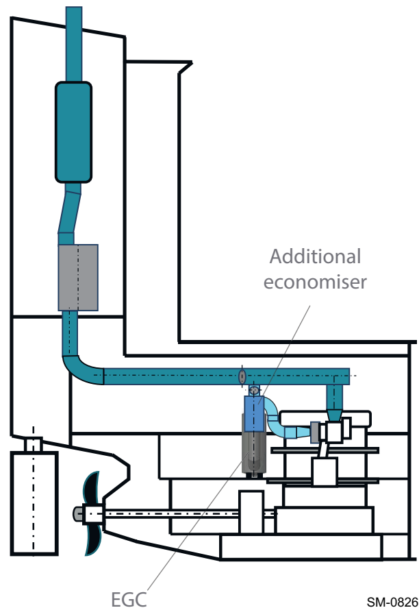
Figure 4-14 The short route arrangement
