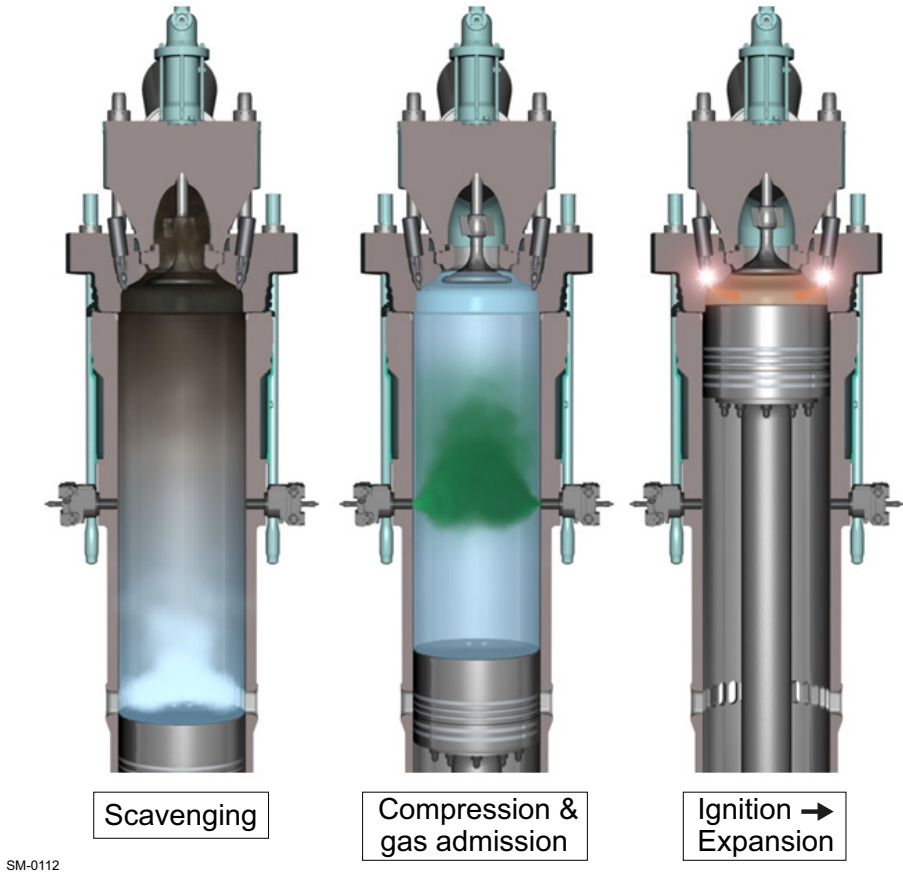
Figure 4-30 Lean burn with pilot ignition
