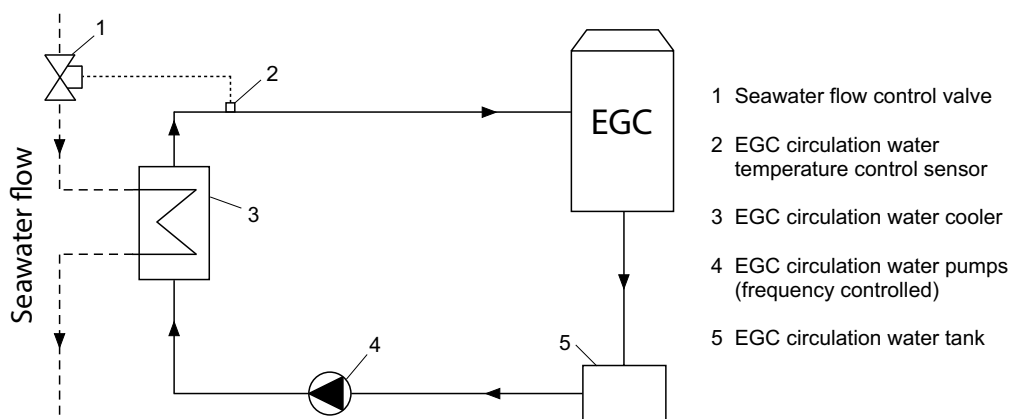
Figure 4-7 The EGC circulation water system (off-engine option)
