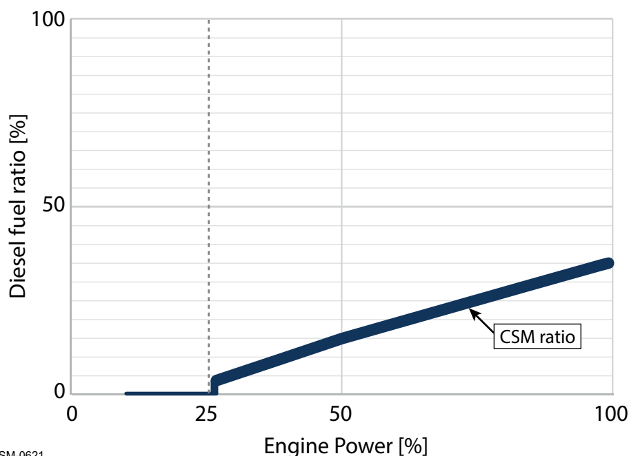
Figure 1-5 Example of diesel fuel ratio during active CSM
