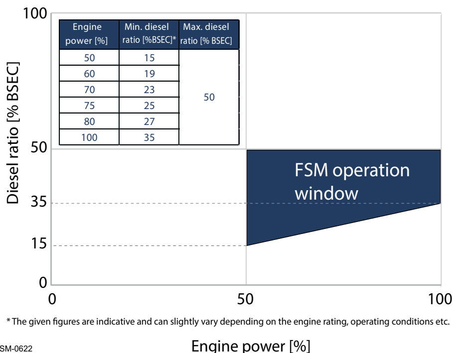
Figure 1-6 FSM: Available operating window
