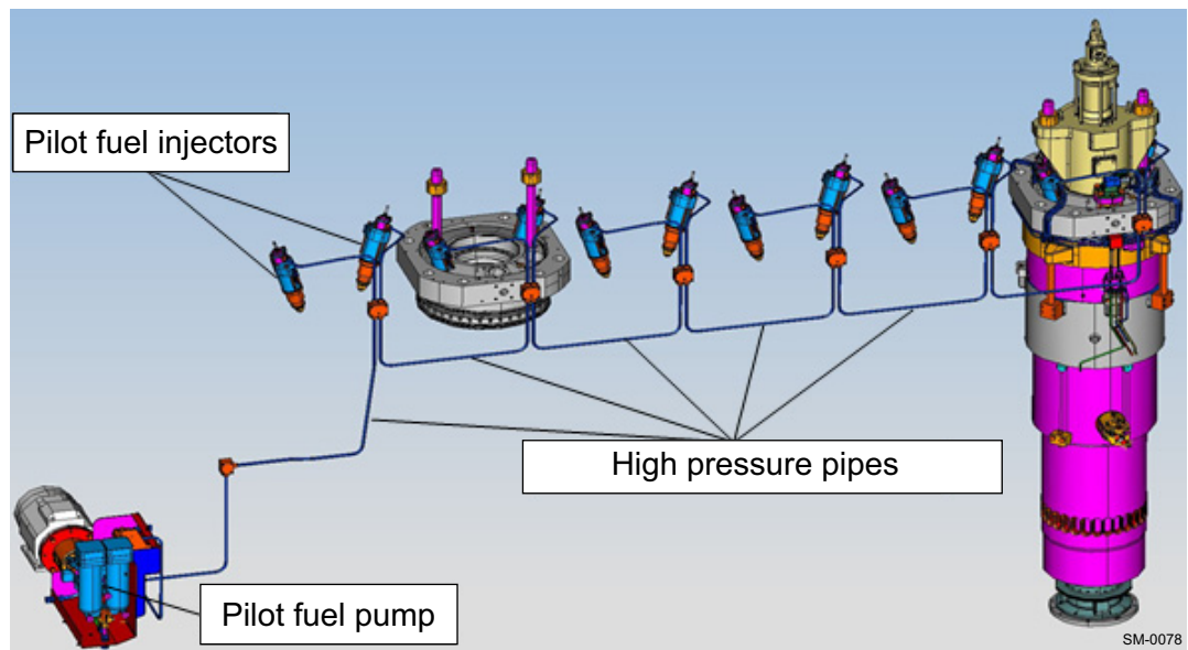
Figure 4-52 Pilot fuel high-pressure system
